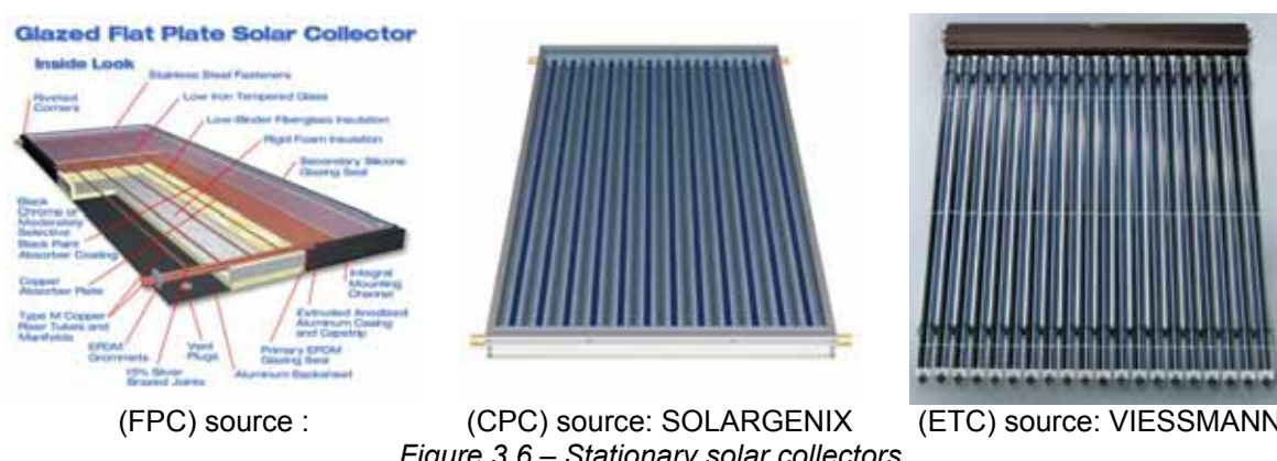
Figure 3.6 – Stationary solar collectors.
