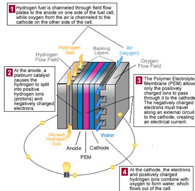
Figure 1.5 – Basic construction of a fuel cell-example Polymer Electrolyte fuel cell [ONO04].
