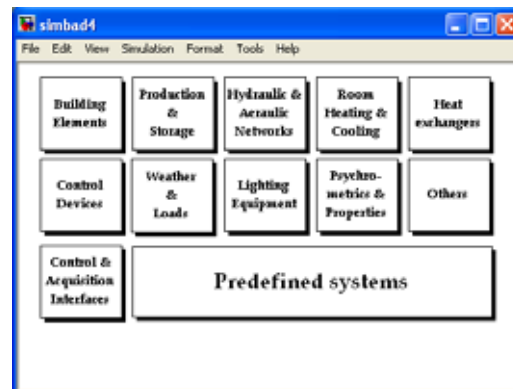
Figure 5.4 – SIMBAD library.
