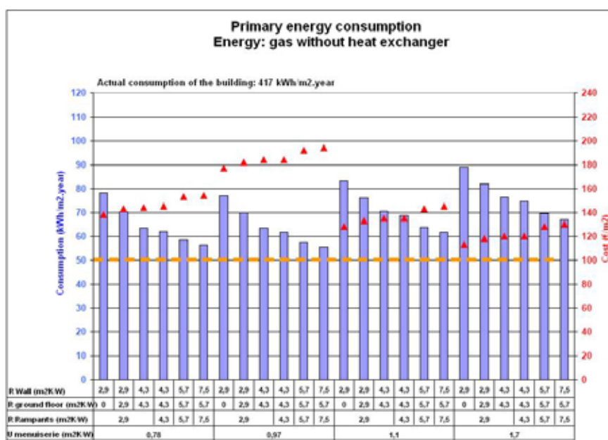
Figure 1.2 – Performance of refurbished buildings heated with gas and ventilated with a mechanical ventilation system without a heat recovery ventilation unit [SID07].
