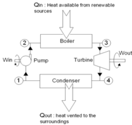
Figure 2.3 – Rankine cycle layout.
