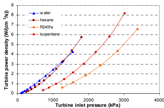
Figure 3.34 – Turbine power density, T_{cond} = 80^{\circ}\text{C} .
