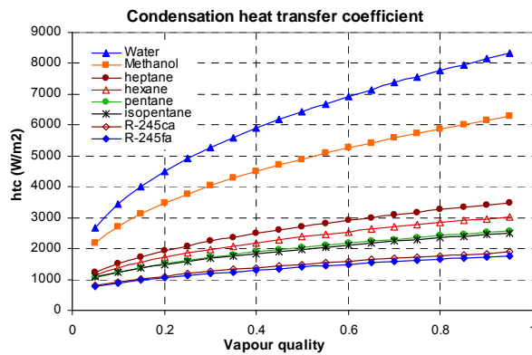
Figure 2.15 – Condensation heat transfer coefficient, T_{cond} = 80^{\circ}\text{C} , G_c = 30 \text{ kg/m}^2.\text{s} , D_h = 4.48 \text{ mm} .
