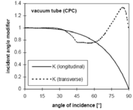
Figure 5.5 – Incidence angle modifier functions for the solar collector tested.
