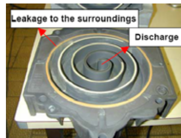
Figure 3.38 – Fixed scroll of the ATLAS COPCO oil free compressor.
