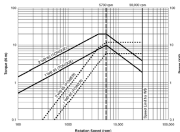
Figure 3.55 – WB torque–speed–power curves.
