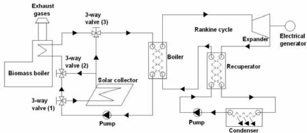
Figure 1.16 – Simplified flow sheet of the proposed SBORC-μCHP system.
