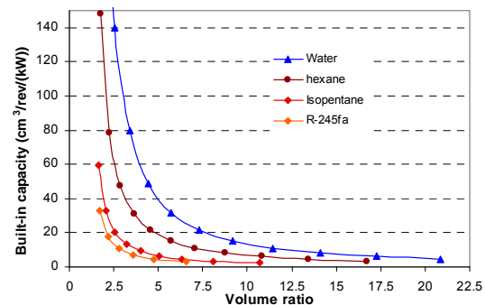
Figure 3.35 – Turbine built-in suction volume, T_{cond} = 80^{\circ}\text{C} .
