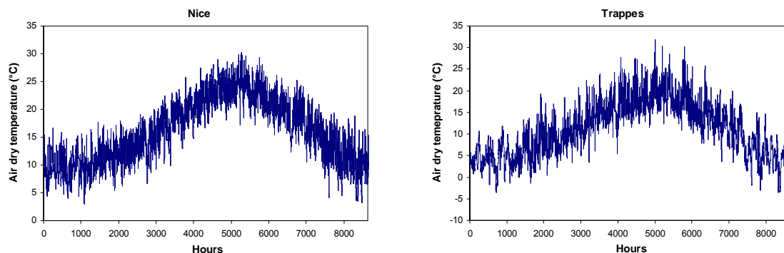
Figure 5.12 – RT2005 ambient temperature profiles.
