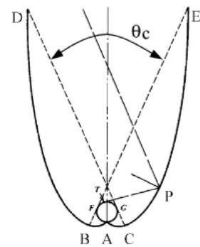
Figure 3.8 – Schematic diagram of a CPC.
