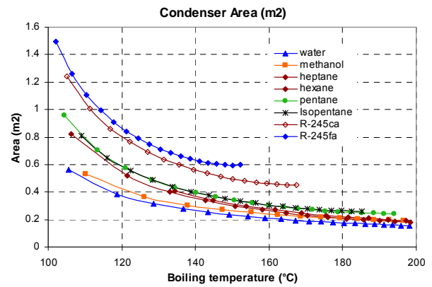
Figure 2.16 – Condenser area for different boiling temperature, T_{cond} = 80^{\circ}\text{C} , G_c = 30 \text{ kg/m}^2.\text{s} , D_h = 4.48 \text{ mm} .
