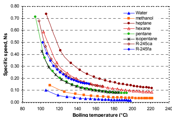
Figure 2.9 – Specific speed ( N = 3000 \text{ rpm} , W_{is} = 10 \text{ kW} )
