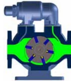
Figure 3.19 – Vane pump layout [VIKINGPUMP].
