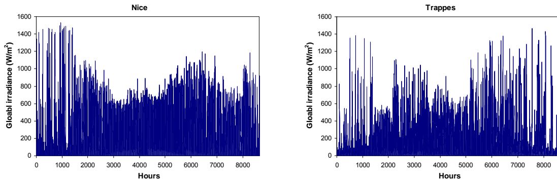
Figure 5.13 – Standard RT2005 global radiation data.
