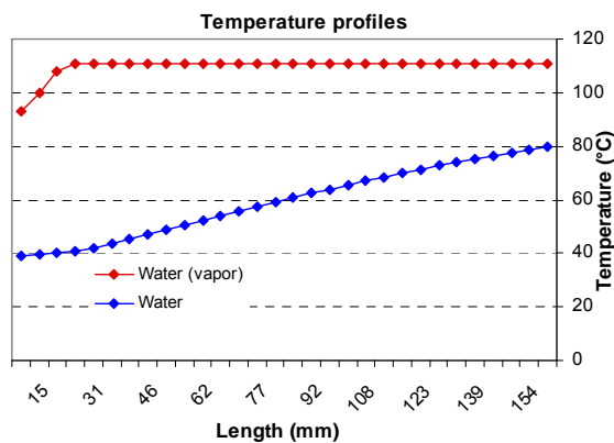
Figure 3.51 – Temperature profiles.
