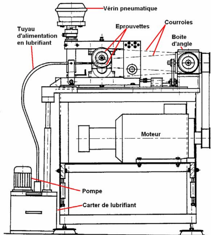
FIG. 2.3 – Machine bi-disques
