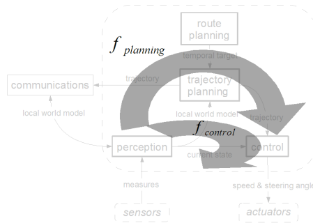
Figure 5.4: Main two logic parallel execution loops
