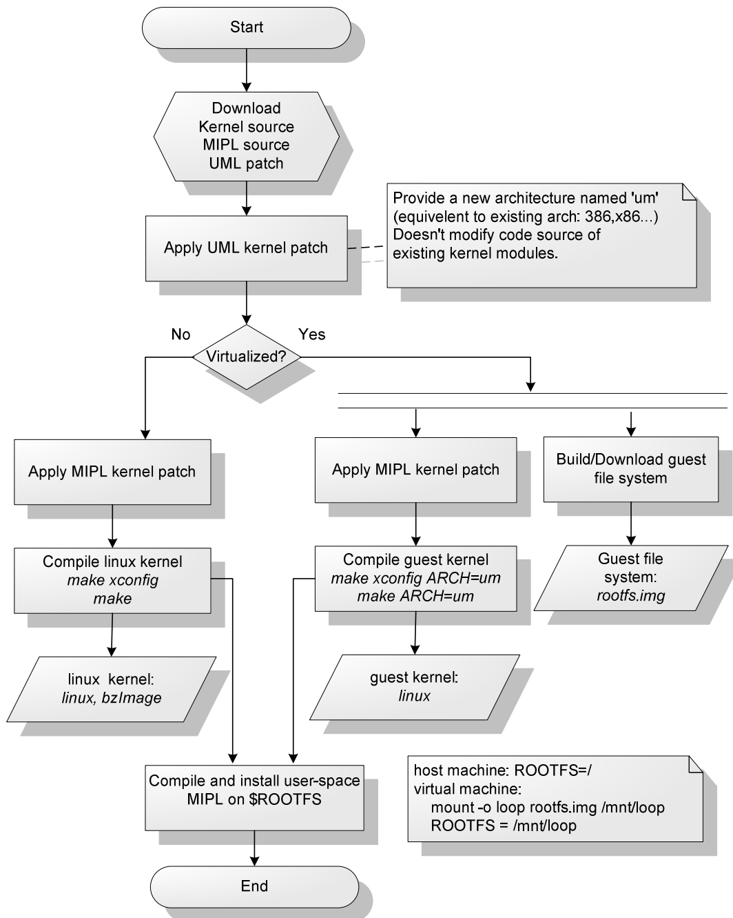
Figure 39. Unified Development Process for Mobile IP in UML/real testbed
