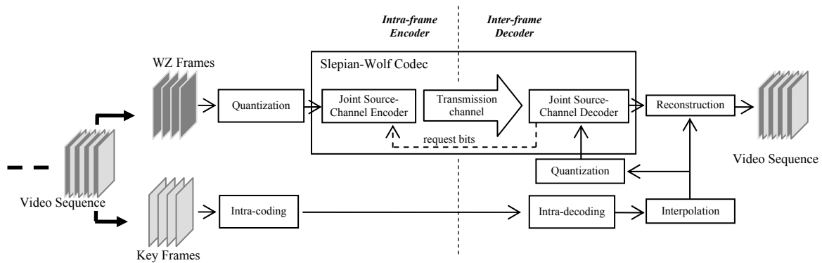
Figure 4.1 Block-diagram of the pixel-domain distributed video codec
