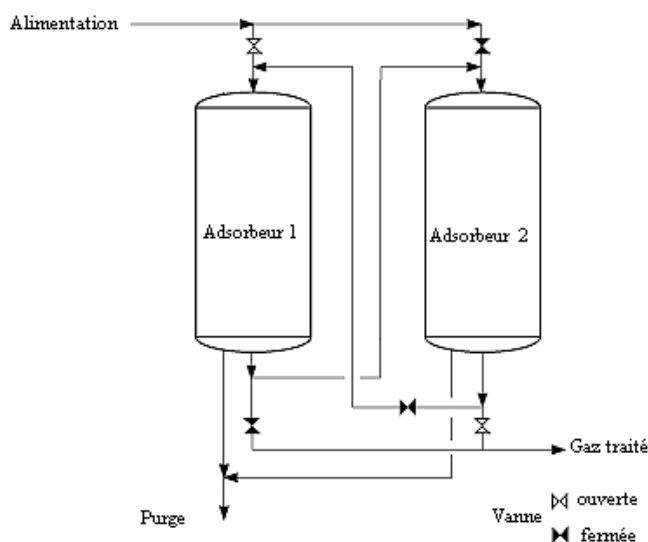
Figure 16 : Procédé PSA Pressure Swing Adsorption
