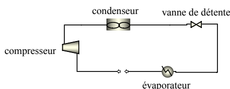
Figure 39 : Machine frigorifique.
