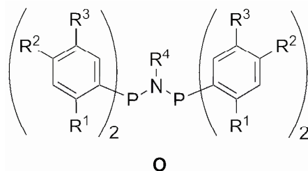
Figure 2. Bis(diarylphosphino)amine ligands O .
