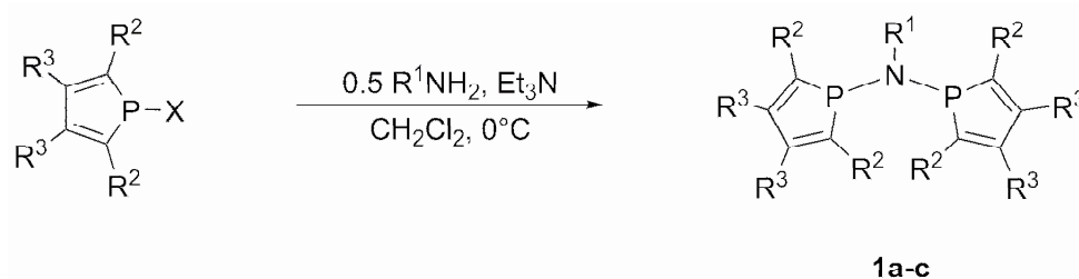
Scheme 1. Synthesis of bis(phosphole)amines 1a-c . X = Cl, Br.
