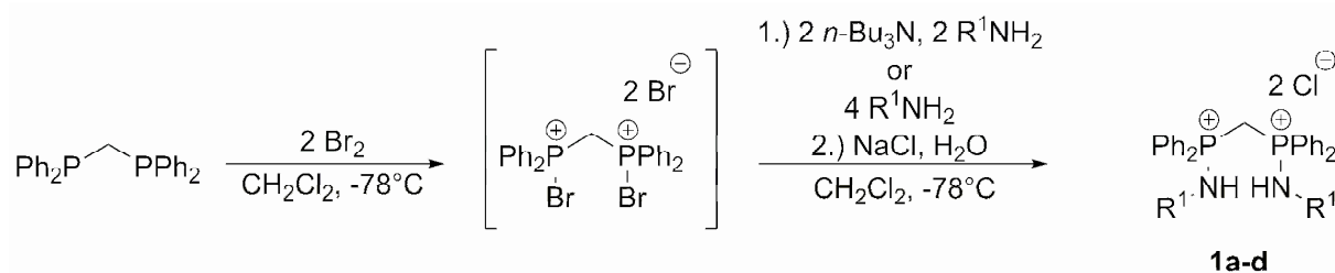
Scheme 2. Synthesis of bis(aminophosphonium) chlorides 1a-d by the Kirsanov method. a: R^1 = i\text{-Pr} , b: R^1 = t\text{-Bu} , c: R^1 = \text{Ph} , d: R^1 = o\text{-MeO-C}_6\text{H}_4 .
