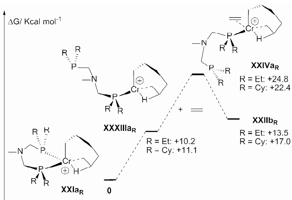
Scheme 31. Overall energetic pathway showing the possible formation of XXIIb R ( R = \text{Et}, \text{Cy} ) ethylene complexes from the pentacoordinated XXIa R chromacycloheptanes.
