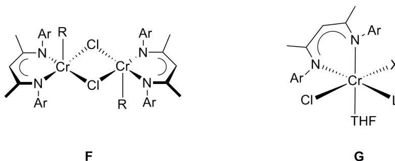
Figure 3. Cr(III)-β-ketiminate complexes. F : R = Me, Ar = Ph, 2,6- i -Pr-C 6 H 3 , G1 : Ar = 2,6- i -Pr-C 6 H 3 , X∩L = PhCOO, G2 : Ar = Ph, X = Cl, L = THF.
