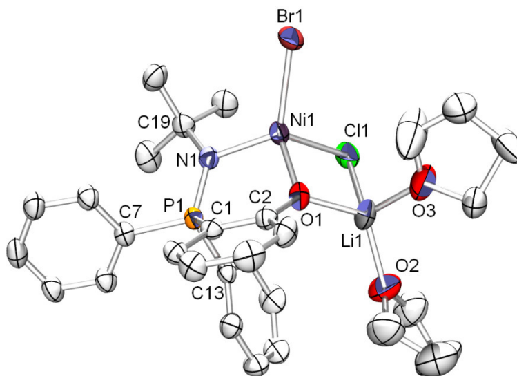
Figure 8. Ortep representation of the x-ray crystal structure of 10b . Partial chloride bromide exchange has been observed on this structure and the Br/Cl occupation factors refine to a value close to 0.8/0.2. Hydrogen atoms have been omitted for clarity. Thermal ellipsoids are represented at the 50% level. Important bond lengths (Å) and angles (°): P1-N1 = 1.601(2), P1-C1 = 1.802(3), N1-C19 = 1.506(3), C2-O1 = 1.323(3), O1-Ni1 = 1.954(2), Ni1-N1 = 1.981(2), Ni1-Br1 = 2.382(2), Ni1-Cl1 = 2.32(1), Cl1-Li1 = 2.32(1), Li1-O1 = 1.894(5), Li1-O2 = 1.871(6), Li1-O3 = 1.930(7), O1-Ni1-N1 = 98.7(1), O1-Ni1-Br1 = 119.19(7), P1-N1-C19 = 129.4(2), P1-N1-Ni1 = 113.4(1), O1-Ni1-Cl1 = 88.6(3), O1-Li1-Cl1 = 90.1(3), O2-Li1-O3 = 106.4(3).
