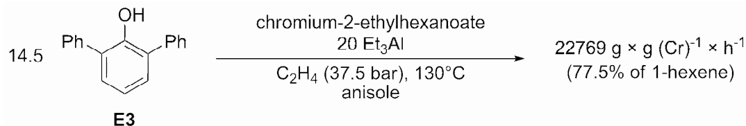
Scheme 7.
