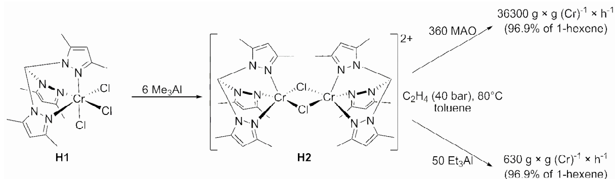
Scheme 12. The two chloro-methyl-aluminate counteranions of H2 have been omitted for clarity reasons. They do not participate in the coordination to the chromium centers.
