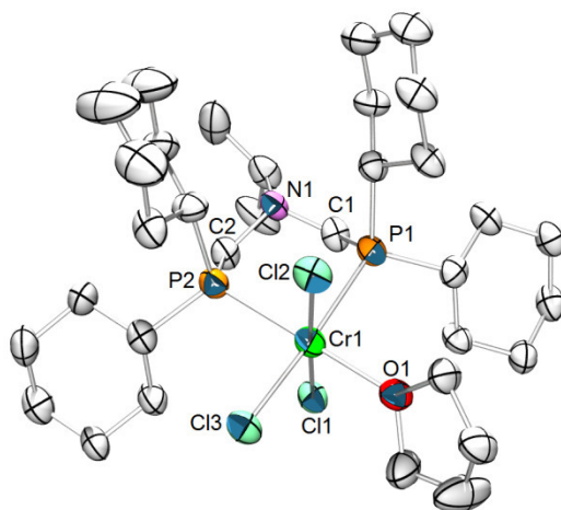
Figure 8. Molecular structure of one molecule of 4d in the crystal. Thermal ellipsoids are drawn at the 30% probability level. Hydrogen atoms are omitted for clarity. Selected bond distances (Å) and angles (°): P1-Cr1 = 2.518(2), P1-Cl1 = 1.836(5), C1-N1 = 1.457(6), N1-C2 = 1.465(7), C2-P2 = 1.863(5), P2-Cr1 = 2.466(2), Cr1-Cl1 = 2.320(2), Cr1-Cl2 = 2.314(2), Cr1-Cl3 = 2.311(2), Cr1-O1 = 2.104(3), P1-C1-N1 = 116.3(4), C1-N1-C2 = 112.8(4), N1-C2-P2 = 116.1(4), C2-P2-Cr1 = 113.6(2), P2-Cr1-P1 = 85.90(5), P2-Cr1-Cl1 = 86.94(6), P2-Cr1-Cl3 = 90.16(6), P2-Cr1-Cl2 = 92.82(6), P2-Cr1-O1 = 177.4(1), P1-Cr1-Cl1 = 85.53(6), P1-Cr1-Cl2 = 89.72(6), Cl3-Cr1-Cl1 = 91.44(6).
