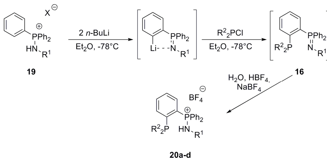
Scheme 11. Access to phosphine-iminophosphoranes 16 and phosphine-aminophosphonium tetrafluoroborates 20a-d as described by Boubekeur et al. X = Cl, Br, a : \text{R}^1 = \text{CH}_2\text{-}t\text{-Bu} , \text{R}^2 = \text{Ph} , b : \text{R}^1 = i\text{-Pr} , \text{R}^2 = \text{Ph} , c : \text{R}^1 = t\text{-Bu} , \text{R}^2 = \text{Ph} d : \text{R}^1 = t\text{-Bu} , \text{R}^2 = i\text{-Pr} .
