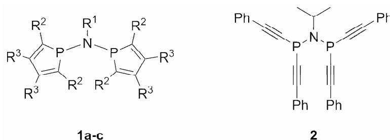
Figure 1. Evaluated PNP ligands. 1a : R 1 = R 2 = Ph, R 3 = H, b : R 1 = i -Pr, R 2 = Ph, R 3 = H, c : R 1 = Ph, R 2 = SiMe 3 , R 3 = Me.
