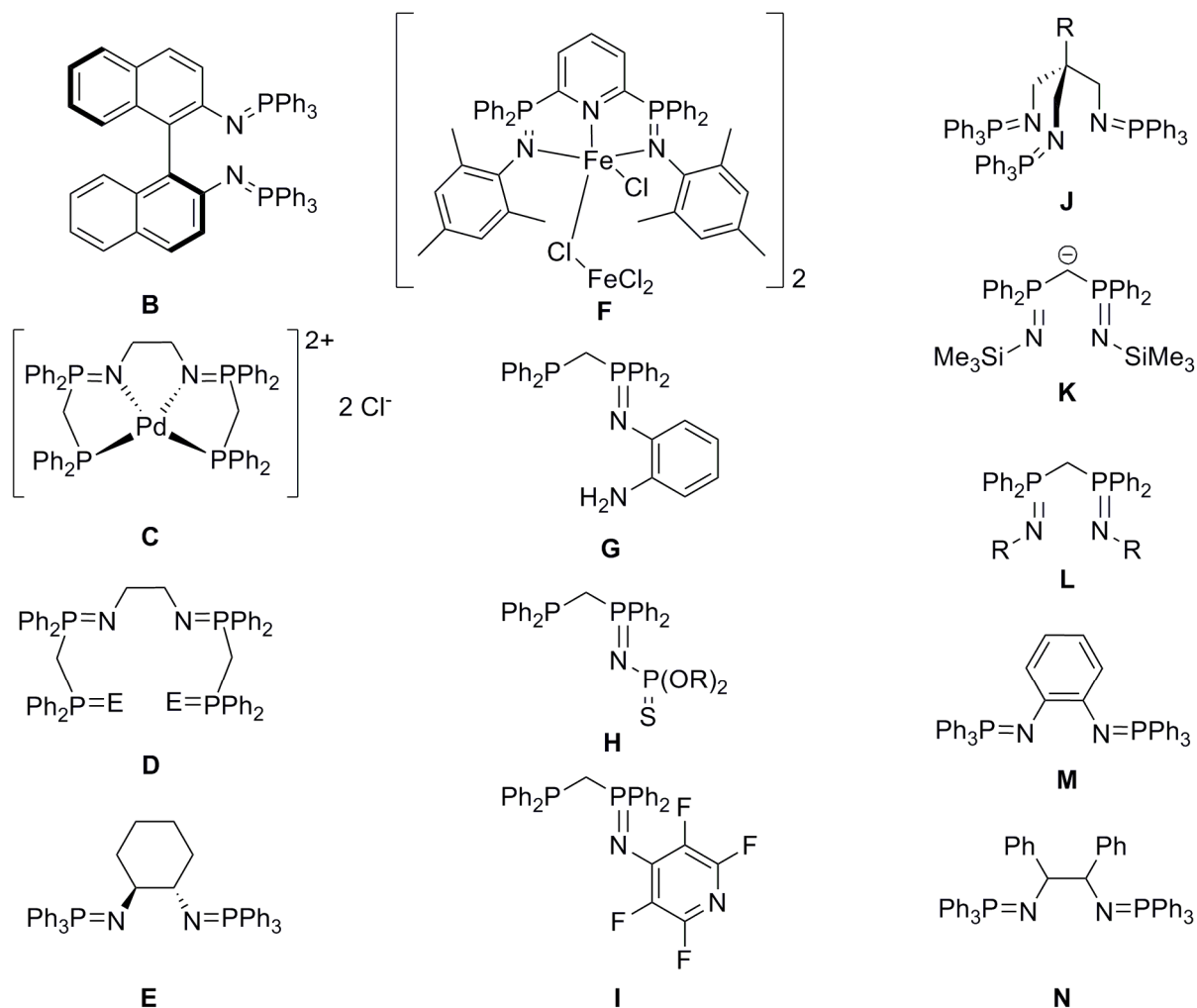
Figure 2. Some iminophosphorane ligands and complexes which have found applications in homogeneous catalysis processes. D ( \text{E} = \text{O}, \text{S}, \text{lone pair} ).
