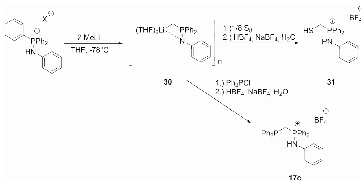
Scheme 16. Lithiation of [\text{Ph}_3\text{P}-\text{N}(\text{H})\text{Ph}]^+\text{X}^- ( \text{X} = \text{Cl}, \text{Br} ) with MeLi and subsequent quenching reactions.
