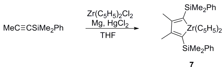
Scheme 5. Synthesis of the zirconacyclopentadiene 7 .
