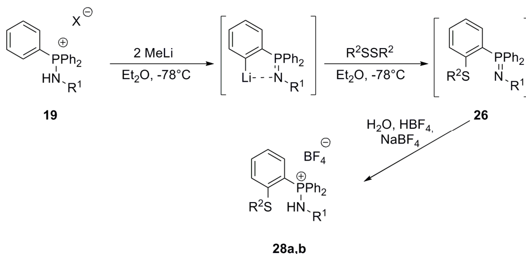
Scheme 14. Access to thioether-iminophosphoranes 26 and thioether-aminophosphonium tetrafluoroborates 28a,b . X = Cl, Br, a : R^1 = t\text{-Bu} , R^2 = \text{Ph} , b : R^1 = t\text{-Bu} , R^2 = n\text{-Bu} .
