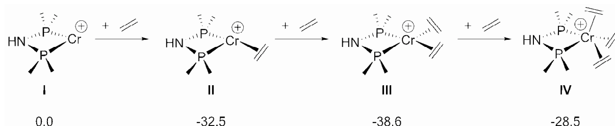
Scheme 11. Relative Stability of various [(\text{PNP})\text{Cr}(\text{ethylene})_n]^+ species. Gibbs free energies are given in \text{Kcal} \times \text{mol}^{-1} .
