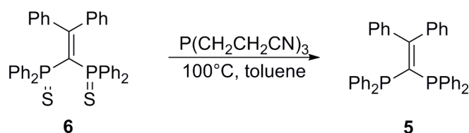
Scheme 4. Synthesis of the diphosphine 5 .
