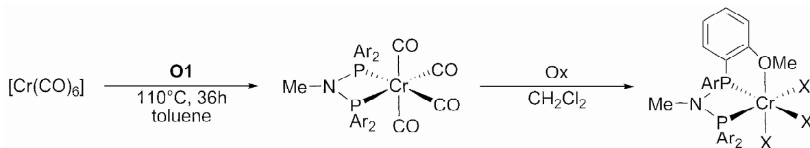
Scheme 20. Ar = o -MeO-C 6 H 4 , Ox = Br 2 , thus X = Br, and Ox = I 2 , thus X = I.
