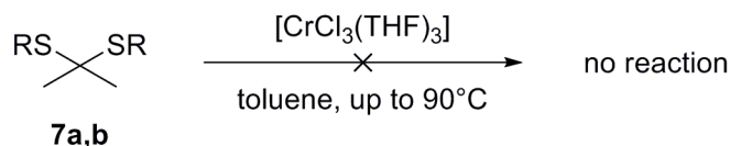
Scheme 6. Coordination attempts with dithioacetals 7a,b .
