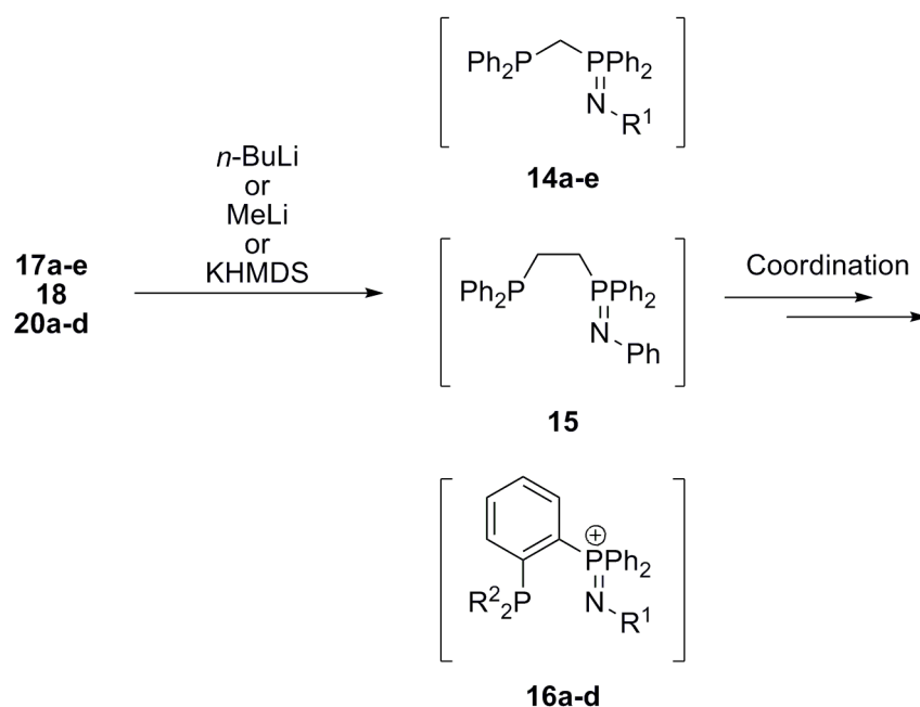
Scheme 12. Deprotonation-coordination sequence.
