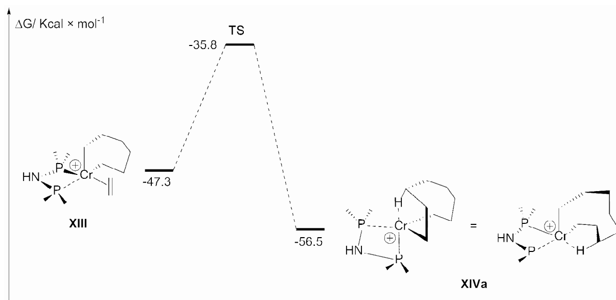
Scheme 18. Chromacyclononane formation.
