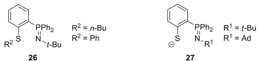
Figure 17. Neutral thioether-iminophosphorane ( 26 ) and anionic thiophenolato-iminophosphorane ( 27 ) ligands.
