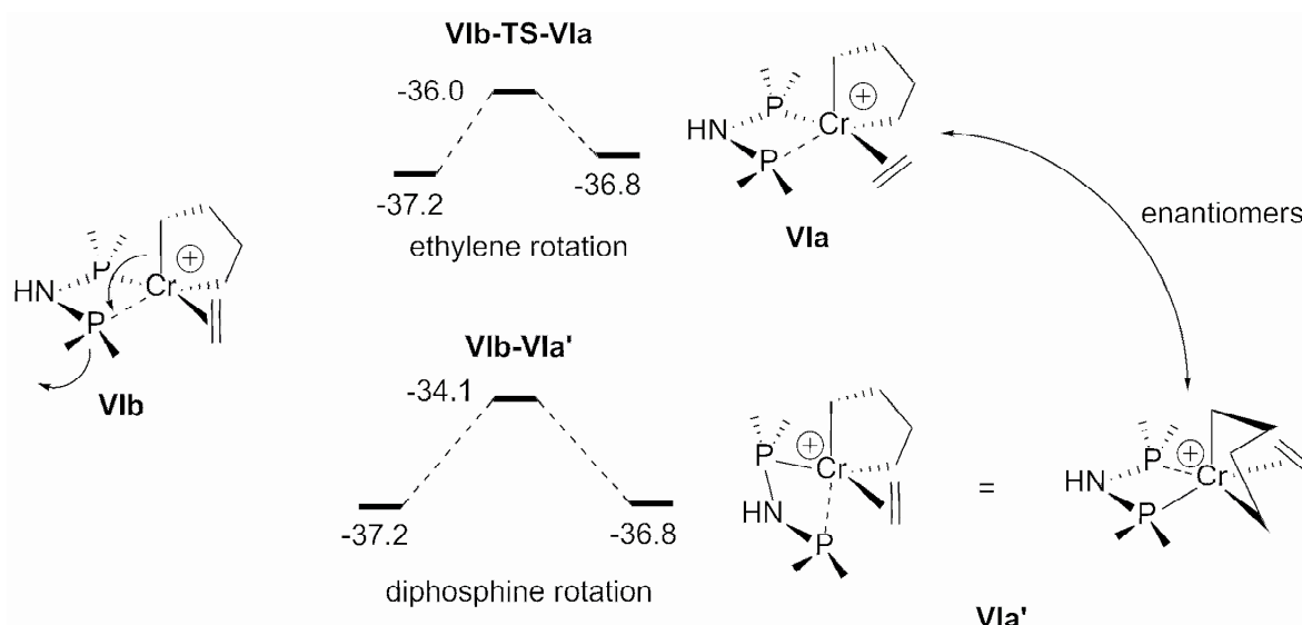
Scheme 13. VIb \leftrightarrow VIa ( VIa' ) interconversion via either ethylene or diphosphine rotation.
