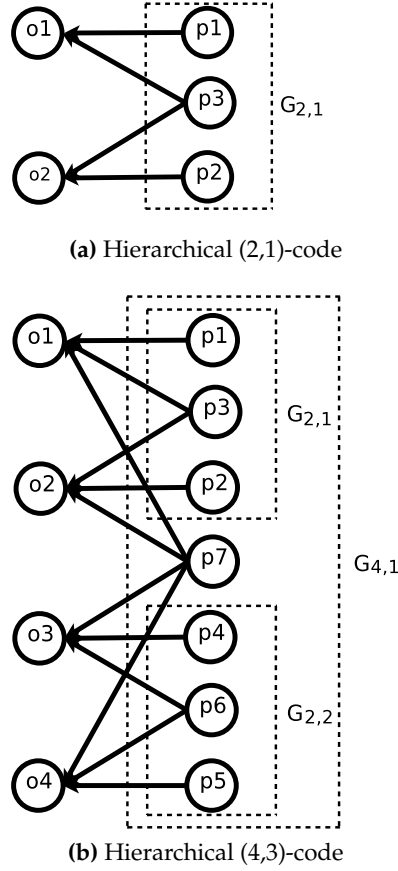
Figure 5.4: Samples of Code Graphs for Hierarchical Codes.
