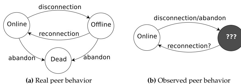
Figure 1.3: State machine modeling the behavior of a peer.
