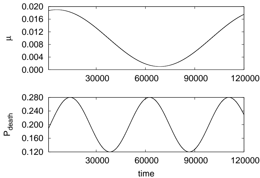
Figure 6.6: Simulation with varying parameters and an ideal estimator. Evolution of the input parameters \mu and P_{death} .
