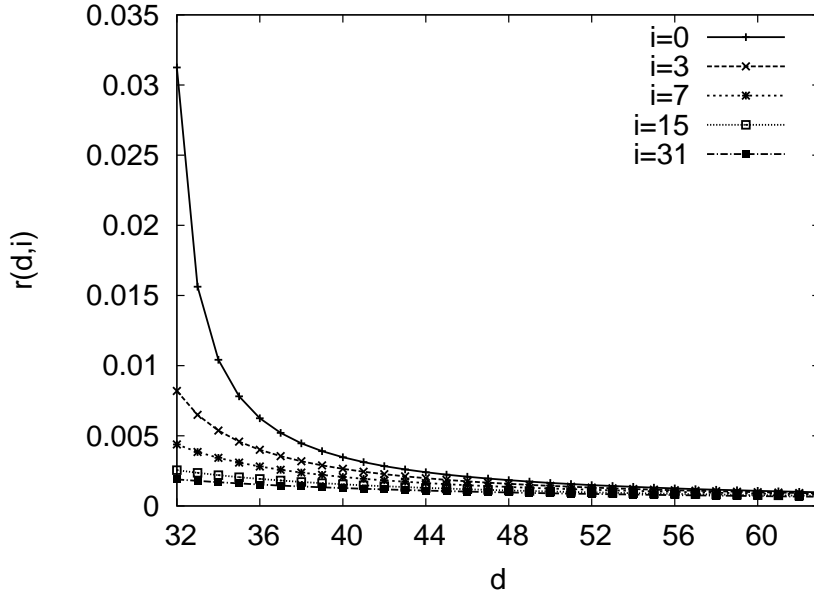
Figure 4.2: Function r(d,i) , which determines the amount of data that needs to be transferred upon a repair, for a Regenerating Code with k=32 and h=32 .
