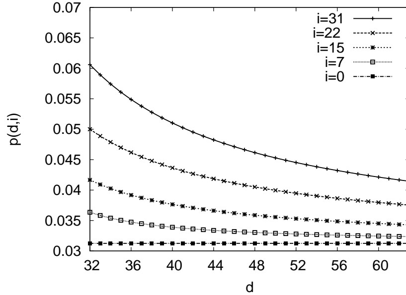
Figure 4.1: Function p(d, i) , which determines the block size, for a Regenerating Code with k=32 and h=32 .
