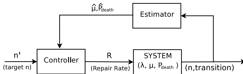
Figure 6.1: The adaptive control scheme.
