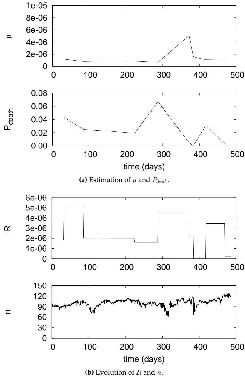
Figure 6.14: Adaptive Hybrid Scheme: Simulation with PlanetLab traces for D = 500 .
