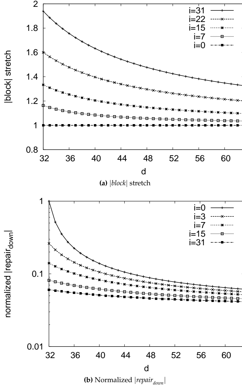
Figure 4.3: Size of the parity blocks and repair communication cost (in log-scale) normalized by the reference values of a traditional erasure code, for RC(32, 32, d, i) .
