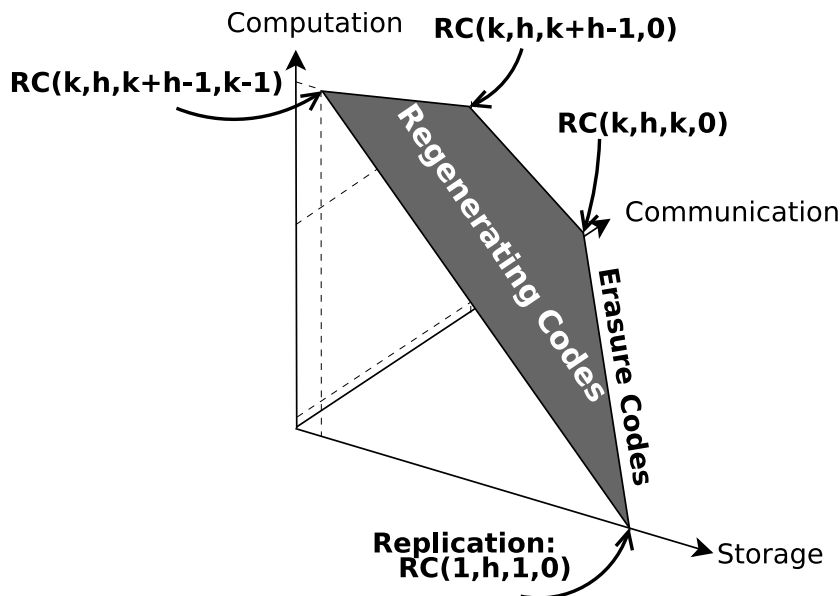
Figure 4.9: Illustration of the trade-offs provided by Regenerating Codes.
