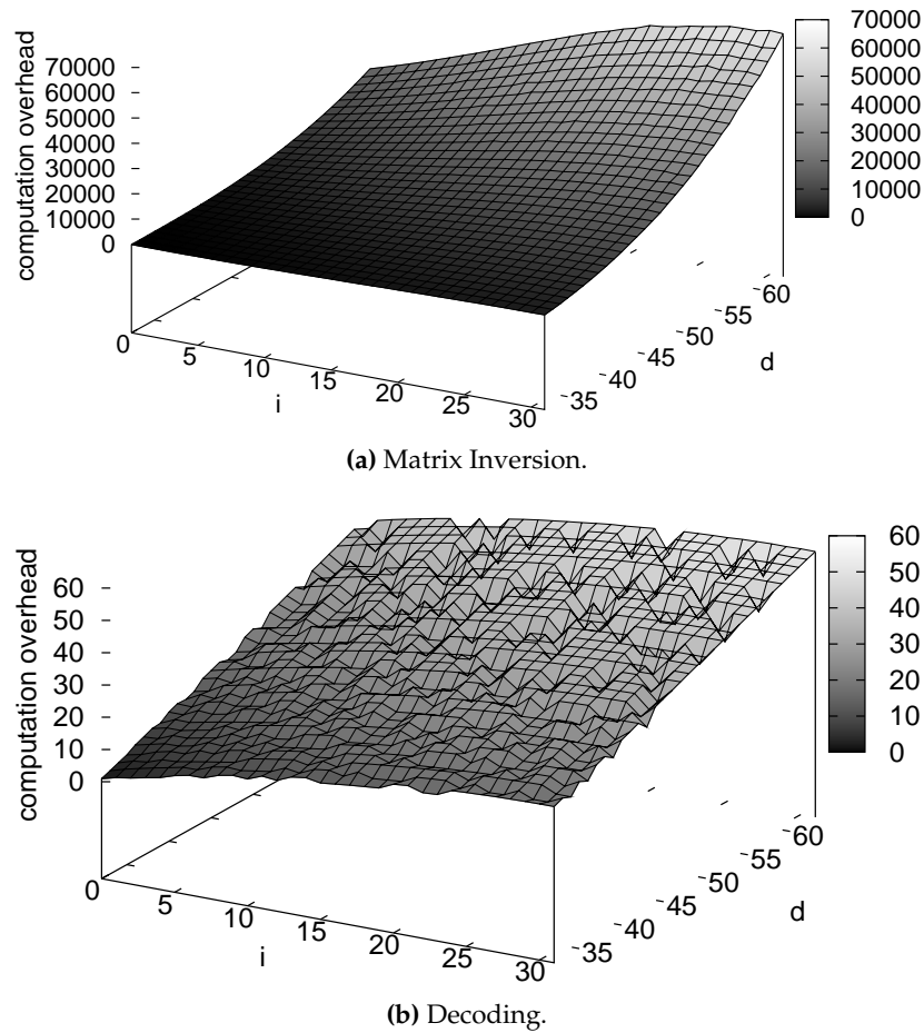
Figure 4.8: Reconstruction computation overhead for RC(32, 32, d, i) .
