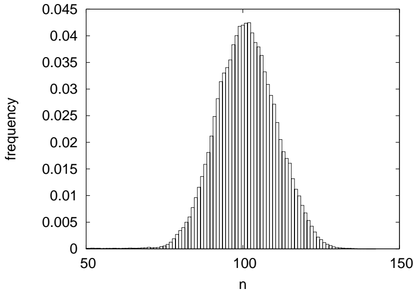
Figure 6.8: Simulation with varying parameters and an ideal estimator. Distribution of the number of available parity blocks.
