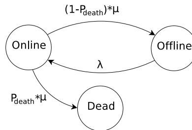
Figure 6.2: The Continuous-Time Semi-Markov chain of a peer life-cycle.
