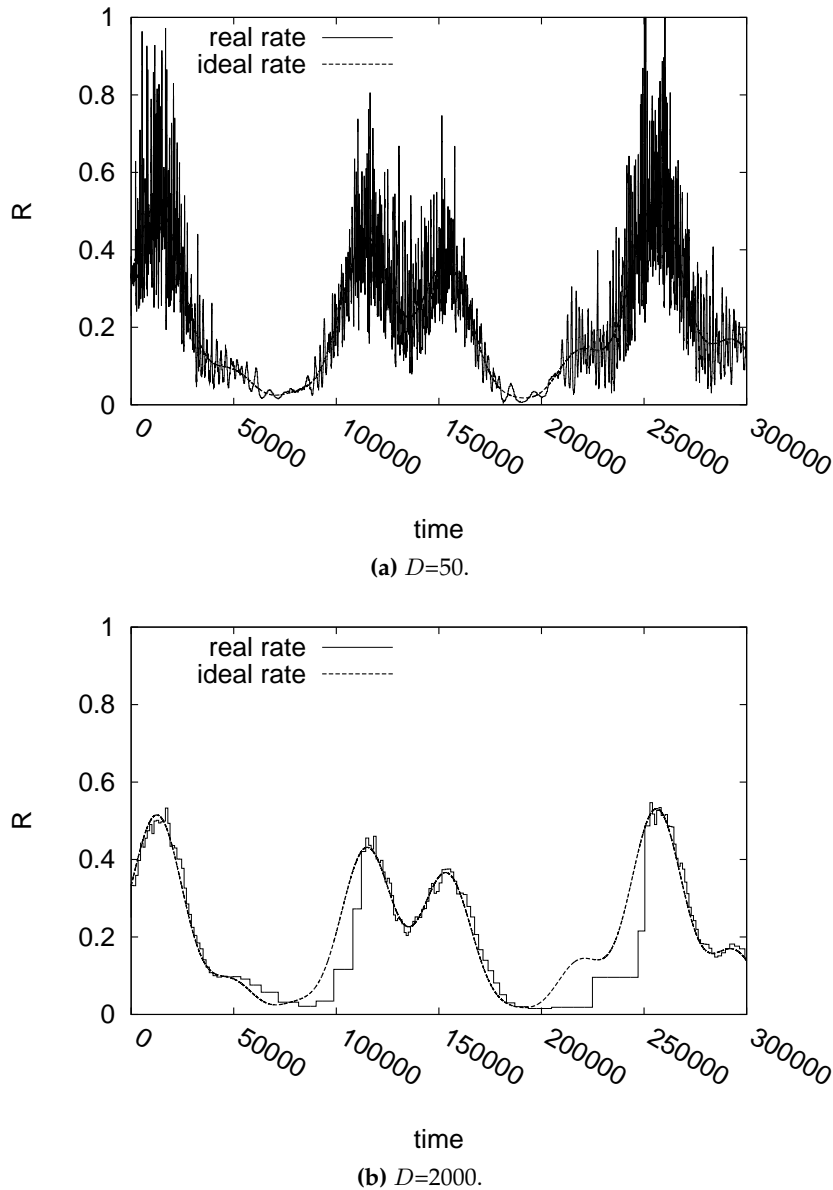
Figure 6.11: Adaptive Proactive Scheme: Simulation with synthetic data. Comparison of R_{inst} and R_{ideal} for D = 50 and D = 2000 .
