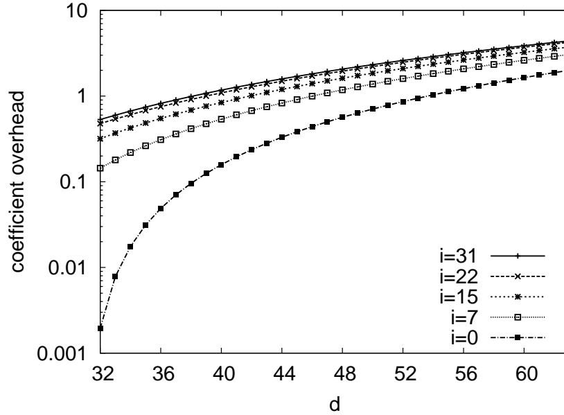
Figure 4.5: Coefficient overhead of RC(32, 32, d, i) for a 1 MByte file.
