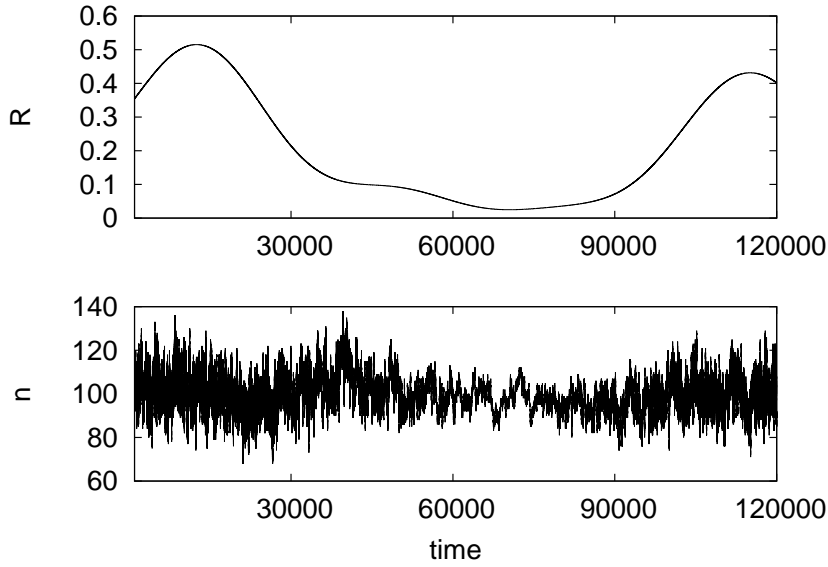
Figure 6.7: Simulation with varying parameters and an ideal estimator. Repair rate R and evolution of the number of available parity blocks.
