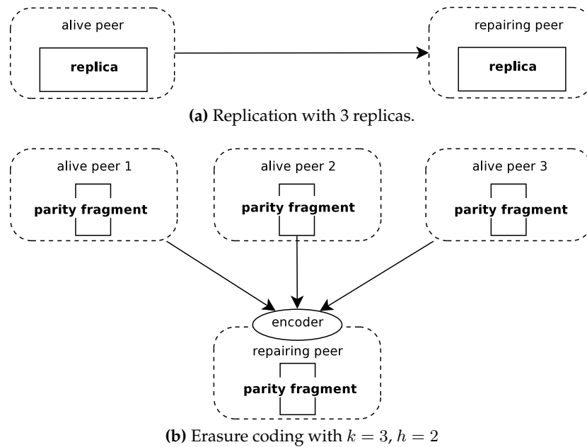
Figure 1.5: Redundancy schemes: data repair.
