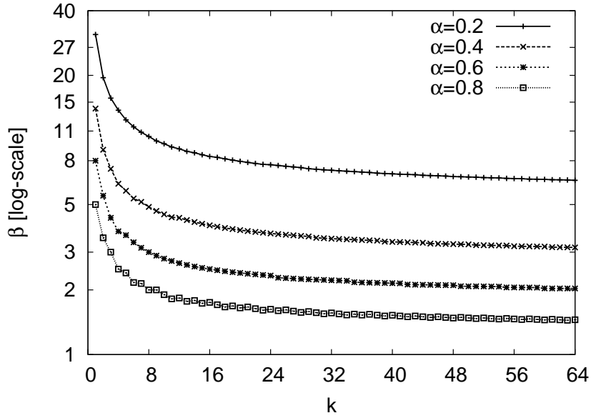
Figure 3.2: Redundancy factor \beta required for an availability of 99% as function of the up ratio \alpha and the number of original fragments k the file is cut into.
