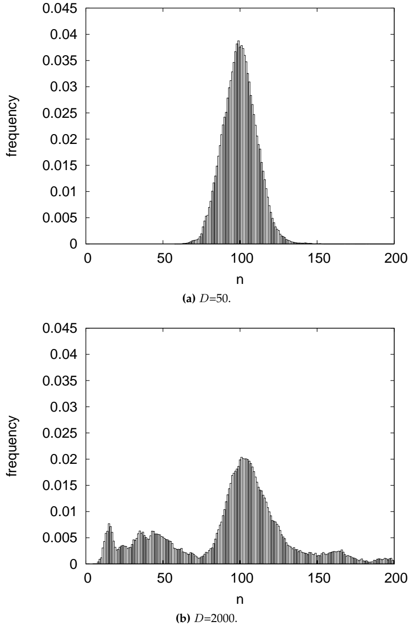
Figure 6.10: Adaptive Proactive Scheme: Simulation with synthetic data. Distribution of the number of available parity blocks for D = 50 and D = 2000 .
