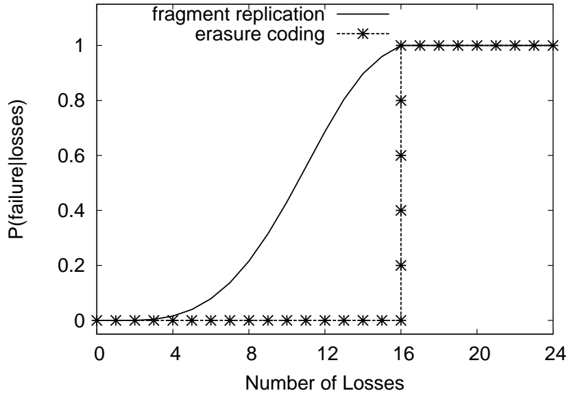
Figure 5.1: Fragment replication scheme compared to erasure codes with k = 8 and N_{rep} = 3 . P(\text{failure}|l) as function of the number of concurrent losses l .
