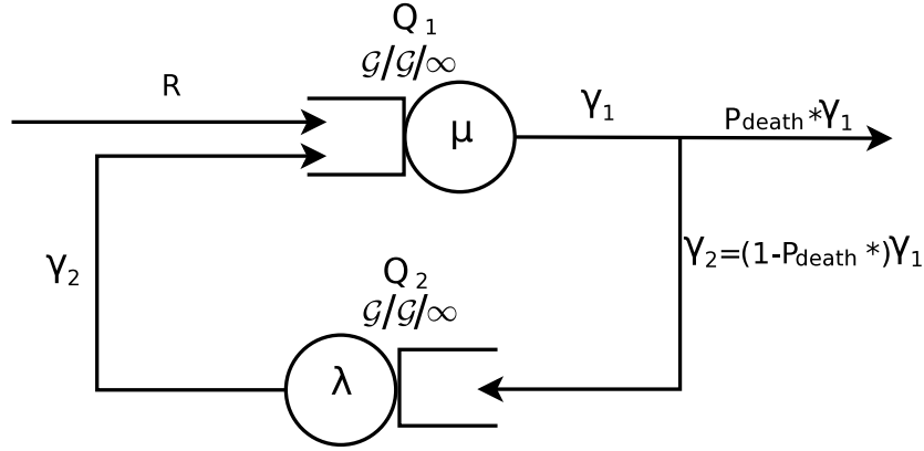
Figure 6.3: Queuing system representing the overall system behavior.
