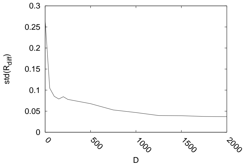
(b) Standard deviation of R_{diff} .
