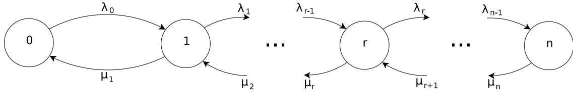
Figure 3.7: Generic birth-death process with closed population.
