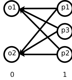
Figure 5.2: Example of a Code Graph for a classical (2,1)-linear erasure code. All the parity fragments p_1 , p_2 and p_3 are obtained as a linear combination of the two original fragments o_1 and o_2 .
