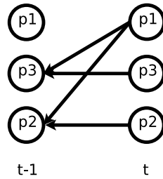
Figure 5.3: Example of one step of an Information Flow Graph . Parity fragments p_2 and p_3 have survived at time t - 1 . Parity fragment p_1 has been lost at time t - 1 and has been repaired at time t combining the parity fragments p_2 and p_3 .
