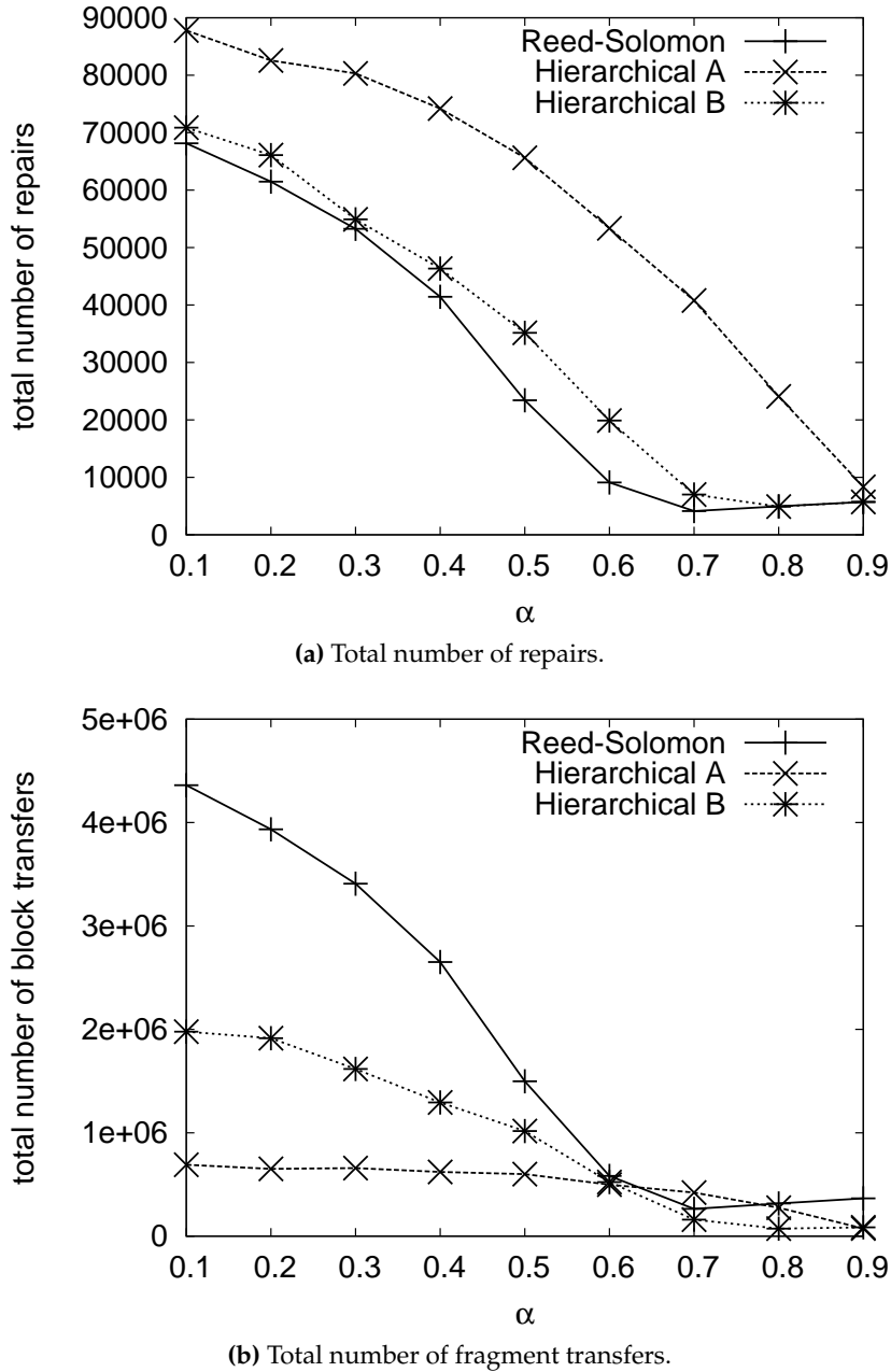
Figure 5.8: Cost of maintenance for Reed-Solomon and Hierarchical (64,64)-codes as function of the up ratio \alpha = T_{on}/(T_{on} + T_{off}) . a = 10, T = 3T_{off} .
