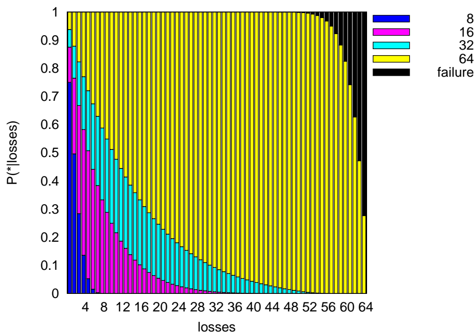
(b) Hierarchical Code B.
