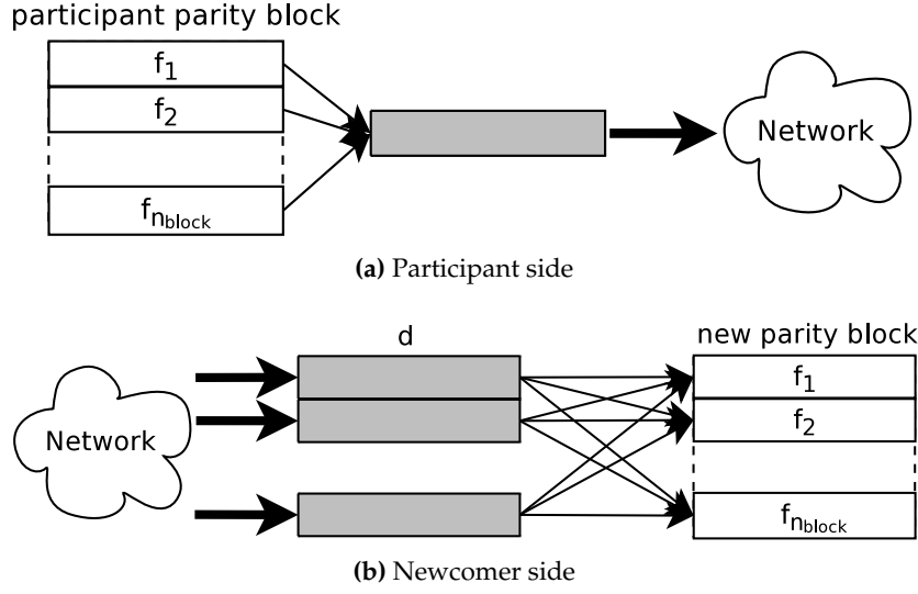
Figure 4.4: Repair scheme on the participant side and on the newcomer side. Every arrow indicates a participation to a random linear combination.
