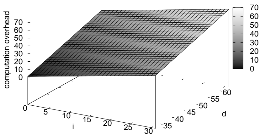
Figure 4.6: Encoding computation overhead for RC(32, 32, d, i) .
