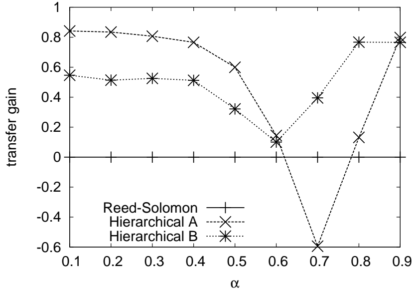
Figure 5.9: Gain of Hierarchical (64,64)-codes in terms of number of fragment transfers with respect of Reed-Solomon (64,64)-codes as function of the up ratio \alpha = T_{on}/(T_{on} + T_{off}) . a = 10 , T = 3T_{off} .
