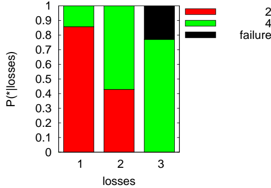
Figure 5.5: Examples of a Hierarchical (4,4)-code. P(d|l) and P(\text{failure}|l) as function of the number of concurrent losses l .
