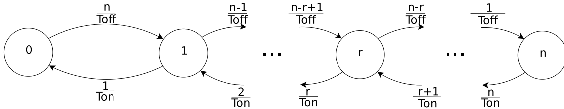
Figure 3.6: Continuous-time Markov model expressing the number of available fragments.
