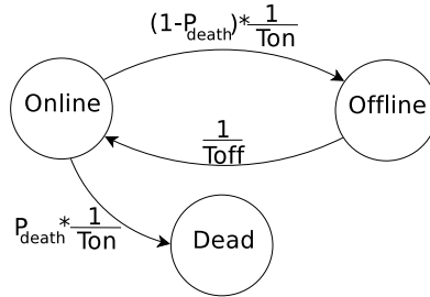
Figure 5.7: State machine modeling the behavior of a peer for Hierarchical Codes experiments.
