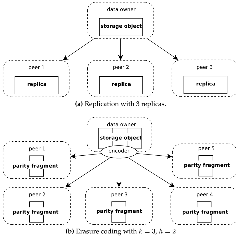
Figure 1.4: Redundancy schemes: data insertion.
