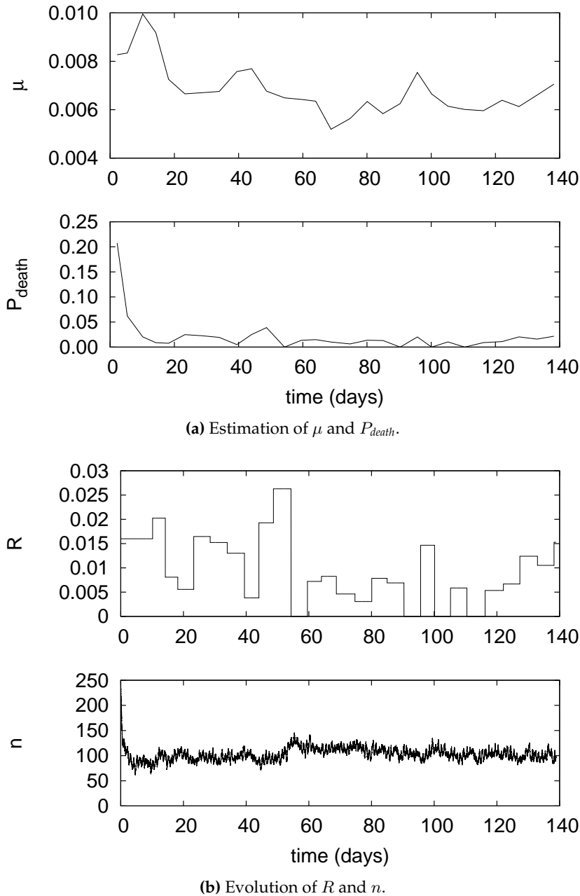
Figure 6.16: Proactive scheme with D = 1000 on KAD traces.
