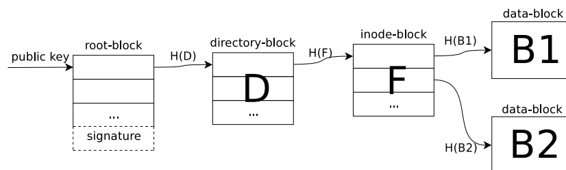
Figure 1.6: Data layout in CFS.
