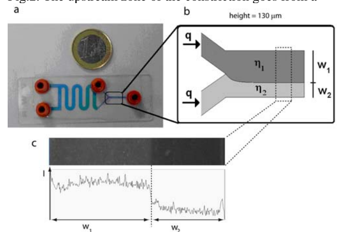
Fig.3. a) Picture of the chip with its connectors, the serpentine reservoir and the viscosimeter. b) Schematic focus on the viscosimeter and its principle. c) Experimental image of the interface and fluorescence intensity profile along the width from which the interface position is determined.
