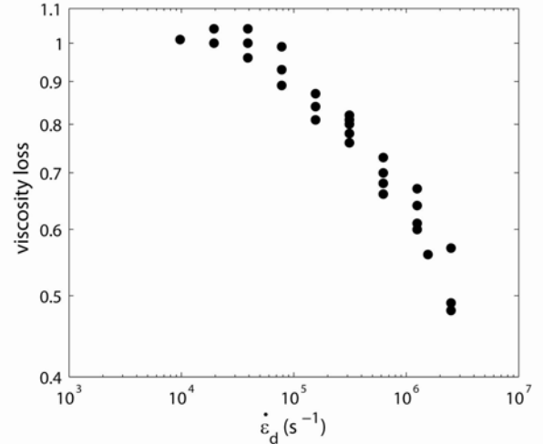
Fig.8. Viscosity ratio measured in the chip at \dot{\gamma}_m = 5.5 \text{ s}^{-1} versus the maximum imposed deformation rate \dot{\epsilon}_d for a 0.4% 5 MDa PEO solution.
