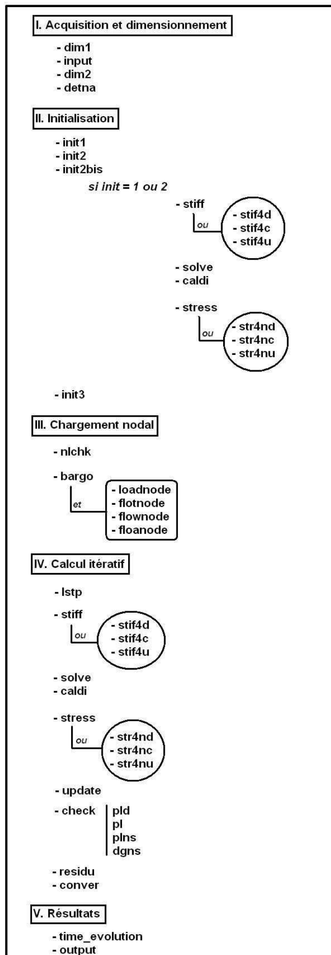
FIGURE 12.1 – Principales subroutines du programme \Theta -Stock.
