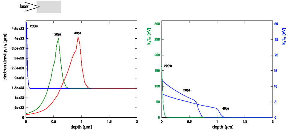
Figure 5.1: Excerpt from the simulations in Fig.4.13 for the evolution beyond the target boundary. ( left ) The shock propagates deeper into the bulk; ( right ) the evolution of the electron temperature. (The 20\text{ps} and the 40\text{ps} plots in the right graph are referred to the rightmost scale of temperature).
