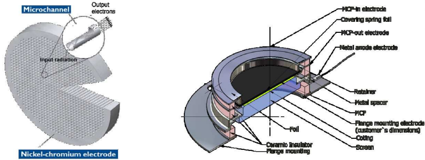
Figure 6.10: Graphical representation of the MC plate (left) and of its assembly (right).
