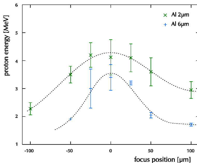
Figure 7.4: Proton cutoff energy for different focus position on Aluminum targets of 6\mu\text{m} and 2\mu\text{m} . In the entire scanned area, more energetic protons are generated from the thinner target (dashed lines are added to help visualization).
