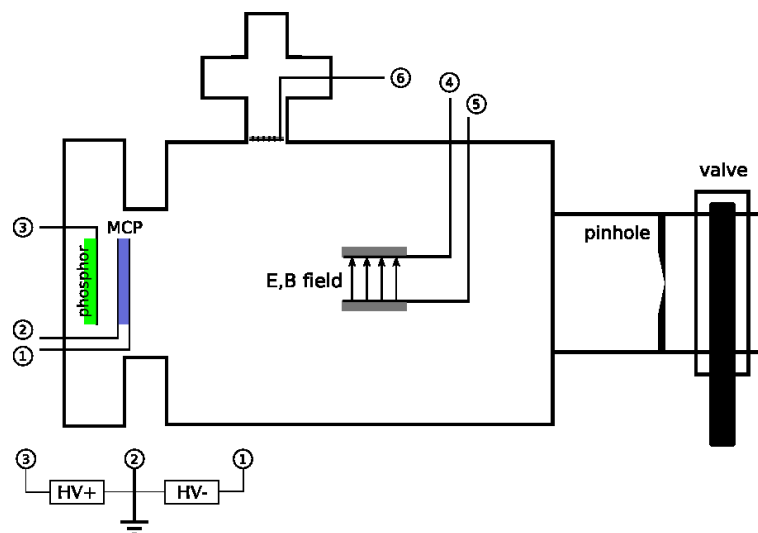
Figure 6.13: Schematics of the TP+MCP chamber (1)-(2) electrodes for MCP polarization; (3) phospor input electrode; (4)-(5) electrodes for TP electric field; (6) shielding gate
