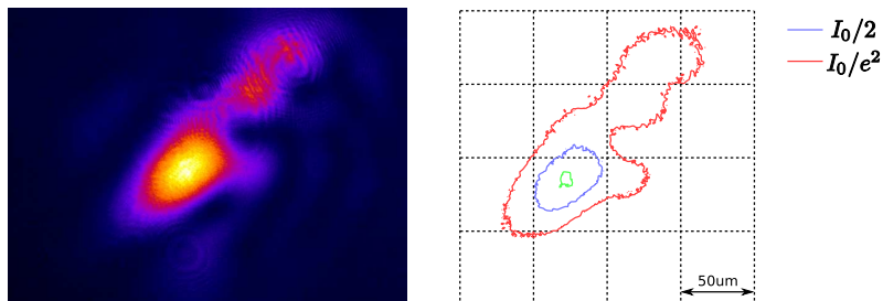
Figure 4.5: CCD image and intensity contours of the focal spot
