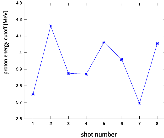
Figure 7.13: Proton cutoff energy for 8 shots in a row on 3\mu\text{m} thick aluminum target. The average energy is E_p = 3.9\text{MeV} with a peak-to-valley fluctuation of 12%.
