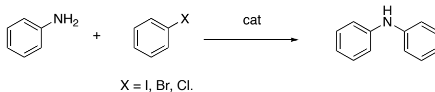
Scheme 23: Palladium catalyzed amination of haloarenes.
