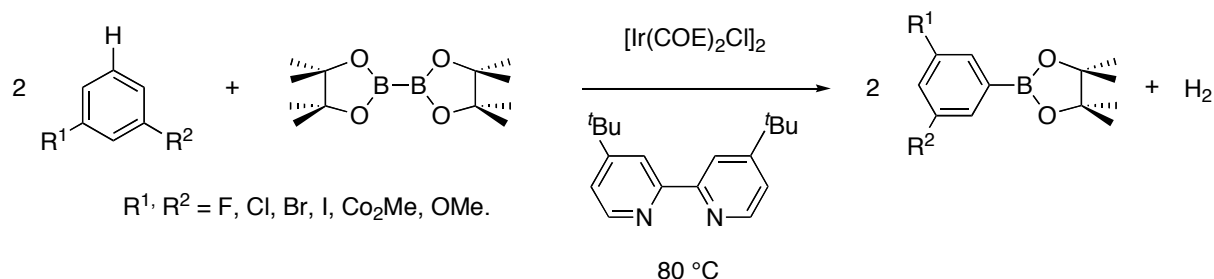
Scheme 11: Borylation of arenes catalyzed by a bipyridine iridium complex.
