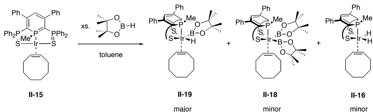
Scheme 28: Reaction of II-15 with an excess of pinacolborane.
