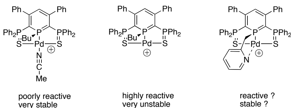
Scheme 13: Cationic \text{SPS}^{\text{R}} palladium pincer complexes.
