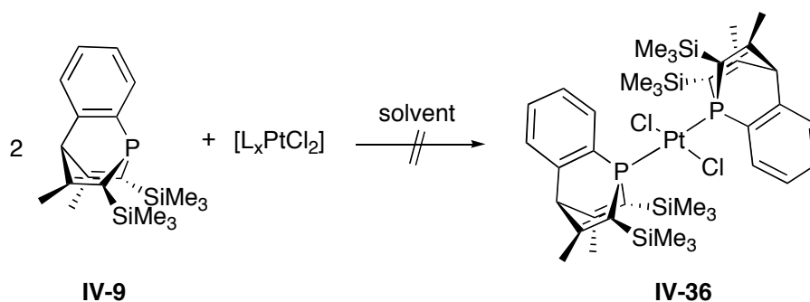
Scheme 17: Attempted synthesis of platinum complex IV-36 .
