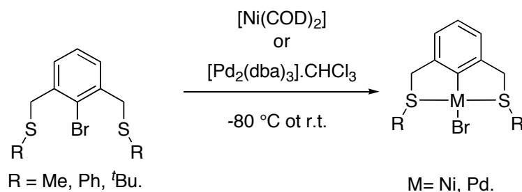
Scheme 3: Synthesis of SCS-palladium and nickel pincer complexes from zerovalent metal precursors.
