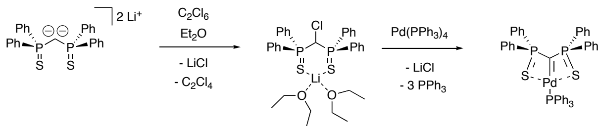
Scheme 9: Synthesis of a room temperature stable carbenoide and its reaction with \text{Pd(PPh}_3)_4 .
