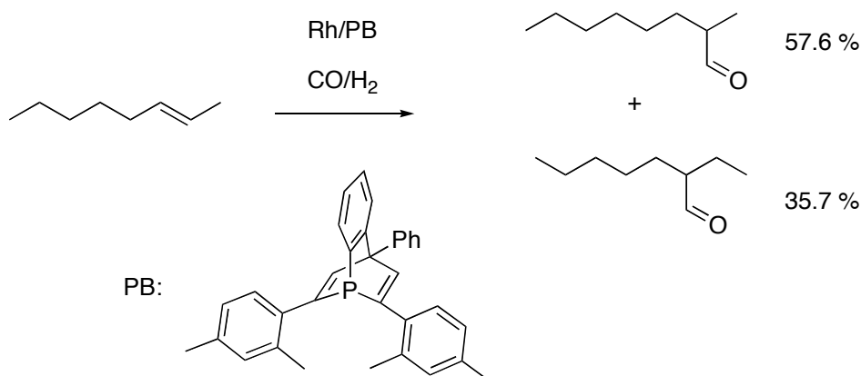
Scheme 29: Application of 1-phosphabarrelenes as ligands in hydroformylation of internal alkynes.
