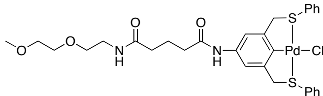
Scheme 4: Recyclable SCS-palladium catalyst for the Heck reaction.
