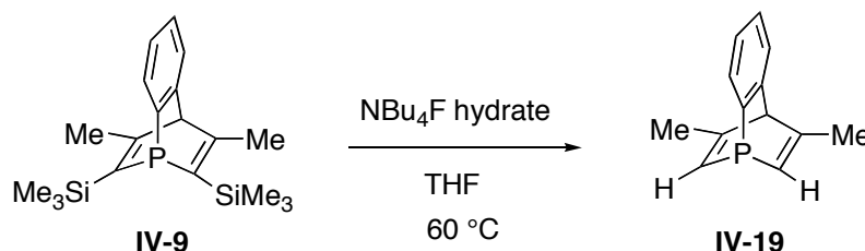
Scheme 29: Hydrodesilylation of phosphabarrelene IV-9.
