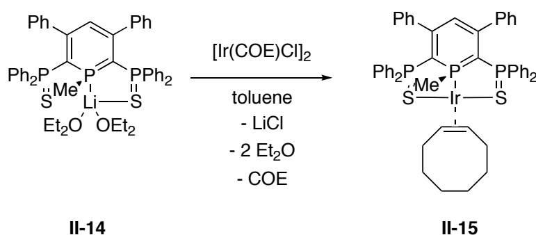
Scheme 16: Synthesis of [(SPSMe)Ir(COE)] II-15 .
