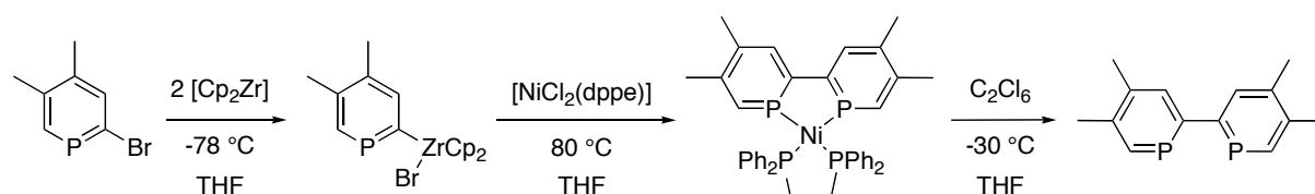
Scheme 8: Synthesis of a 2,2'-biphosphinine.
