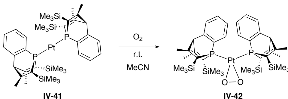
Scheme 22: Formation of an oxygen adduct of platinum(0)-complex IV-42 .
