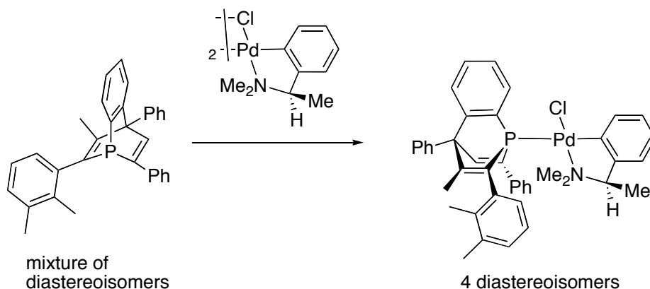
Scheme 5: Determination of diastereomeric ratio of atropoisomeric phosphabarrelenes with a chiral palladium complex.
