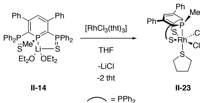
Scheme 22: Synthesis of complex II-23.
