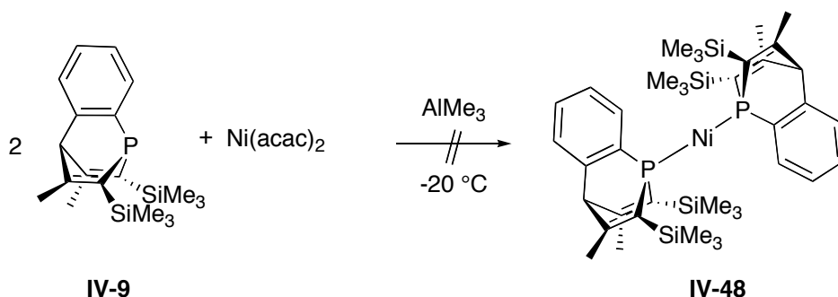
Scheme 29: Attempted synthesis of complex IV-48.
