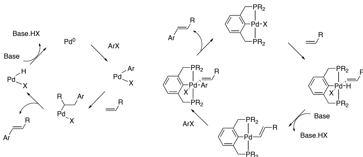
Scheme 18: Postulated mechanisms for the Heck reaction. Left: Classical mechanism based on \text{Pd(0)}/\text{Pd(II)} intermediates. Right: Mechanism proposed by Morales-Morales and Jensen based on \text{Pd(II)}/\text{Pd(IV)} intermediates.
