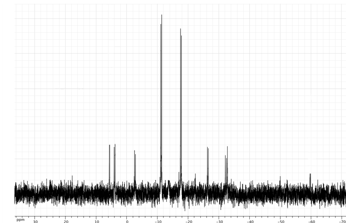
Figure 1: ^{31}\text{P} NMR spectrum of the reaction of IV-41 with phenylacetylene leading to IV-72 .
