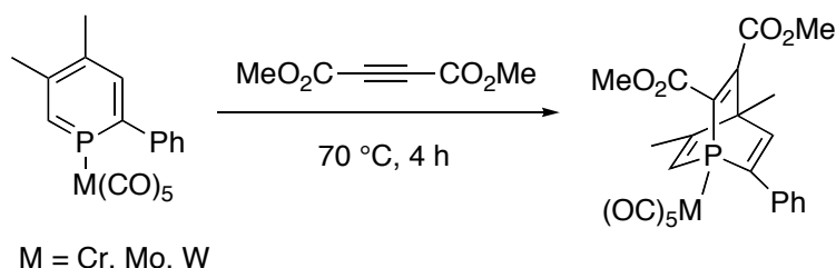
Scheme 1: Synthesis of group 6 complexes of phosphabarrelenes by Mathey and Märkl.
