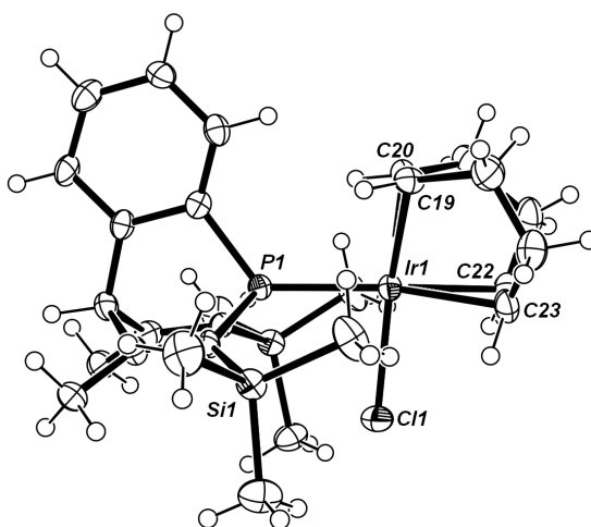
Figure 22: Molecular structure (ORTEP-representation, thermal ellipsoids at a 50 % probability) of complex 58. Selected bond lengths [ \text{\AA} ] and angles [ ^\circ ]: Ir1-P1: 2.325, Ir1-Cl1: 2.382, Ir1-C19: 2.108, Ir1-C23: 2.176, C19-C20: 1.425, C23-C24: 1.390 P1-Ir1-Cl1: 84.63.
