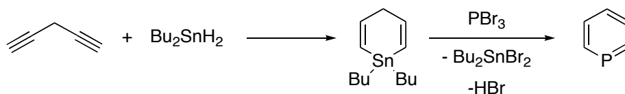
Scheme 2: Synthesis of the parent-phosphinine C_5H_5P by Ashe.
