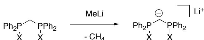
Scheme 32: Envisaged synthesis of anionic pincer ligands derived from dppm.
