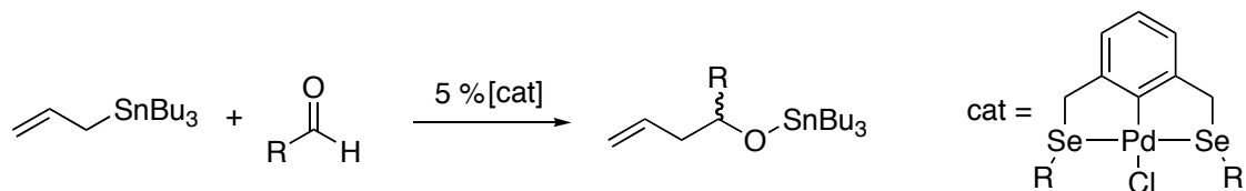
Scheme 11: Allylation of aldehydes with tributylallyltin catalyzed by a SeCSe palladium pincer complex.
