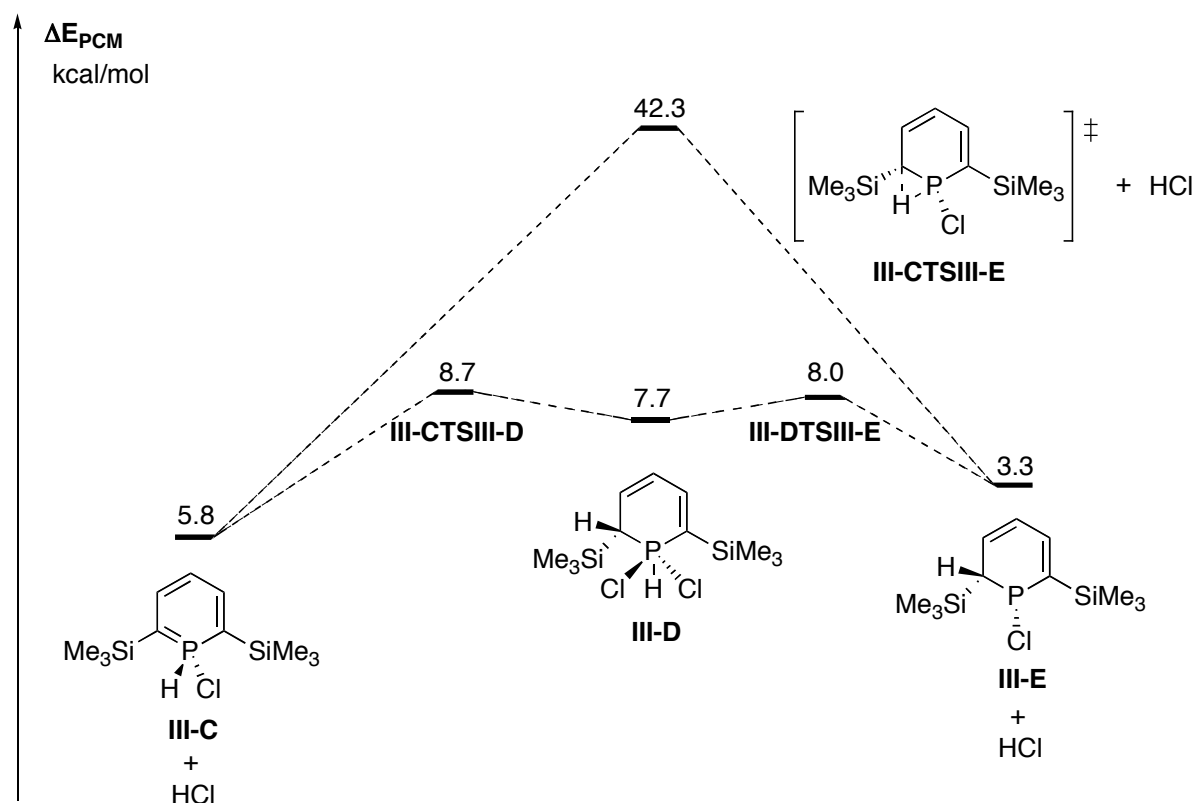
Scheme 9: Isomerisation of \lambda^5 -phosphenine III-C to phosphine III-E .
