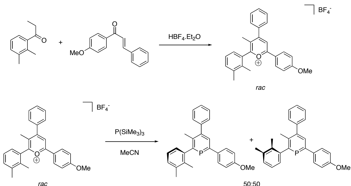
Scheme 15: Synthesis of atropoisomeric pyrilium salts and phosphinines.
