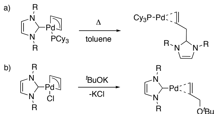
Scheme 14: Reduction of allylpalladium complexes (a) by reductive elimination, (b) by nucleophilic attack by alkoxides.
