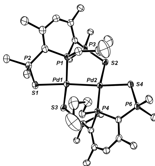
Figure 7: Molecular structure of complex II-11 (ORTEP-Plot, thermal ellipsoids with 50 % probability, phenyl groups and hydrogen atoms were omitted for clarity) Selected bond lengths[Å] and angles[°]: Pd(1)-Pd(2): 2.5815(3), P(1)-Pd(1): 2.2515(8), Pd1-S1: 2.4171(8), Pd(1)-S(3): 2.3540(8), S(1)-Pd(1)-Pd(2): 174.02(2), P(1)-Pd(1)-S(3): 167.37(3).
