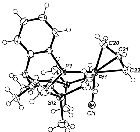
Figure 12: Molecular structure (ORTEP-representation, thermal ellipsoids at a 50 % probability) of complex IV-39 . Selected bond lengths [ \text{\AA} ] and angles [ ^\circ ]: Pt1-P1: 2.261(1), Pt1-Cl1: 2.373(1), Pt1-C20: 2.100(6), Pt1-C22: 2.18(3), P1-Pt1-C22: 171.4(7), P1-Pt1-Cl1: 85.68(5), C20-Pt1-Cl1: 167.6(2).
