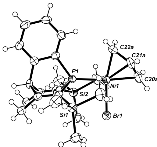
Figure 17: Molecular structure (ORTEP-representation, thermal ellipsoids at a 50 % probability) of complex IV-43 . Selected bond lengths [ \text{\AA} ] and angles [ ^\circ ]: Ni1-P1: 2.198(2), Ni1-Br1: 2.335(1), Ni1-C20a: 2.061(6), Ni1-C22a: 2.000(6), P1-Ni1-C20a: 172.8(2), P1-Ni1-Br1: 92.59(5).
