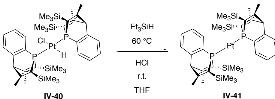
Scheme 17: Reduction of complex IV-40 with triethylsilane.
