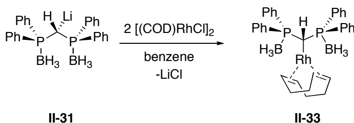
Scheme 10: Reaction of II-31 with [(\text{COD})\text{RhCl}]_2 .
