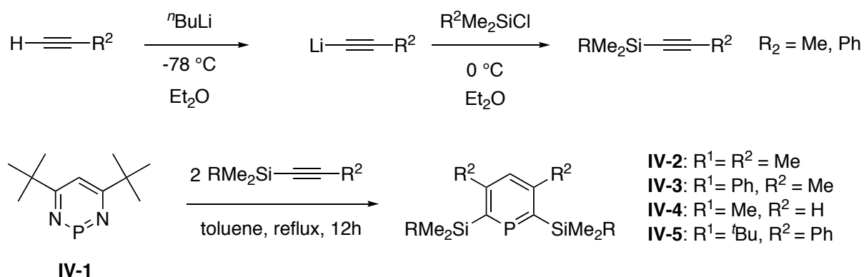
Scheme 20: Synthesis of 2,6-disilyl-substituted phosphanes IV-2 - IV-5.
