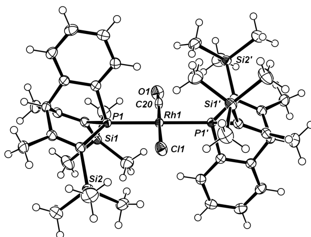
Figure 19: Molecular structure (ORTEP-representation, thermal ellipsoids at a 50 % probability) of complex IV-51 . Selected bond lengths [ \text{\AA} ] and angles [ ^\circ ]: Rh1-P1: 2.3341(5), Rh1-Cl1: 2.343(2), Rh1-C20: 1.82(1), P1-Rh1-P1': 180.0 ^\circ , C20-Cl1: 178.2(4).
