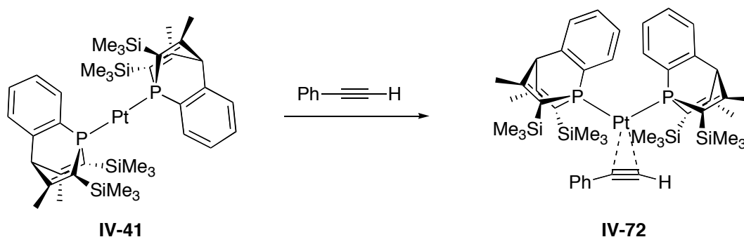
Scheme 19: Reaction of IV-41 with phenylacetylene.
