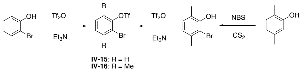
Scheme 26: Synthesis of benzyne precursors IV-15 and IV-16 .
