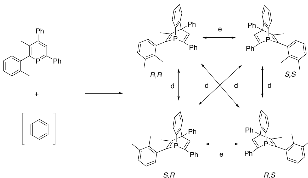
Scheme 19: Synthesis of chiral phosphabarrelenes starting from an atropisomeric phosphinine (e: enantiomers; d: diastereoisomers).
