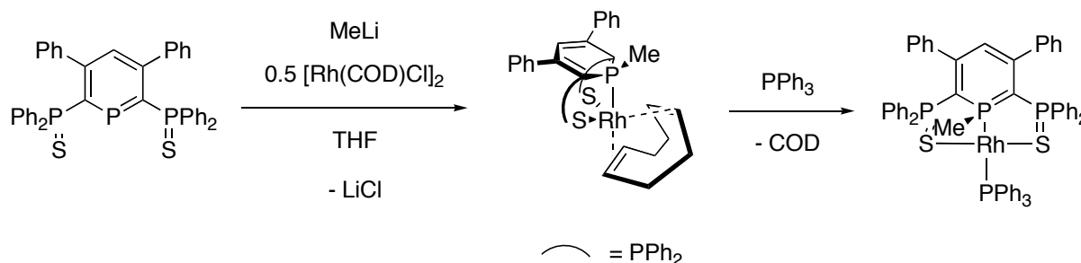
Scheme 5: Synthesis of [(SPS Me )Rh(COD)] and [(SPS Me )Rh(PPh 3 )] complexes.
