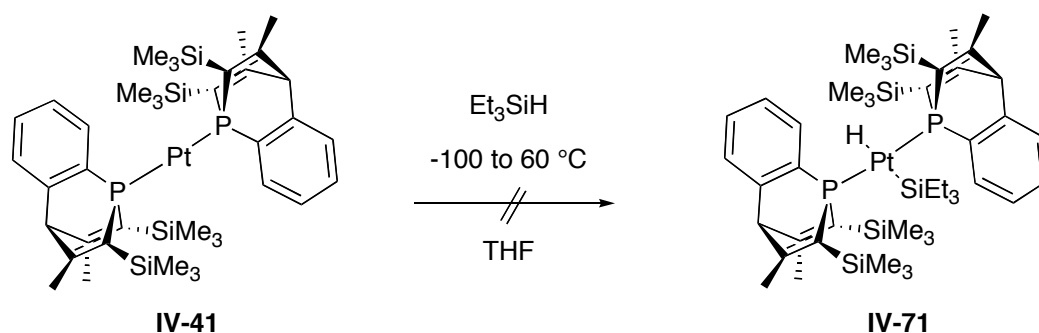
Scheme 18: Reactivity of complex IV-41 towards triethylsilane.
