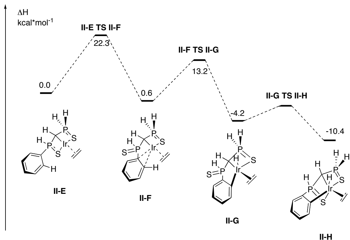
Scheme 15: Computed energetic pathway for the conversion of II-E into II-H .
