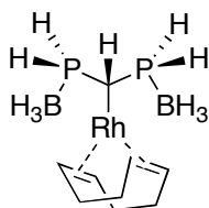
Scheme 12: Model complex used for structure optimization.
