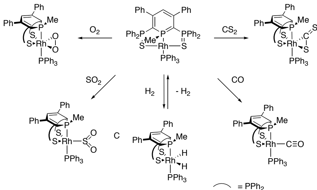
Scheme 6: Fixation of small molecules by the [(\text{SPS}^{\text{Me}})\text{Rh}(\text{PPh}_3)] -complex.
