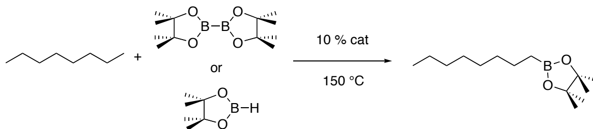
Scheme 30: Attempted borylation of n -octane catalyzed by complexes II-15 , II-21 , II-22 and II-23 .
