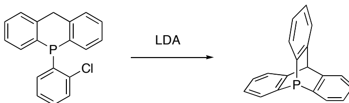
Scheme 6: Synthesis of 9-phosphatriptycene by Bickelhaupt and coworkers.
