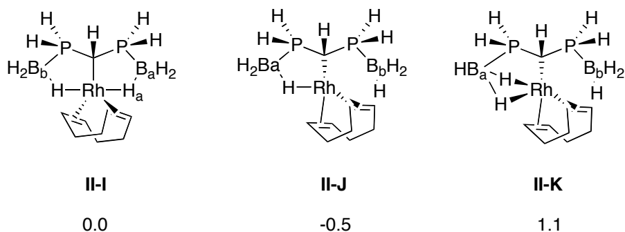
Scheme 13: Relative free energies of calculated structures II-I - II-K in kcal mol -1
