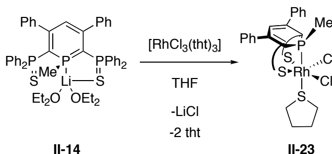
Scheme 29: Synthesis of a [(SPS^{Me})RhCl_2(tht)] II-23 .
