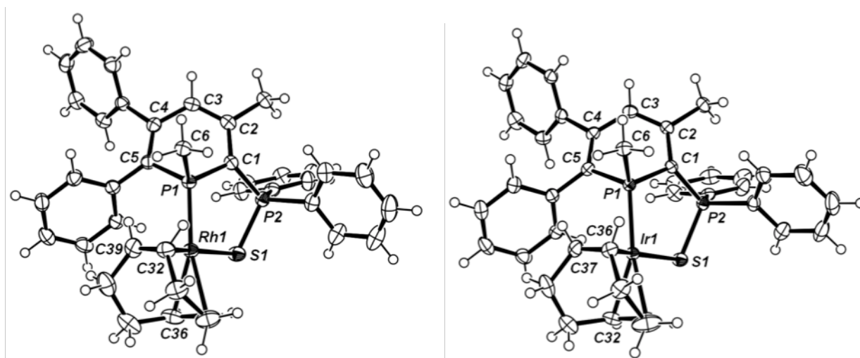
Figure 2: Molecular structure of complex II-21 (left) and II-22 (right) (ORTEP-Plot, thermal ellipsoids with 50 % probability, phenyl groups and hydrogen atoms were omitted for clarity, The products crystallized as racemic mixtures, only one enantiomer is presented) Selected bond lengths[Å] and angles[°] for II-21 : Rh1-P1: 2.2778(5), Rh1-S1: 2.3431(5), P1-Rh1-S1: 87.86(2). Selected bond lengths[Å] and angles[°] for II-22 : Ir1-P1: 2.2808(6), Ir1-S1: 2.3301(6), P1-Ir1-S1: 89.15(2).
