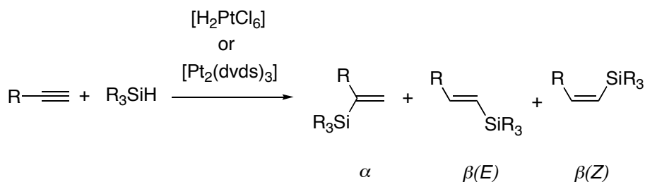
Scheme 13: Hydrosilylation of terminal alkynes with the Speier or the Karstedt catalyst.
