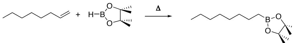
Scheme 25: Thermal hydroboration of oct-1-ene.
