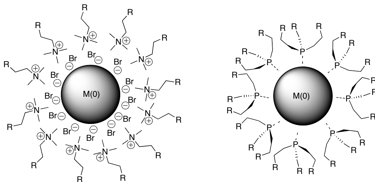
Scheme 7: Stabilization of NPs through a) electrostatic interactions and b) coordination.
