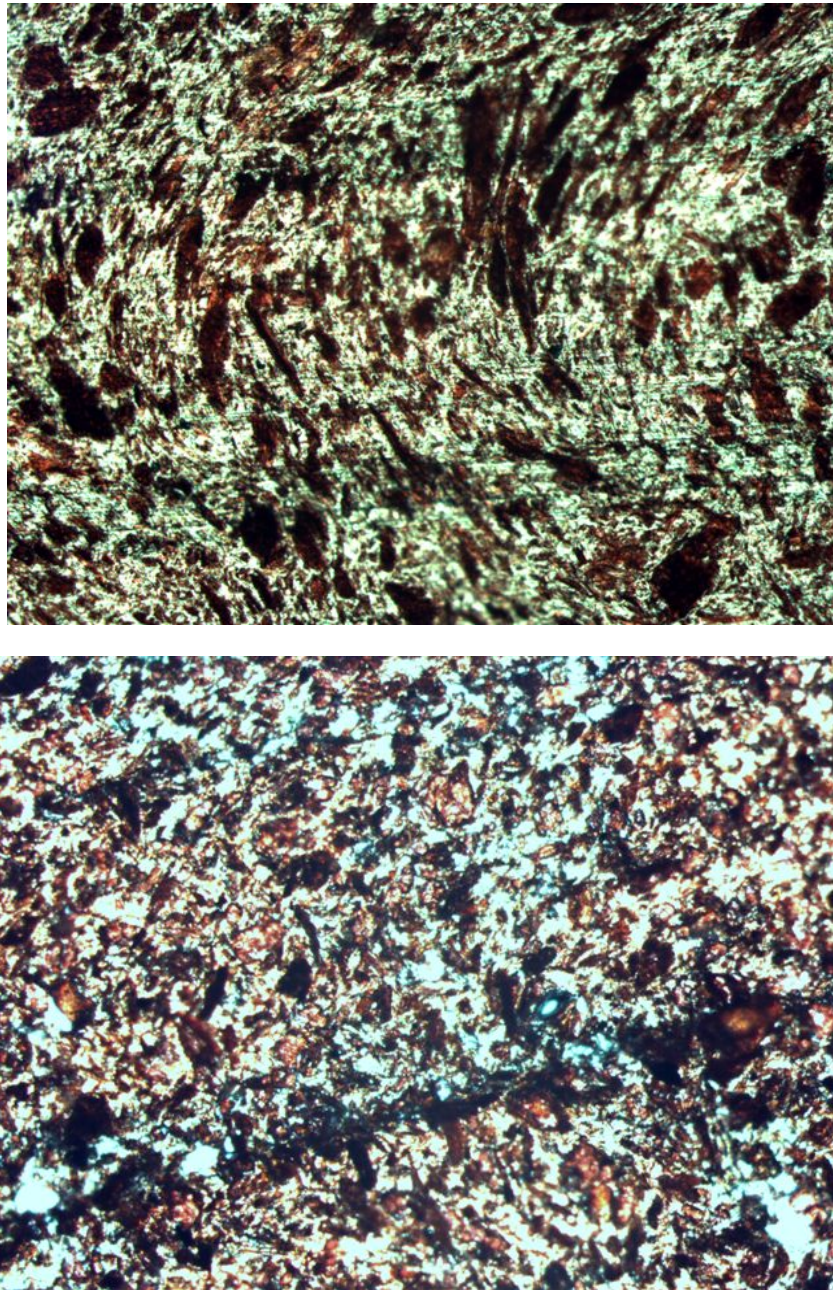
Appendix 5. Example of transversal section (x5) of the structure of an injected moulding composite made with 45 wt% jack pine wood particle (top) and bark particle (bottom). Initially mean size of the particles was 42 mesh.
