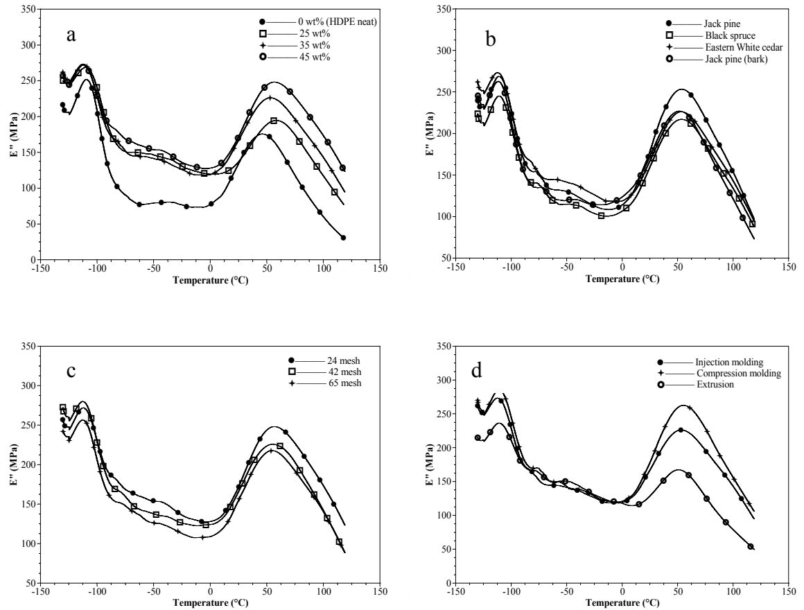
Figure 8.2. Loss modulus of (a) eastern white cedar particle (42 mesh)/HDPE composites, (b) wood particle (35 wt%, 24 mesh)-based composites (c) jack pine (35 wt%)/HDPE composites and (d) jack pine(35wt%, 24 mesh)/HDPE composites.
