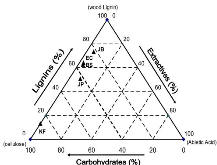
Figure 4.7. Ternary diagram of the surface component fraction of the used fibers (KF: bleached Kraft fiber; JP: jack pine; BS: black spruce; EC: eastern white cedar; JB: jack pine bark).
