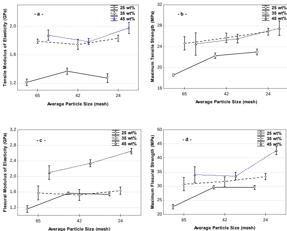
Figure 6.5. Effect of wood particle size with various filler contents on (a) tensile modulus of elasticity (b), tensile strength, (c) flexural modulus of elasticity, and (d) flexural strength of WPC.
