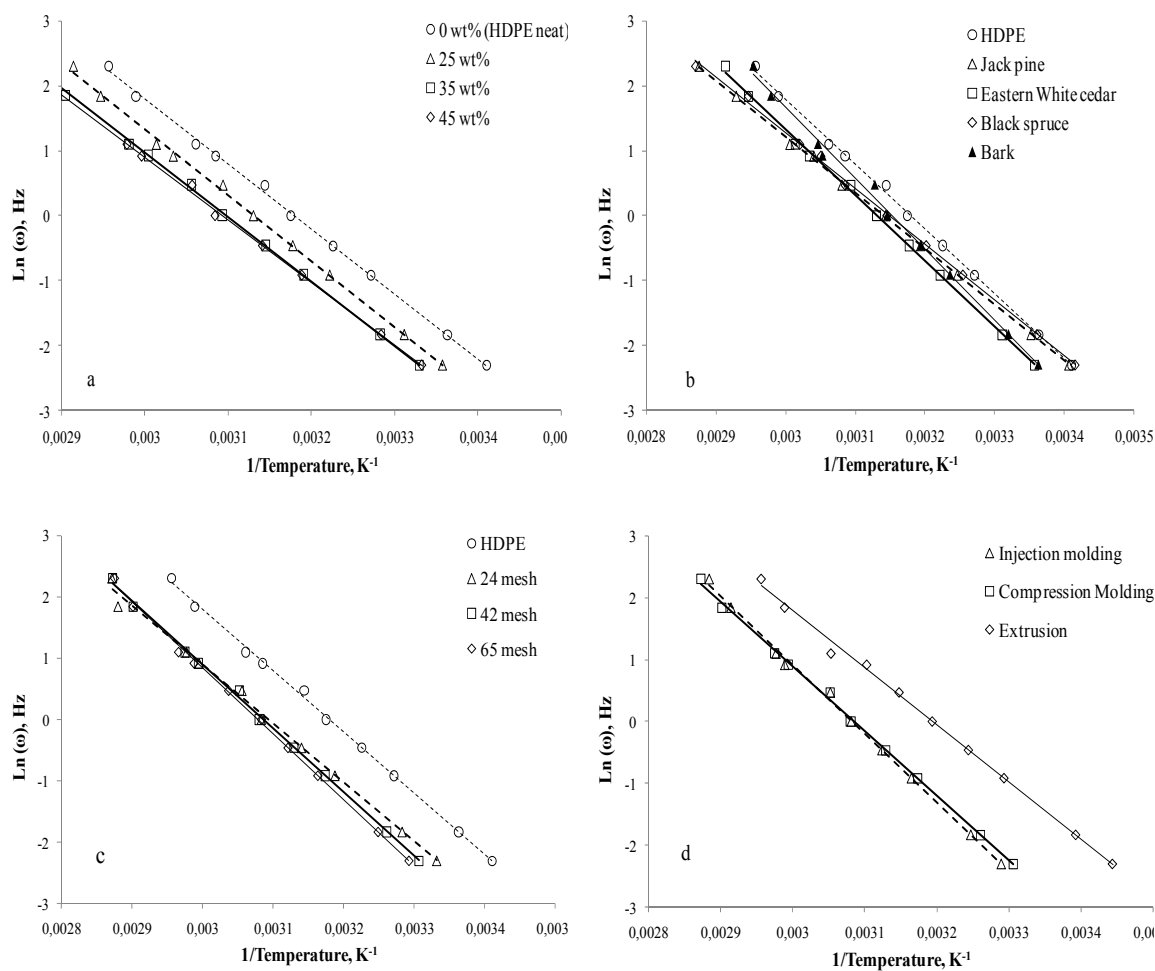
Figure 8.4. Examples of Arrhenius plots for \alpha -relaxation peaks of (a) eastern white cedar particle(42 mesh)/HDPE composites, (b) wood particle(35 wt%, 24 mesh)-based composites (c) jack pine(35 wt%)/HDPE composites, and (d) jack pine (35 wt%, 24 mesh)/HDPE composites
