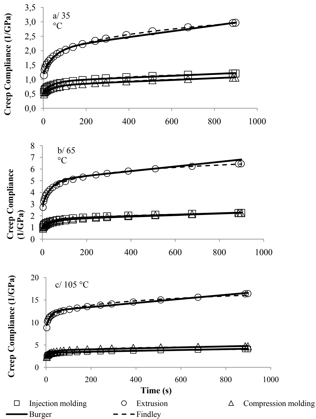
Figure 9.8. Short term creep tests for composites made with different processes. Composites containing 35wt% black spruce wood particles (24 mesh).
