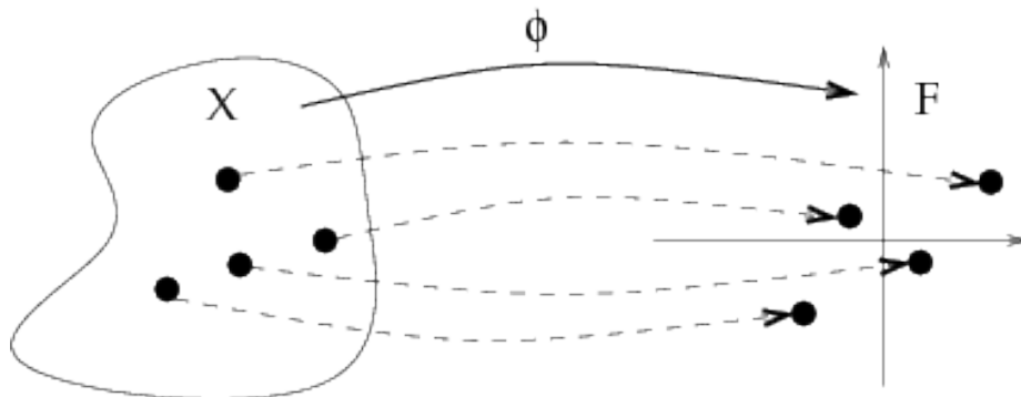
Figure 1.8: Defining a kernel over a space \mathcal{X} , such as the space of all small molecules or the space of all proteins, is equivalent to embedding \mathcal{X} in a vector space F of finite or infinite dimension through a mapping \Phi : \mathcal{X} \mapsto F . The kernel between two points in \mathcal{X} is equal to the inner products of their images in F , as shown in (1.7)
