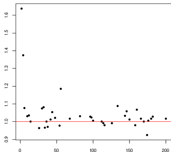
Figure 2.9: Improvement (as a performance ratio) of the hierarchy GPCR kernel against the Dirac GPCR kernel as a function of the number of training samples available. Restricted to [2 - 200] samples for the sake of readability.
