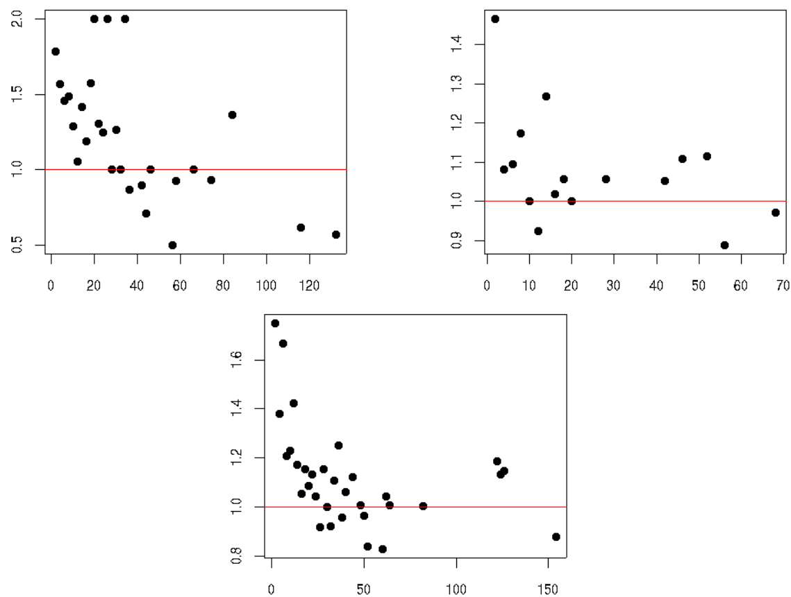
Figure 2.7: Relative improvement of the hierarchy kernel against the Dirac kernel as a function of the number of known ligands for enzymes, GPCR and ion channel datasets. Each point indicates the mean performance ratio between individual and hierarchy approaches across the targets of the family for which a given (x-axis) number of training points was available.
