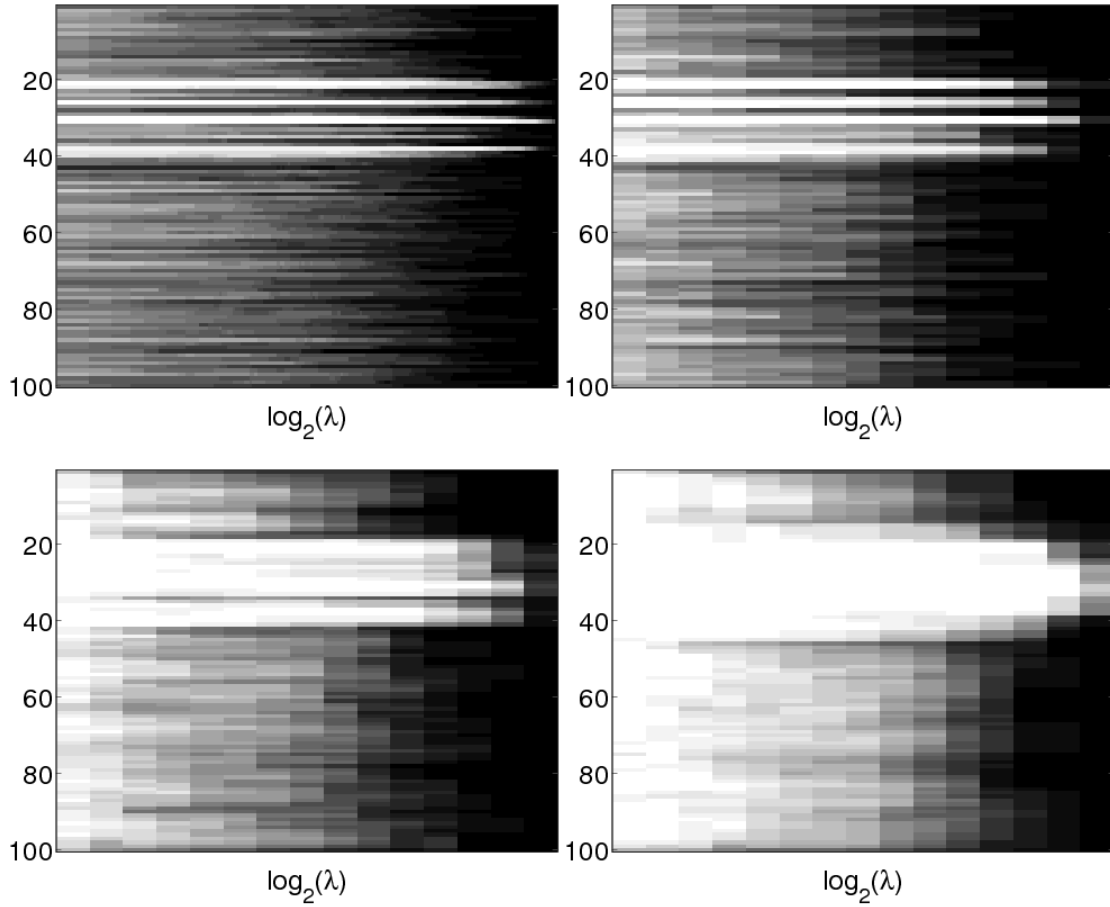
Figure 4.6: Variable selection frequency with \Omega_{\text{overlap}}^{\mathcal{G}}(\cdot) using the chains of length k (left) as groups, for k = 1, 2, 4, 8 .
