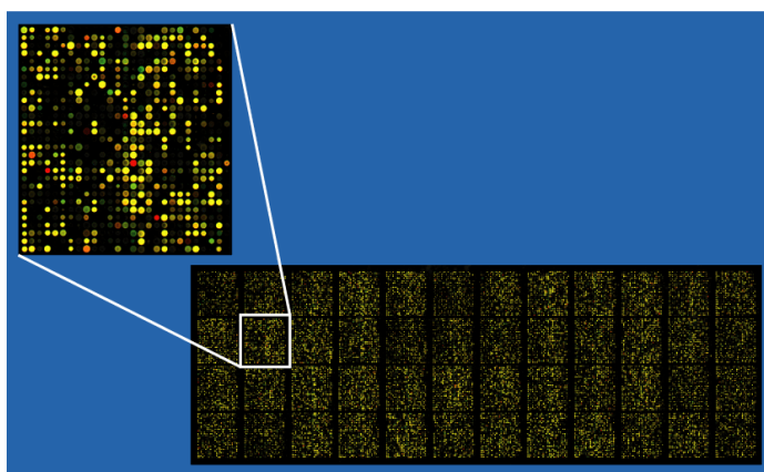
Figure 1.7: Example of an approximately 37,500 probe spotted oligo microarray with enlarged inset to show detail (source: Wikipedia).
