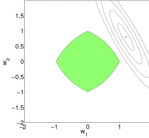
Figure 1.11: Unit ball of the elastic net \lambda_1\|w\|_1 + \lambda_2\|w\|_2 for \lambda_1 = \lambda_2 .
