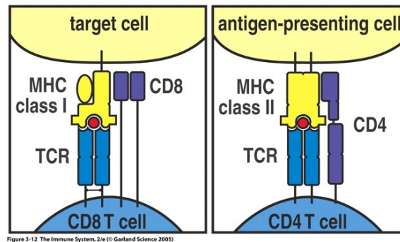
Figure 1.2: T cell – HLA molecule interaction
