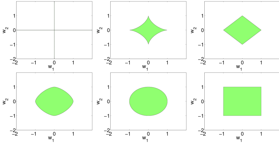
Figure 1.1: Unit balls for the \ell_p norms in two dimensions, for p = 0, \frac{2}{3}, 1, \frac{3}{2}, 2, \infty .
