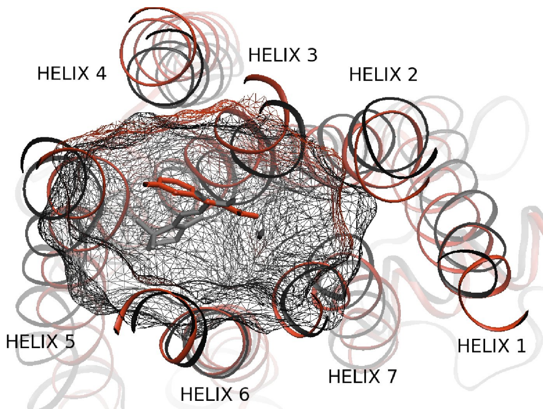
Figure 2.1: Representation of the binding pocket of \beta_2 -adrenergic receptor (in red) and bovine Rhodopsin (in black) viewed from the extracellular surface. On the center of the pocket, 3-(isopropylamino)propan-2-ol and cis-retinal have been represented to show the size and the position of the pocket around each ligand. Figure drawn with VMD (Humphrey et al., 1996).
