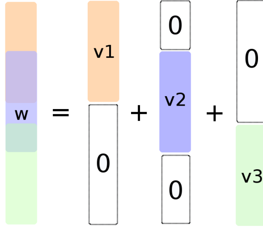
Figure 4.2: Latent decomposition of w over (v_g)_{g \in \mathcal{G}} . Applying the \ell_1/\ell_2 penalty to the decomposition instead of applying it to the w_g removes only the variables which do not belong to any selected group.
