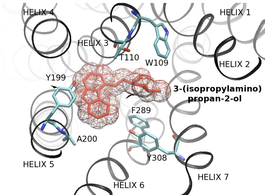
Figure 2.2: 3-(isopropylamino)propan-2-ol and the protein environment of \beta_2 -adrenergic receptor as viewed from the extracellular surface. Amino acid side chains are represented for 6 of the 31 residues (in cyan, blue and red) of the binding pocket motif. Transmembranes helix and 3-(isopropylamino)propan-2-ol are colored in black and red respectively. Figure drawn with VMD (Humphrey et al., 1996).
