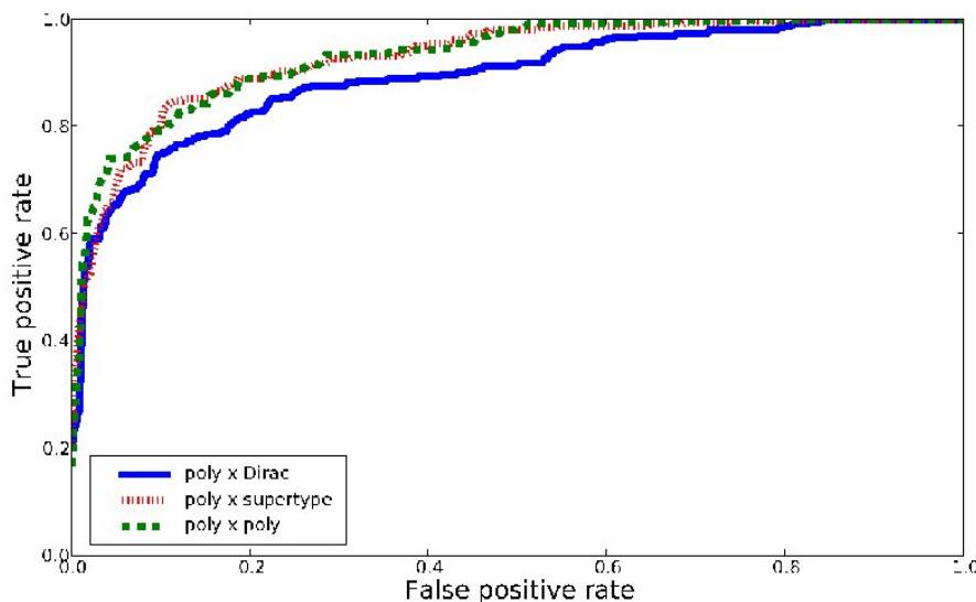
Figure 2.4: ROC curves on the pooled ten folds of the MHCBN+SYFPEITHI+LANL benchmark.
