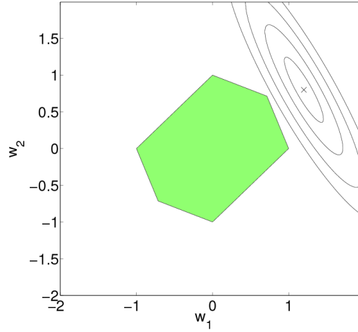
Figure 1.12: Unit ball of the fused penalty (1.22) for \lambda_1 = \frac{2}{3} , \lambda_2 = \frac{1}{3} .
