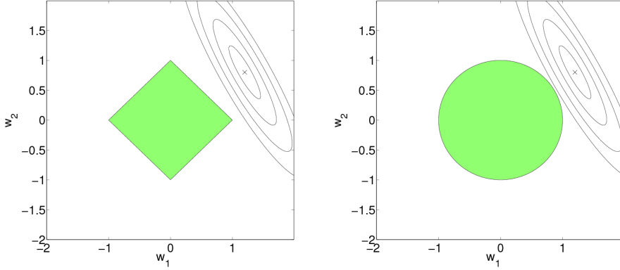
Figure 1.10: Sparsity induction by the \ell_1 norm.
