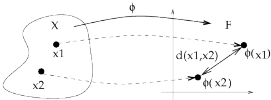
Figure 1.9: We can define the distance between two objects x_1 and x_2 , such as two molecules or proteins, as the Euclidean distance between their images \Phi(x_1) and \Phi(x_2) . If the mapping \Phi is defined by a valid kernel k , then this distance can be computed easily without computing \Phi(x_1) and \Phi(x_2) , as shown in (1.8). This kernel trick can be extended to a variety of linear algorithms that only manipulate the data through inner products.
