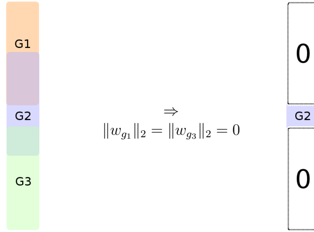
Figure 4.1: Effect of penalty (4.1) on the support. Removing any group containing a variable removes the variable from the support.
