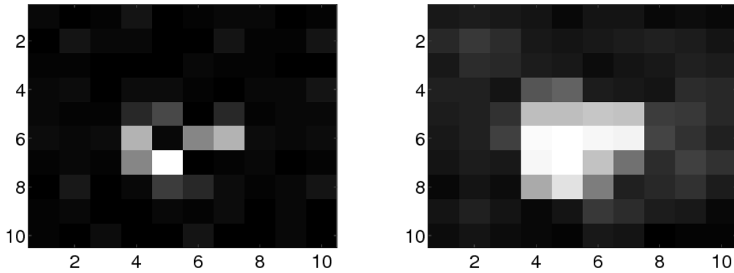
Figure 4.7: Grid view of the variable selection frequencies with the non-linear graph setting. Left: Lasso, right: \Omega_{\text{overlap}}^{\mathcal{G}}(\cdot) using 4-cycles as groups. n = 30 training points, \lambda is arbitrarily fixed.
