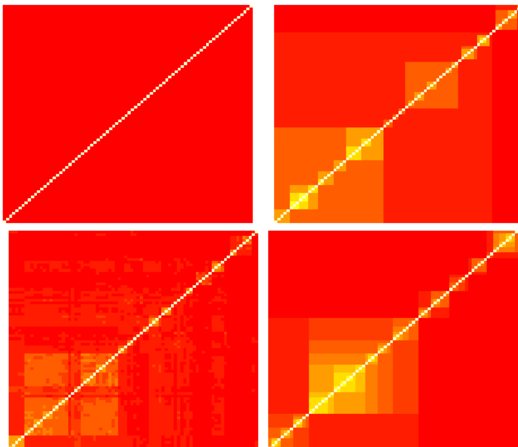
Figure 2.8: GPCR kernel Gram matrices ( K_{tar} ) for the GLIDA GPCR data with multitask, hierarchy, binding pocket and binding pocket hierarchy kernels.
