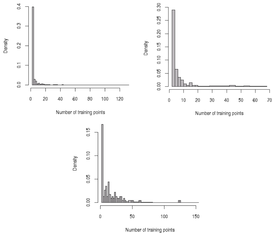
Figure 2.5: Distribution of the number of training points for a target for the enzymes, GPCR and ion channel datasets. Each bar indicates the proportion of targets in the family for which a given (x-axis) number of data points is available.
