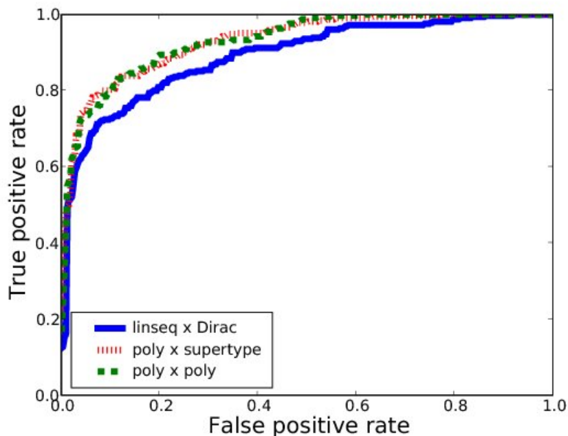
Figure 2.3: ROC curves on the pooled five folds of the SYFPEITHI+LANL benchmark.
