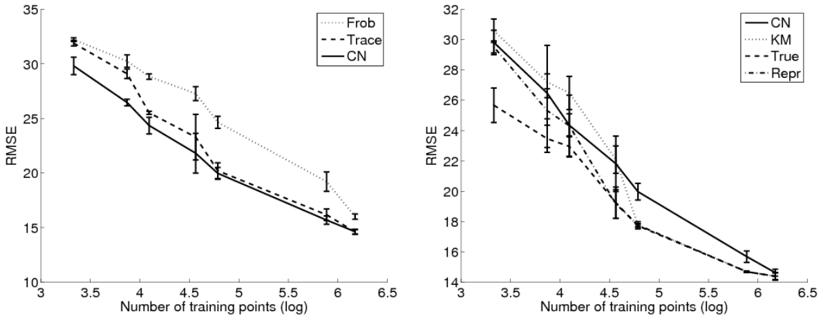
Figure 3.1: RMSE versus number of training points for the tested methods.
