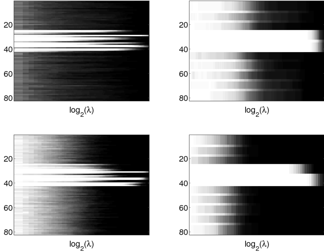
Figure 4.4: Frequency of selection of each variable with the Lasso (left) and \Omega_{\text{overlap}}^{\mathcal{G}}(\cdot) (right) for n = 50 (top) and 100 (bottom).
