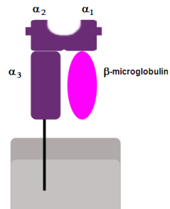
Figure 1.4: Schematic representation of MHC class I molecule (source: Wikipedia).
