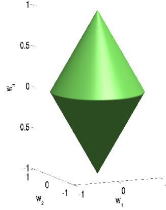
Figure 1.13: Unit ball of the group-lasso in 3 dimensions with \mathcal{G} = \{\{1, 2\}, \{3\}\} .
