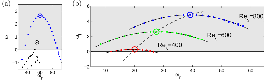
Figure 2. (a) Part of the full global spectrum showing the least-stable boundary-layer modes (in blue) and the slow-moving set of acoustic modes (in black) as presented in Mack and Schmid (2009b); unstable half-plane in light grey. (b) Least-stable eigenvalues, belonging to global boundary-layer modes, of the global spectrum for selected sweep Reynolds numbers Re_s ( Ma_s = 1.25 , \theta_w = 1 and \beta = 0.224 ). The dashed line indicates the evolution of the maximum growth rate.
