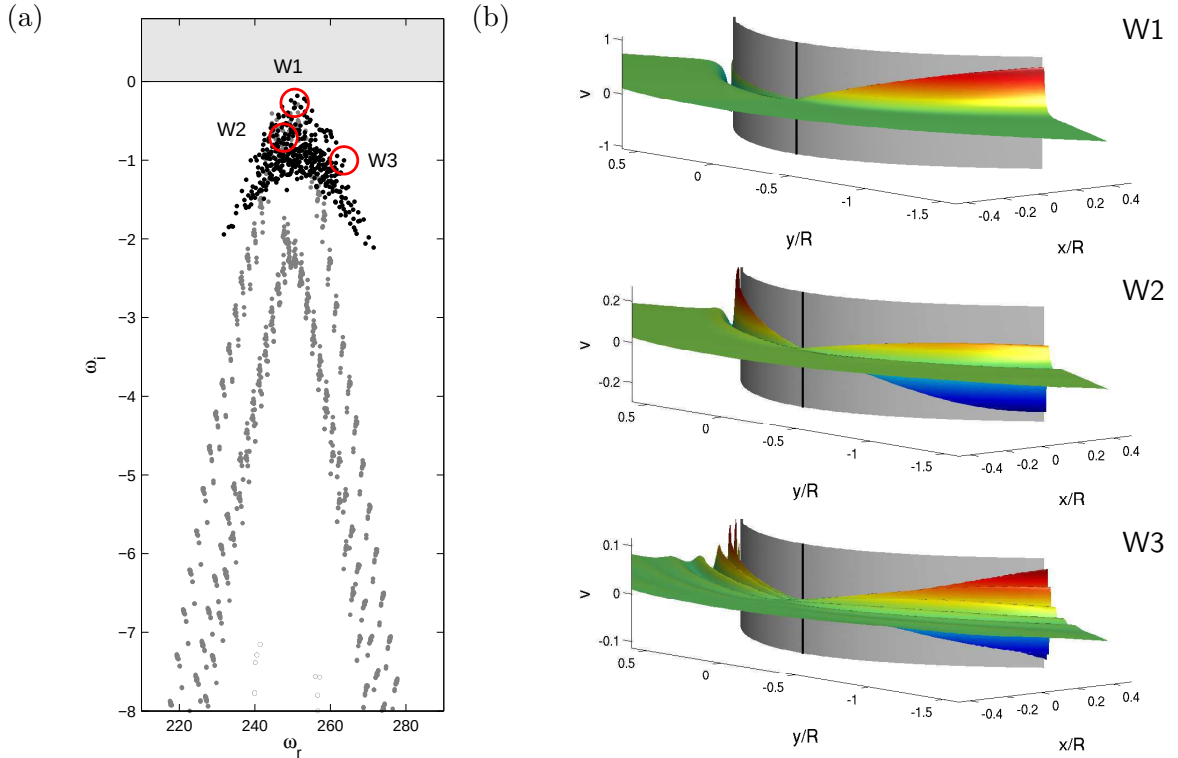
Figure 5.8. (a) Computed region of the global spectrum containing the eigenvalues belonging to wave packet modes (see region IV in figure 5.1). (b) Three representative wave packet modes (W1, W2 and W3) are visualized by the (normalized) chordwise velocity v ; attachment line in black.
