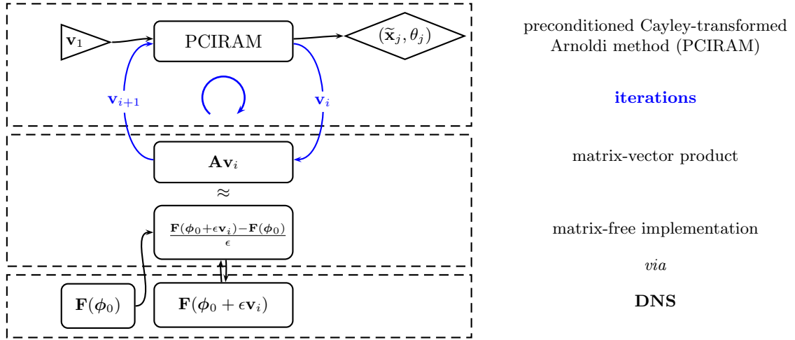
Figure 4.5. Sketch of a (compact) form of our proposed DNS-based global stability solver (abbreviated as PCIRAM) as presented in Mack and Schmid (2010). The dashed boxes represent different components of the algorithm which could be replaced in a modular manner, e.g., instead of direct numerical simulations (DNS), Large-Eddy simulations (LES) could be used to provide the required input for the matrix-free implementation.
