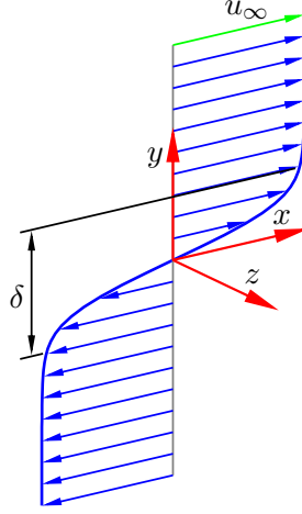
Figure 1. Sketch of a mixing layer showing the base velocity profile (in blue), some of the relevant flow parameters and the Cartesian coordinate system (in red).
