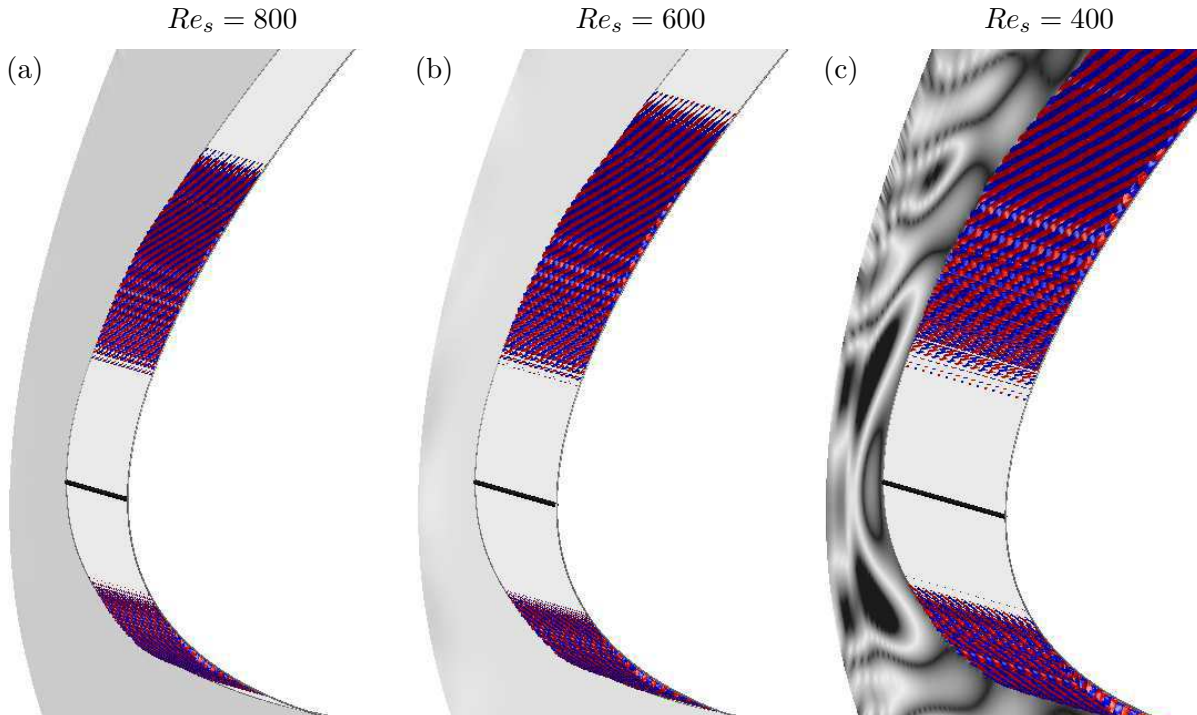
Figure 3. Spatial structure of a the most unstable boundary-layer modes (depicted by circles in figure 2a) visualized by iso-surfaces (positive values in red, negative values in blue) of the normal velocity v(x, y, z) = \text{Real}\{\tilde{v}(x, y) (\cos \beta z + i \sin \beta z)\} ; eight periods in z are shown; attachment line in black: (a) Re_s = 800 , (b) Re_s = 600 and (c) Re_s = 400 . Contours of the associated pressure field of each mode are displayed in the background.
