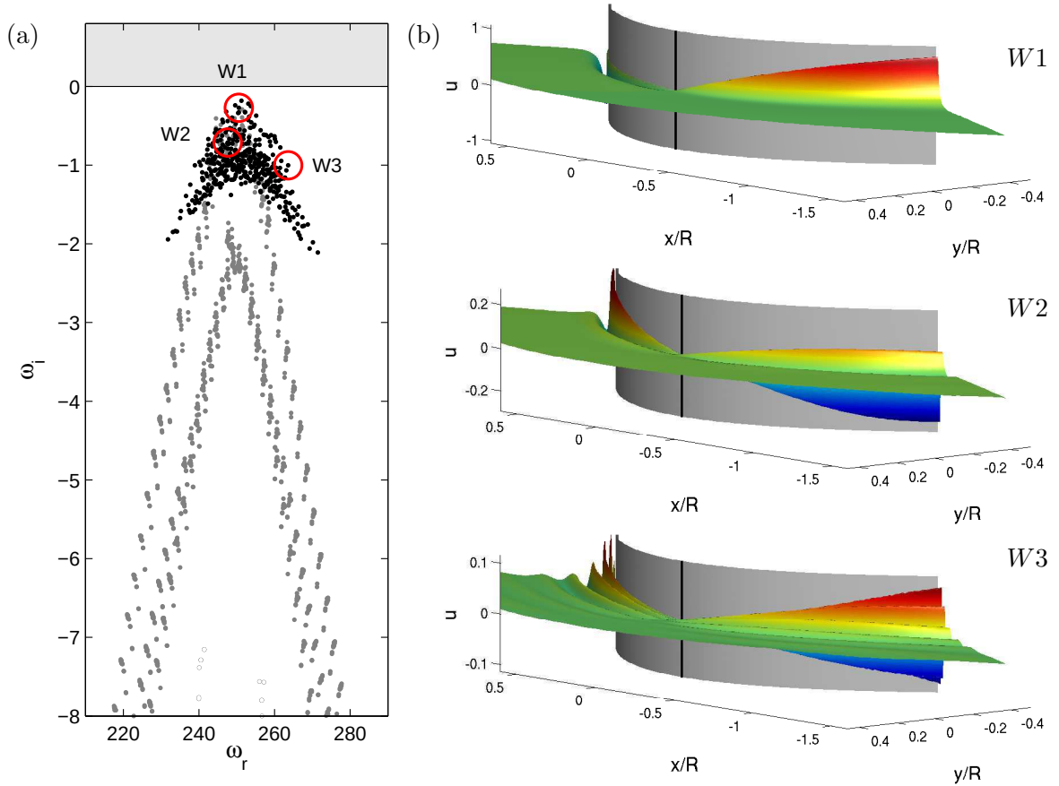
Figure 9. (a) Computed region of the global spectrum containing the eigenvalues belonging to wave packet modes (see region IV in figure 4). (b) Three representative wave packet modes (W1, W2 and W3) are visualized by the (normalized) chordwise velocity u ; attachment line in black.
