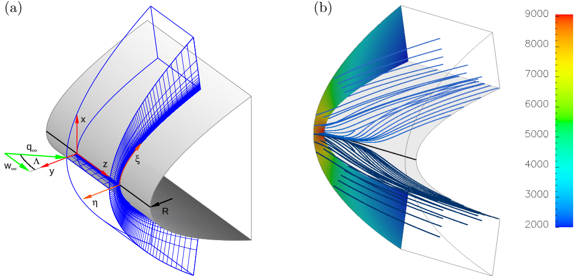
Figure 9. (a) Sketch of the three-dimensional flow configuration showing the relevant flow parameters, the used coordinate systems and the grid-point distribution. The quantities R , q_\infty , \Lambda and w_\infty denote respectively the leading-edge radius of the parabolic body, the freestream velocity, the sweep angle and the resulting sweep velocity. (b) Streamlines (in blue) and pressure field in [Pa] of the computed steady base flow for a sweep Reynolds number Re_s = w_\infty \delta / \nu_r = 800 and a sweep Mach number Ma_s = w_\infty / c_\infty = 1.25 . The resolution is 128 \times 255 points in the normal \eta -direction and the chordwise \xi -direction. The spanwise z -direction is assumed periodic.
