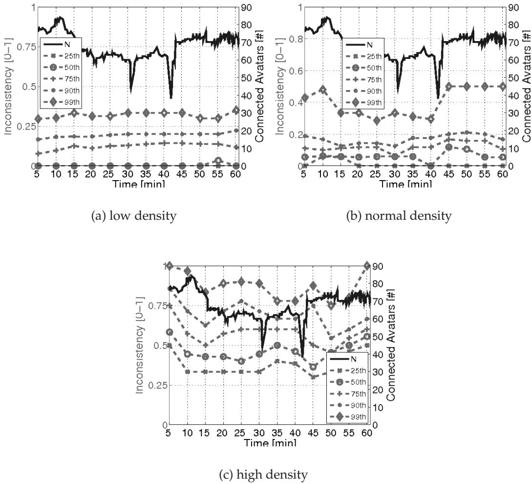
Figure 3.20: Percentiles of the avatar inconsistency over time.
