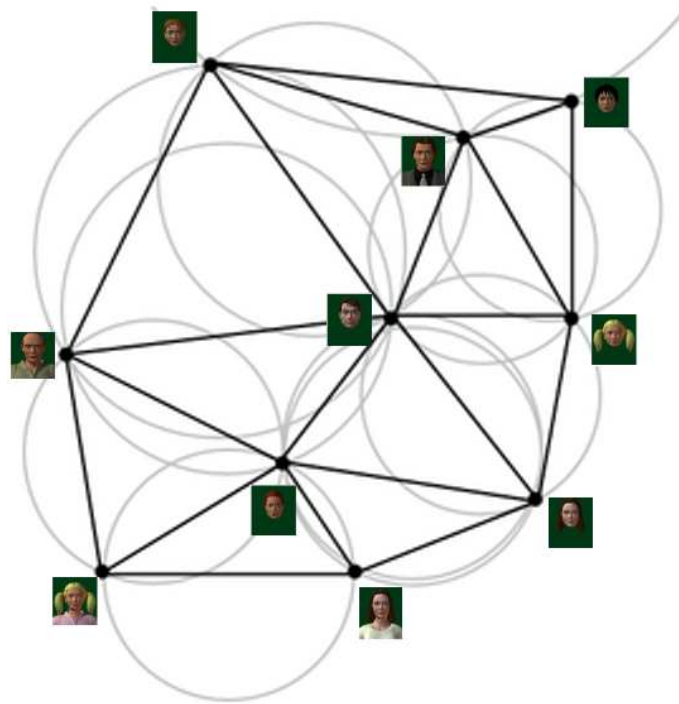
Figure 5.1: Distributed avatar management leveraging the Delaunay Network.
