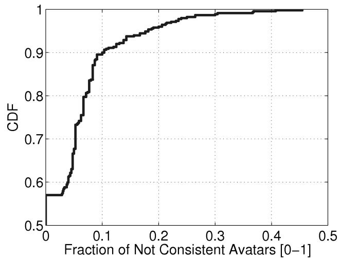
(b) CDF of the fraction of not consistent avatars ; AoI_r = 35 units.
