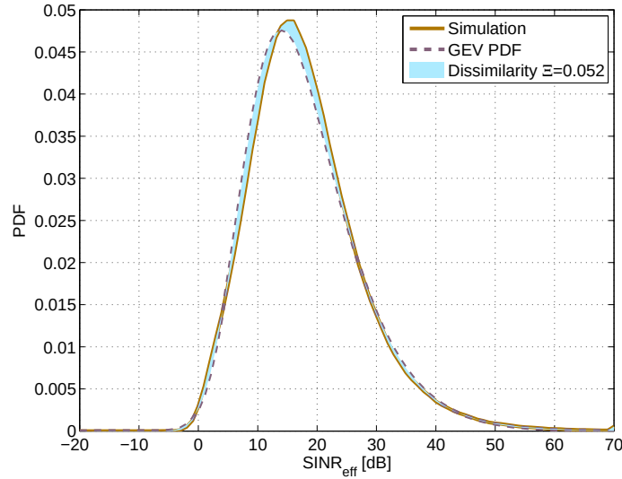
Figure 4.2: SINR_{eff} distribution through simulation and GEV parameters for \sigma_{SH} = 9 dB, R = 1500 m, P_{Tx} = 43 dBm and reuse 3x3x3.
