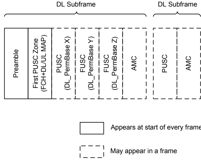
Figure A.2: Illustration of OFDMA frame with multiple zones (inspired from Fig. 219 of [26]).
