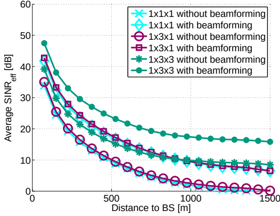
Figure 3.2: Average SINR_{eff} (DL) vs distance for reuse 1x1x1, 1x3x1 and 1x3x3 with beamfomorming.
