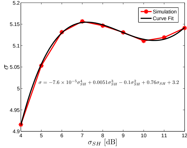
Figure B.3: Scale parameter \sigma of GEV distribution vs \sigma_{SH} for R = 1500 m, P_{Tx} = 43 dBm and reuse 1x1x1.
