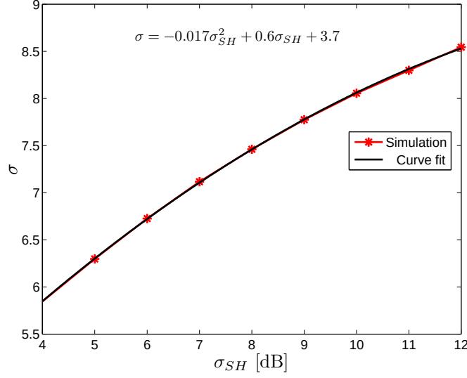
Figure 4.4: Scale parameter \sigma of GEV distribution vs \sigma_{SH} for R = 1500 m, P_{Tx} = 43 dBm and reuse 3x3x3.
