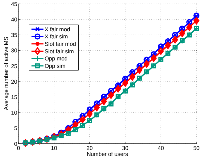
Figure 6.5: Average number of active MS for BE mono-profile with conventional scheduling schemes ( \bar{x}_{on} = 3 Mbits and \bar{t}_{off} = 3 s).
