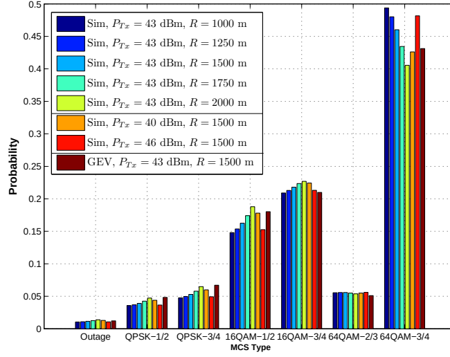
Figure 4.6: MCS probabilities for \sigma_{SH} = 7.5 dB and reuse 3x3x3.
