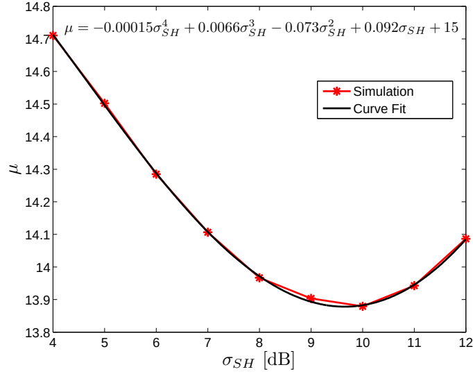
Figure 4.5: Location parameter \mu of GEV distribution vs \sigma_{SH} for R = 1500 m, P_{Tx} = 43 dBm and reuse 3x3x3.
