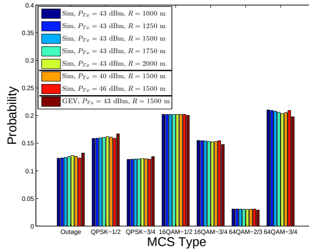
Figure B.20: MCS probabilities for \sigma_{SH} = 7.5 dB and reuse 3x1x1.
