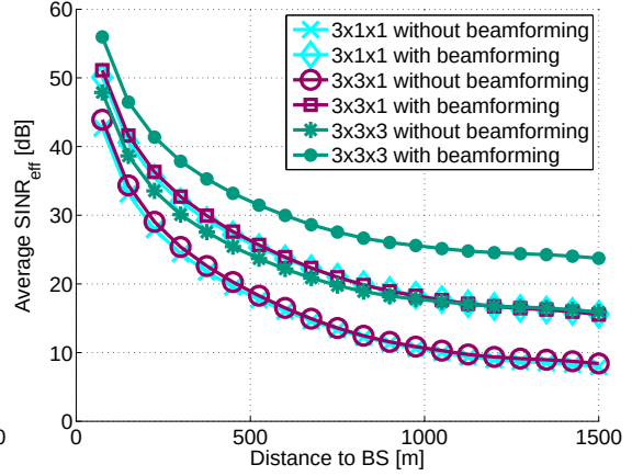
Figure 3.3: Average SINR_{eff} (DL) vs distance for reuse 3x1x1, 3x3x1 and 3x3x3 with beamfomorming.
