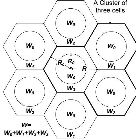
Figure 5.5: Fractional Frequency Reuse (FFR) case. Bandwidth W_0 is deployed with reuse 1 in the inner regions, while W_1 , W_2 and W_3 are deployed with reuse 3 in outer regions.
