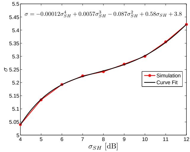
Figure B.8: Scale parameter \sigma of GEV distribution vs \sigma_{SH} for R = 1500 m, P_{Tx} = 43 dBm and reuse 1x3x1.
