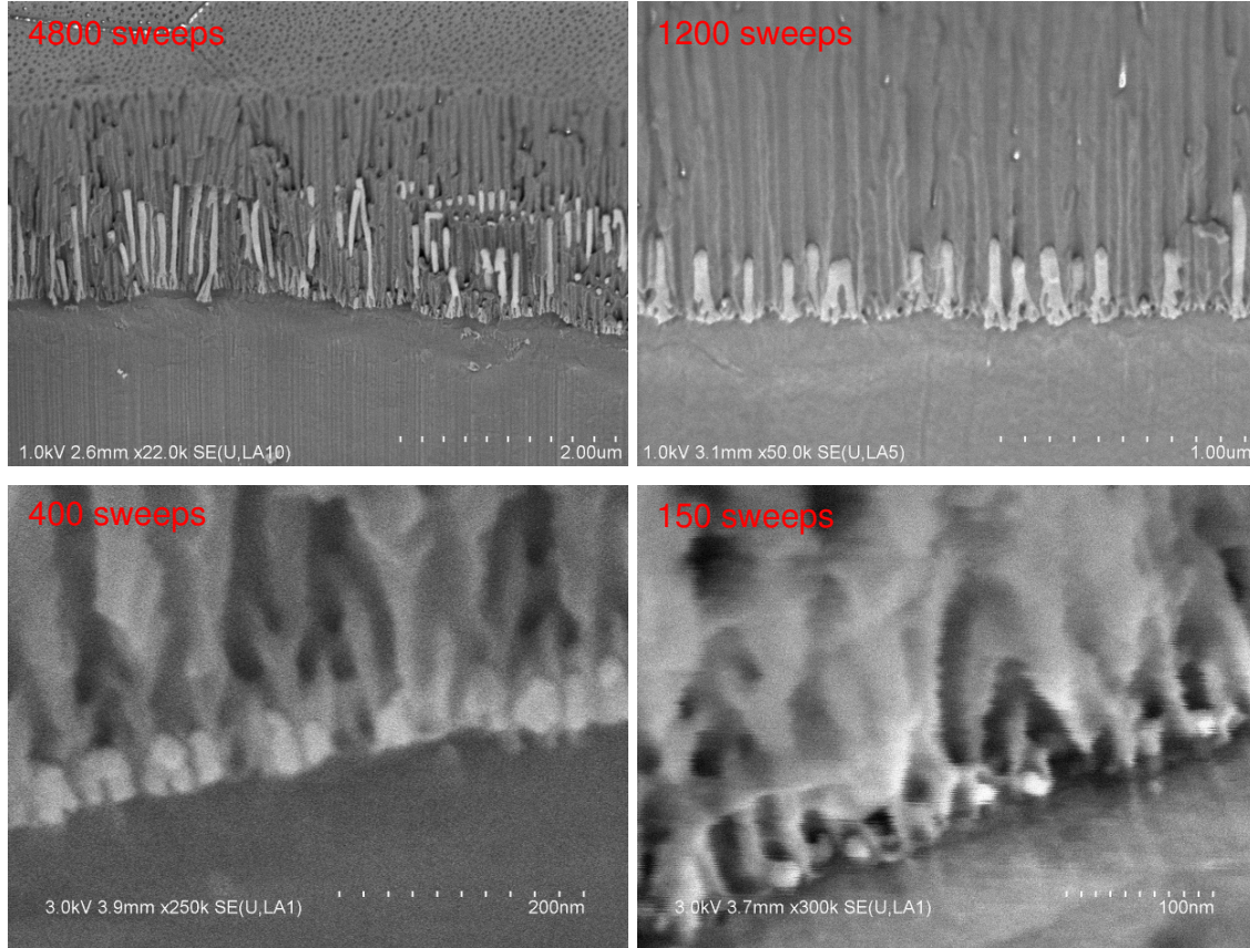
Fig. II.4: Variation of the number of sweeps of the electrodeposition at -4.2 V at about 1.1mA/cm^2 .
