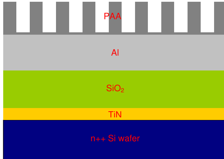
Fig. IV.12.: Multilayer stacking with PAA mask on top.
