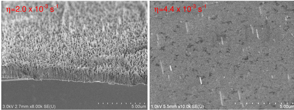
Fig. II.9: SEM image of 45 °tilted samples with deposited Ni-nanowires.
