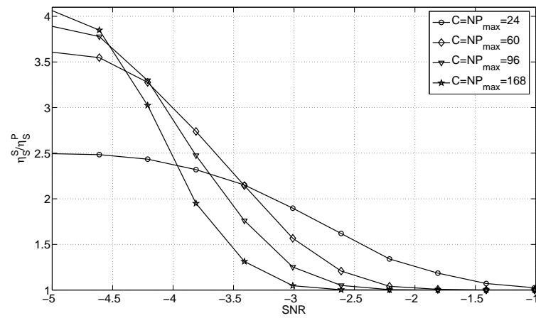
Figure 4.2: Ratio between the SBS efficiency and the PBS efficiency with respect to the SNR for IR-HARQ and different values of C . ( R_0 = 1/4 , L_F = 120 bits, and N = 3 .)
