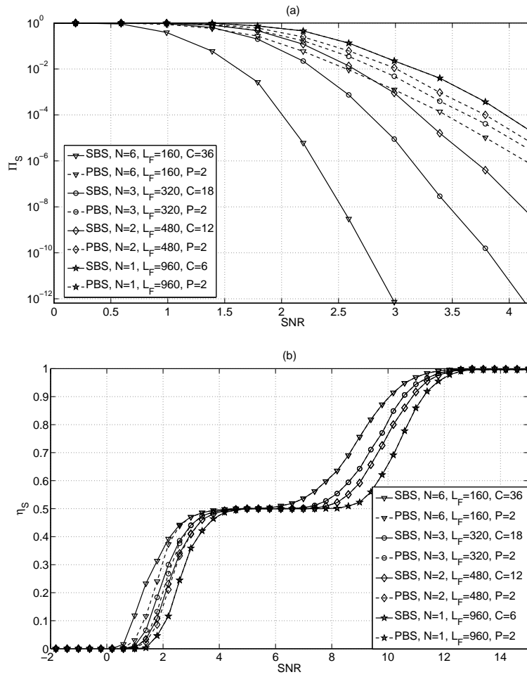
Figure 4.11: Theoretical PER (a) and efficiency (b) versus SNR for IR-HARQ mechanism, PBS and SBS contexts, and different N . ( L_{\text{DSDU}} = 960 bits, R_0 = 1/2 , and C/N = 6 .)
