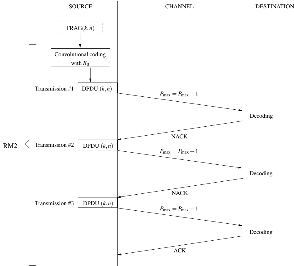
Figure 1.3: RM2 scheme (where P_{\max} \geq 3 ).
