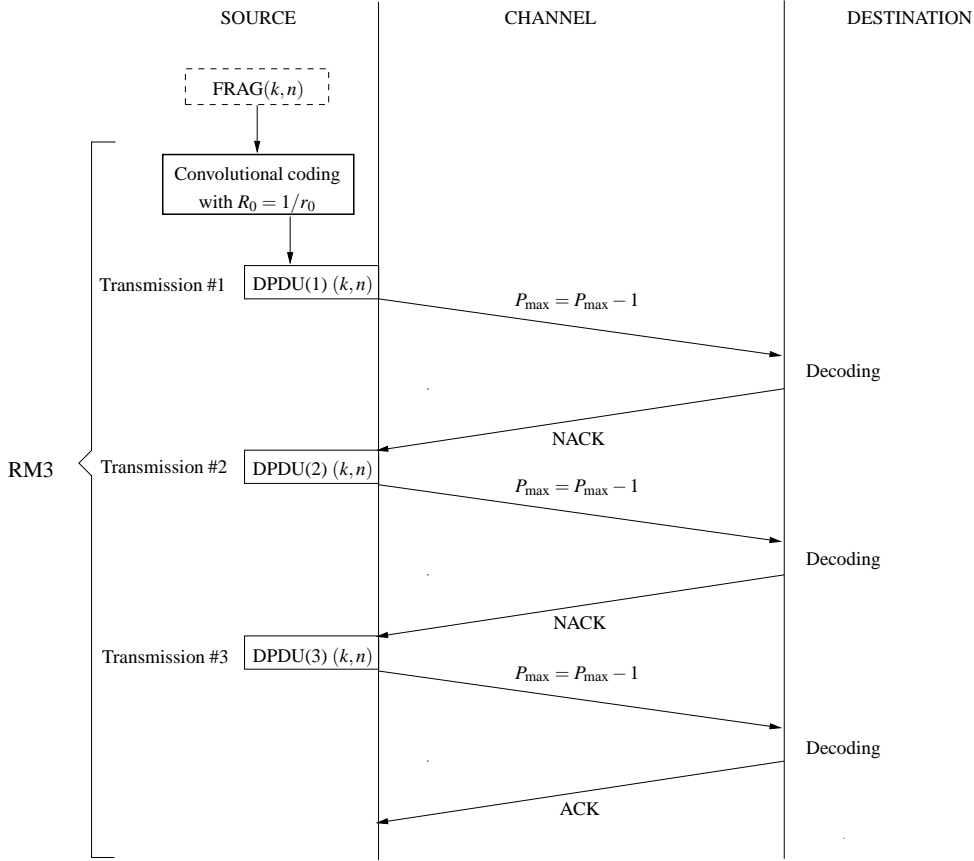
Figure 1.4: RM3 scheme (where P_{\max} \geq 3 and R_0 = 1/r_0 with r_0 \geq 3 ).
