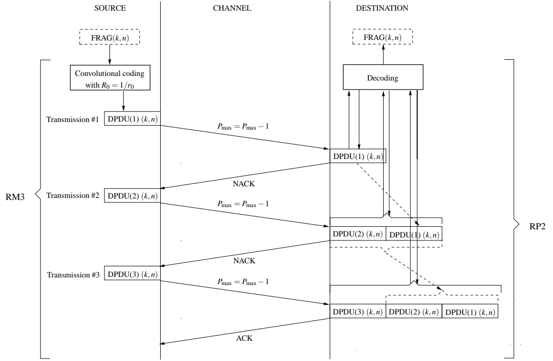
Figure 1.6: RP2 associated with RM3 (where P_{\max} \geq 3 and R_0 = 1/r_0 with r_0 \geq 3 ).
