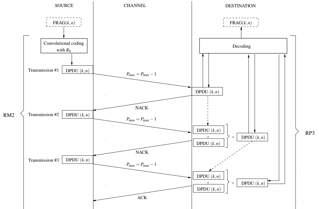
Figure 1.7: RP3 associated with RM2 (where P_{\max} \geq 3 ).
