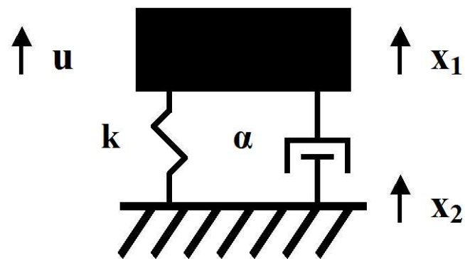
Figure 5.3: Simplified model of building undergoing an earthquake
