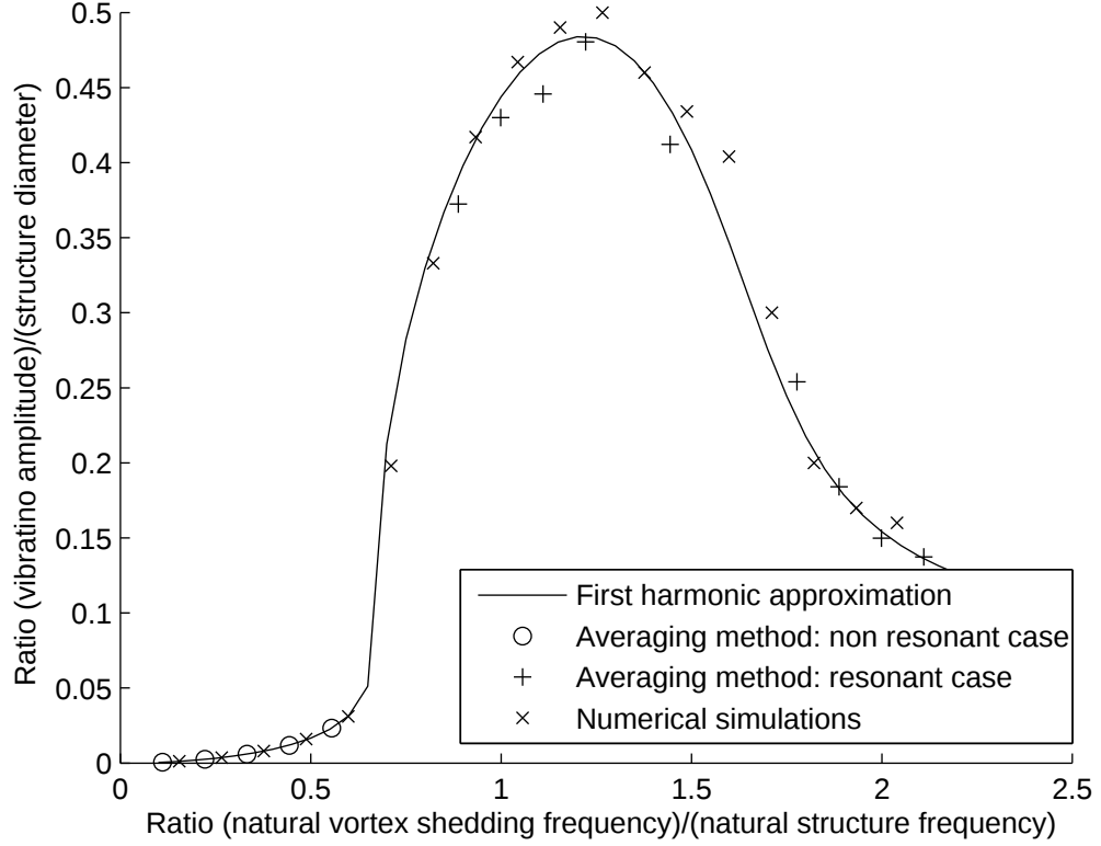
Figure 6.1: VIV amplitudes for different vortex shedding frequencies
