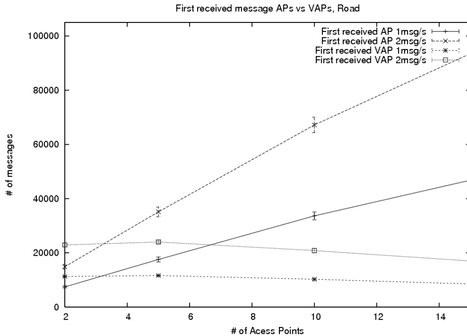
Figure 4.9: Number of messages first received from an AP and VAP
