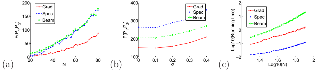
Figure 4.2: (a) F(P_1, P_2) (mean value over 30 repetitions) as a function of graph size N , simulation parameters: p = 0.1, \sigma = 0.05, M = 3 . (b) F(P_1, P_2) (mean value over 30 repetitions) as a function of noise parameter \sigma , simulation parameters: N = 30, p = 0.1, M = 3 . (c) Algorithm running time (mean value over 30 repetitions) as a function of N (log-log scale), other parameters are the same as in (a).
