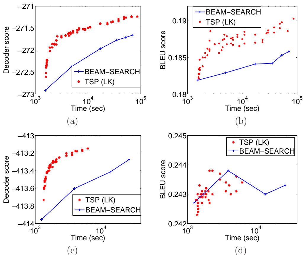
Figure 5.6: (a), (b): Europarl corpus, translation from English to French; (c),(d): NewsCommentary corpus, translation from German to Spanish. Average value of the decoder and the BLEU scores (over 500 test sentences) as a function of time. The trade-off quality/time in the case of LK is controlled by the number of iterations, and each point corresponds to a particular number of iterations, in our experiments LK was run with a number of iterations varying between 2k and 170k. The same trade-off in the case of Beam-Search is controlled by varying the beam thresholds.
