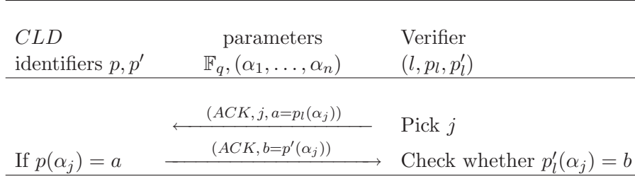
Figure X.1: CLD identification via Moulin-Koetter identification codes
