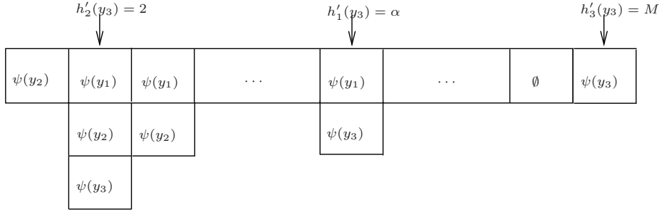
Figure V.1: Construction of Bloom Filters with Storage
