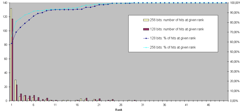
Figure VII.2: Accuracy with 128 bits and 256 bits
