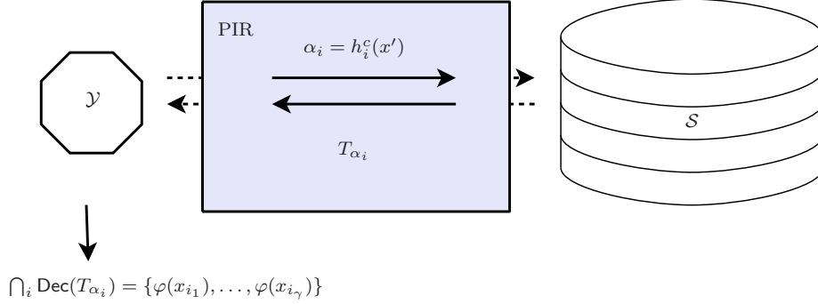
Figure V.3: Retrieving data in a nutshell
