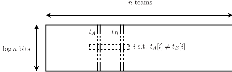
Figure IX.1: Lossless representation of n teams, and resulting two-way communication
