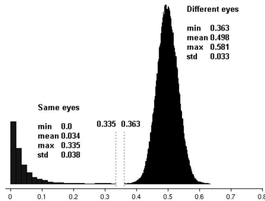
Figure IV.1: Hamming distance distributions from [87]
