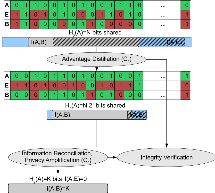
Figure D.2: The global scheme, illustrated
