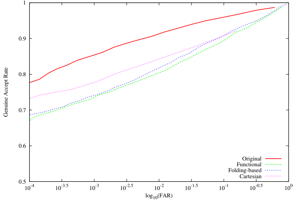
Figure III.4: Detection Error Trade-off curves for experiments on FVC 2000 Db1
