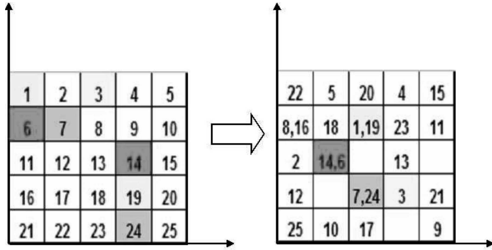
Figure III.1: Cartesian transformation from [147]
