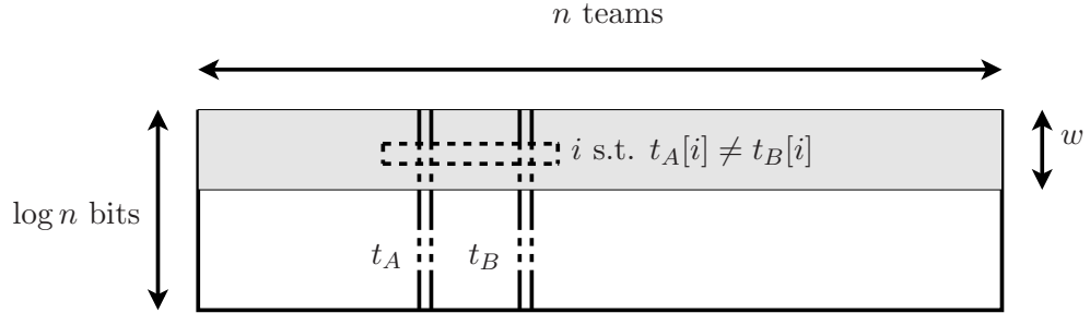
Figure IX.2: Representation of n teams on w < \log n bits.
