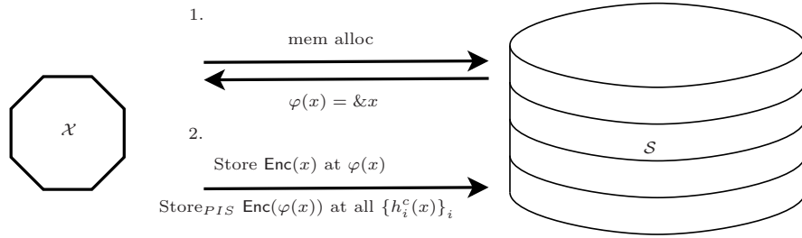
Figure V.2: Sending a message in a nutshell
