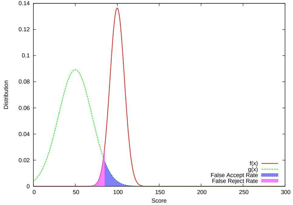
Figure II.1: Illustration of the score distributions for matching and non-matching pairs. The error rates (here FAR = FRR = 4\% ) are the filled areas.
