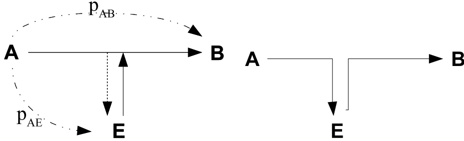
Figure D.1: The noisy channels C_{p_{AB}} , C_{p_{AE}} , and the noiseless channel C_0 .
