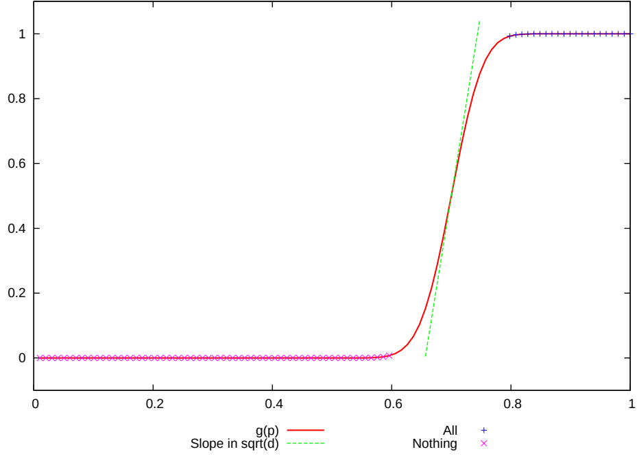
Figure X.2: Illustration of the threshold effect, d = 400 , p_c = 0.7
