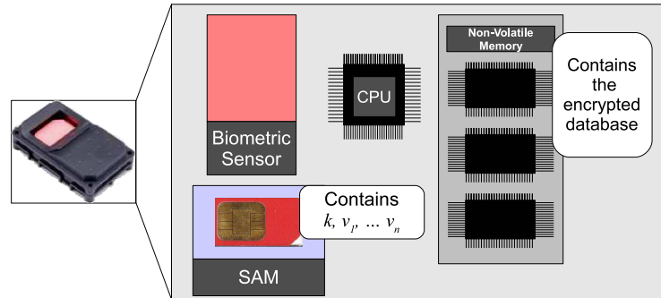
Figure VII.1: Our Biometric Terminal
