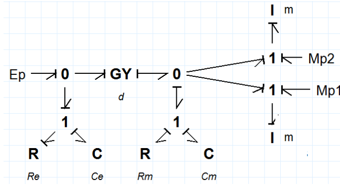
Figure 4.13: Damped model
