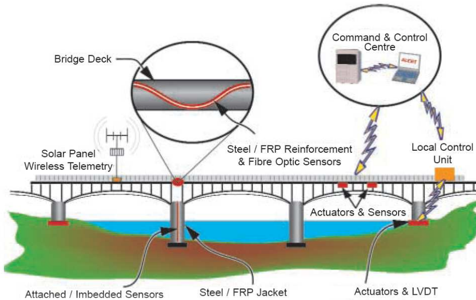
Figure 2.2: Schematic example of a smart bridge [8]
