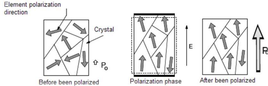
Figure 2.10: Poling process
