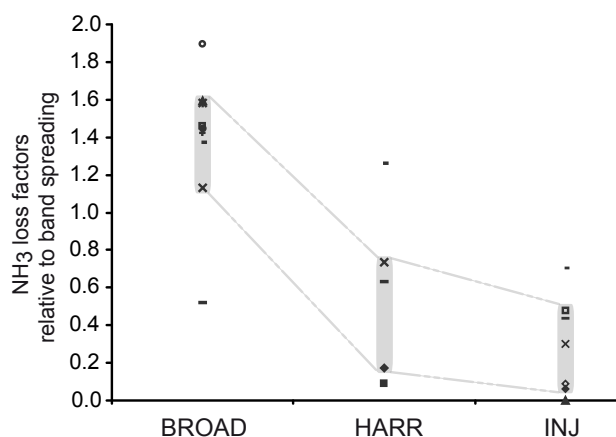
FIGURE 2.3 – Distribution of the relative N loss factors k_{\text{NH}_3, \text{Tech}} for broadcast, harrowing and injection application techniques
