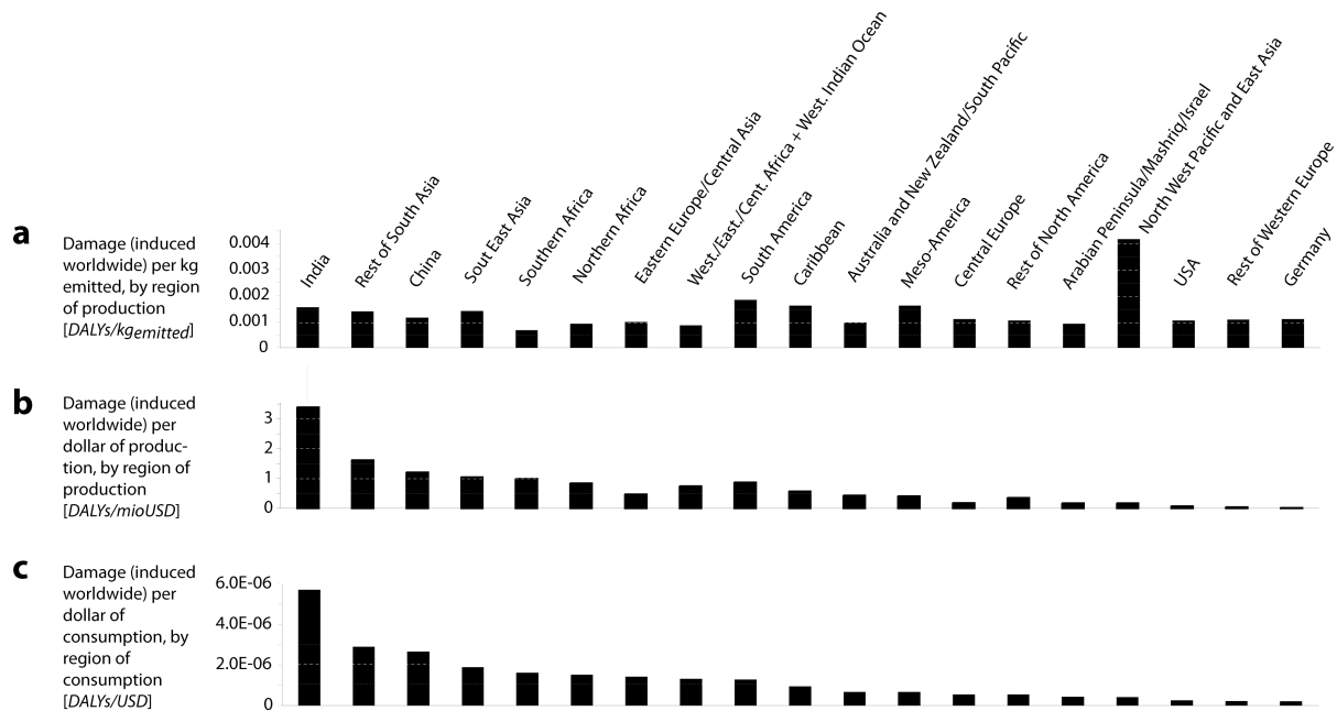
Supplementary Figure S3 Damage factors per kilogram emitted, per dollar of production and per dollar of consumption in each region.
