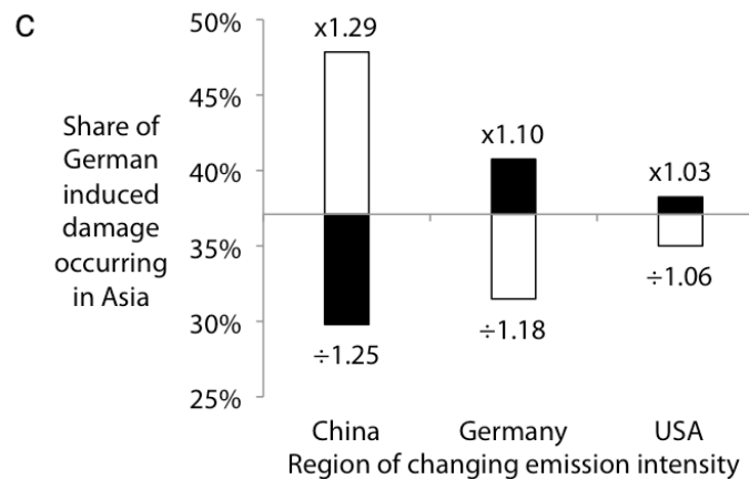
Supplementary Figure S4. Sensitivity studies of various output parameters in the impact model to key input parameters in the multi-regional Input-Output model. Output parameters examined are (a) change in global human health impacts (due to PM 2.5 emissions to meet global final demand), (b) change in share of global induced impacts occurring in Asia (China, South Asia, and South East Asia), and (c) change in share of German-induced impacts occurring in Asia. Bars represent changes due to multiplying by two (white bars) or dividing by two (black bars) the emissions per dollar for the region
