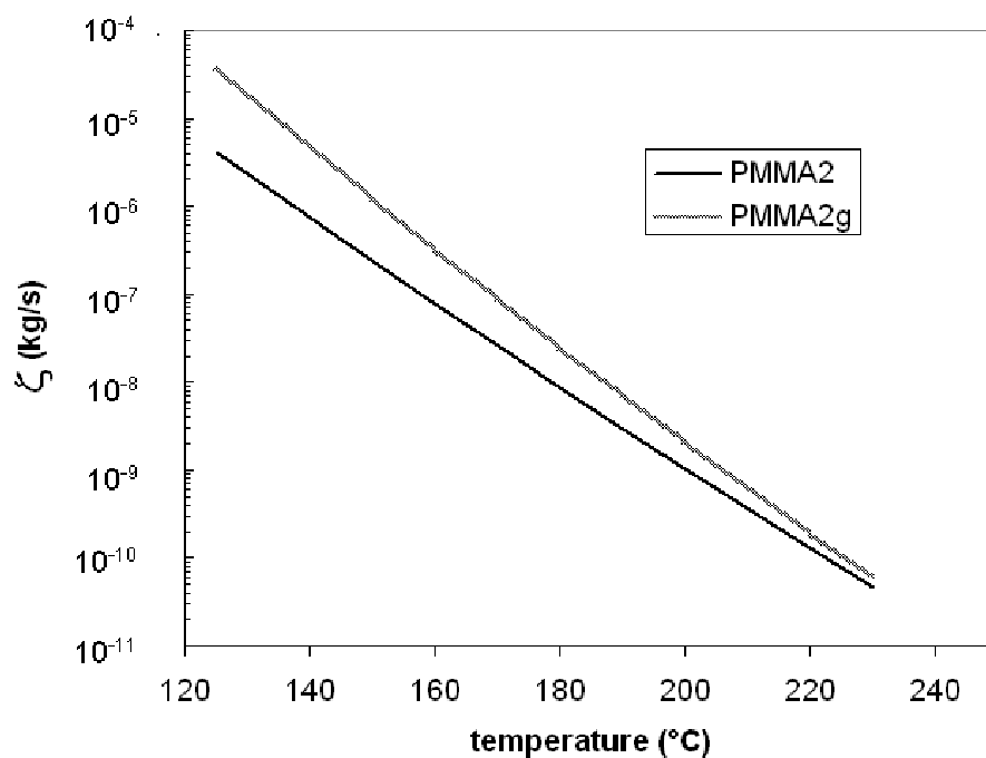
Figure 57 Comparison of the evolution of the friction coefficient \zeta with temperature for PMMA2 and PMMA2g
