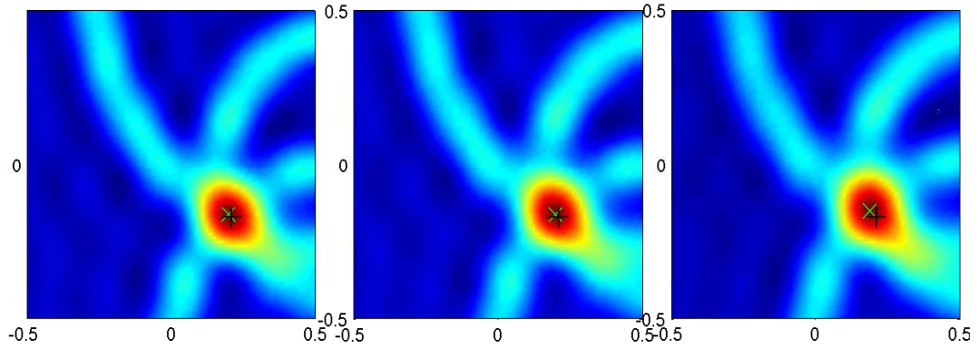
FIGURE 3.13. Kirchhoff results for the geometry sqReg2 with perturbed boundary (from left-to-right, \epsilon = 0.01, 0.025 and 0.05 ). The (black/white) x denotes the (numerical/theoretical) center of the source.
