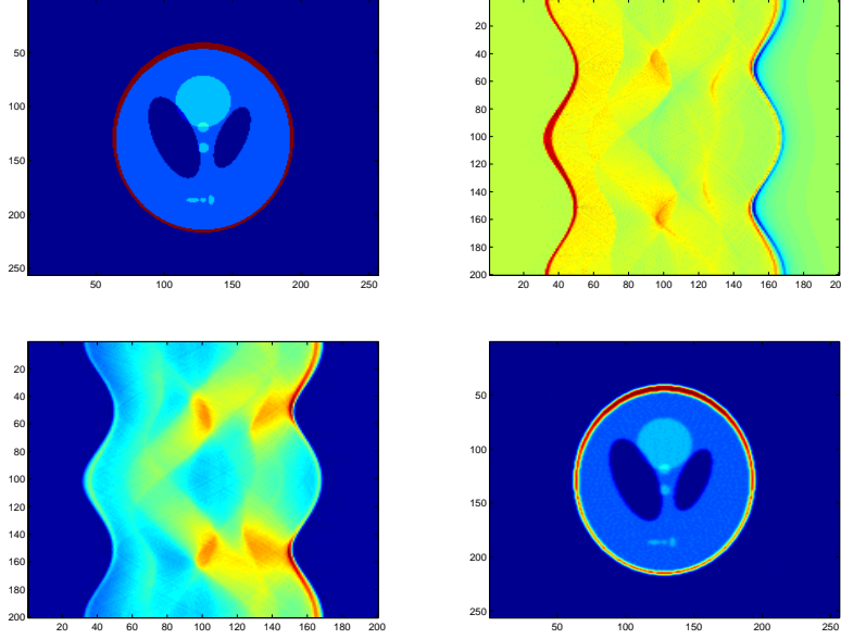
FIGURE 4.1. Numerical inversion using (4.3) with N = 256 , N_R = 200 and N_\theta = 200 . Top left: p_0 ; Top right: p(y, t) with (y, t) \in \partial\Omega \times (0, 2) ; Bottom left: \mathcal{R}_\Omega[p_0](y, t) with (y, t) \in \partial\Omega \times (0, 2) ; Bottom right: \frac{1}{4\pi^2}\mathcal{R}_\Omega^*\mathcal{B}\mathcal{R}_\Omega[p_0] .
