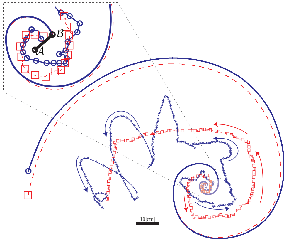
Figure 2.5: Tool Trajectories and its respective resultant crack paths.
