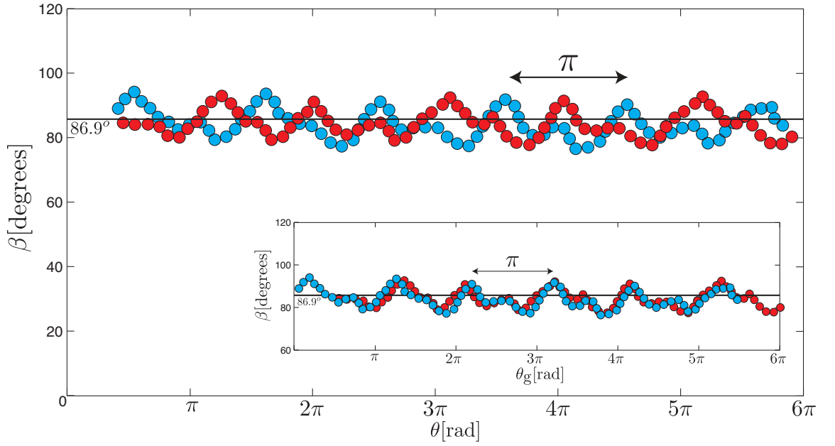
Figure 3.6: Measurements of \beta as a function of the spiral angle. Inset The same data presented as a function of the absolute orientation in the film.
