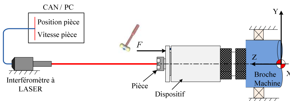
Figure 2.31: Configuration des tests impulsionnels.
