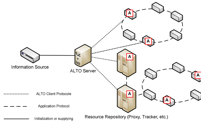
Figure 5.1: ALTO architecture
