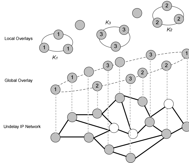
Figure 5.6: Context-Aware DHT model
