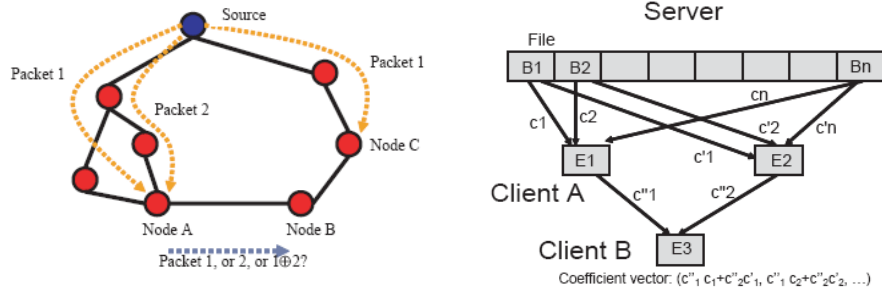
Figure 4.3: Network Coding (Figure from [GKA&al05])
