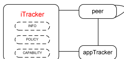
Figure 5.2: iTracker interface in P4P
