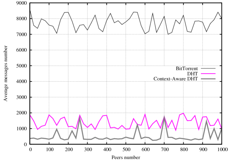
Figure 5.7: Average message number comparison between BitTorrent, generic DHT algorithm and Context-Aware DHT
