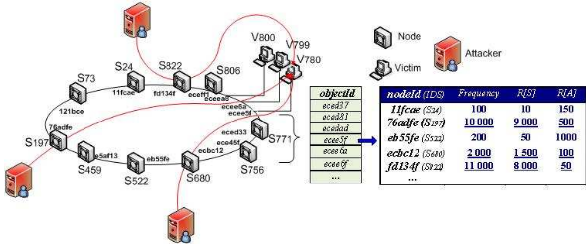
Figure 6.3: Nodes distribution and indexing with Pastry protocol
