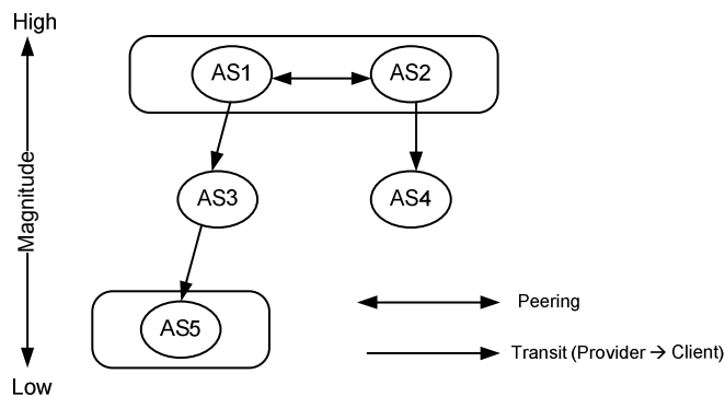
Figure 3.2: Valley-Free Path topology and AS magnitude in AURORA
