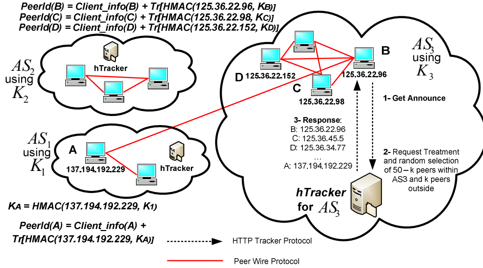
Figure 3.5: bTracker policy scenario example
