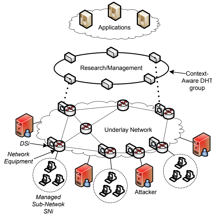
Figure 6.2: The architecture entities
