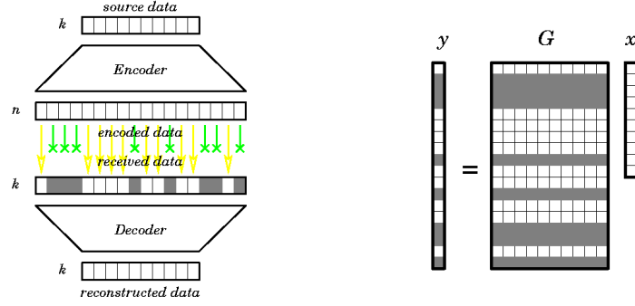
Figure 4.1: GF Matrix in FEC
