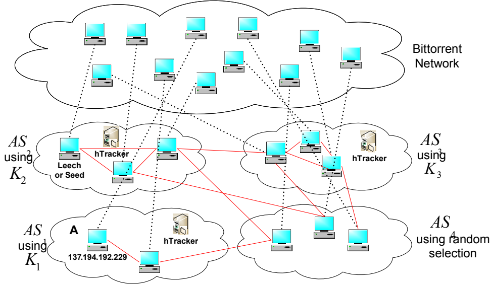
Figure 3.3: Graph representing an example of a 4 ASs BitTorrent Network including 3 ASs using hTracker solution and one generic AS.
