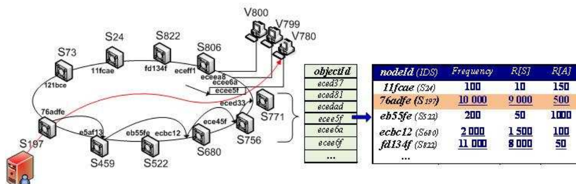
Figure 6.4: Lookup for V780's IDS from IDS S197
