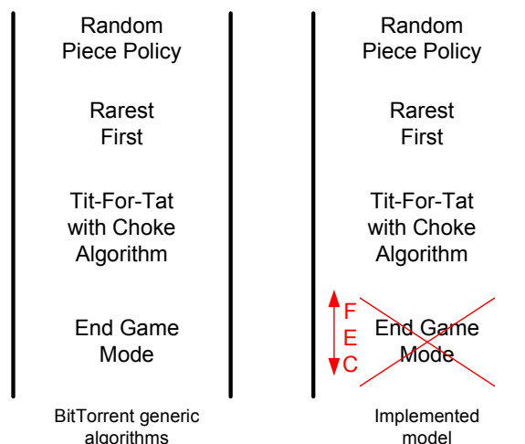
Figure 4.2: FEC at the end
