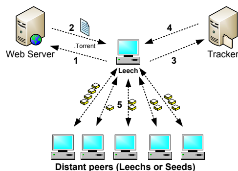
Figure 2.6: BitTorrent Architecture entities
