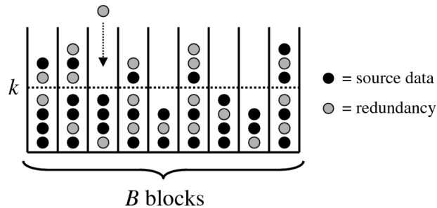
Figure 4.4: Digital Fountain mechanism (Figure from [BYE&al98])
