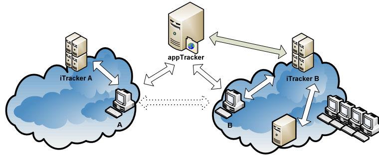
Figure 5.3: P4P architecture
