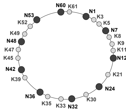
Figure 2.4: Chord algorithm
