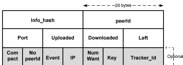
Figure 2.9: Get announce message
