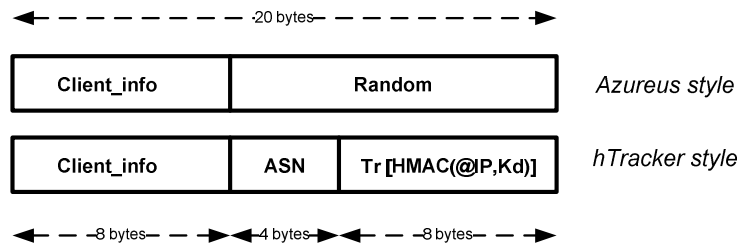
Figure 3.4: hTracker peerId specification
