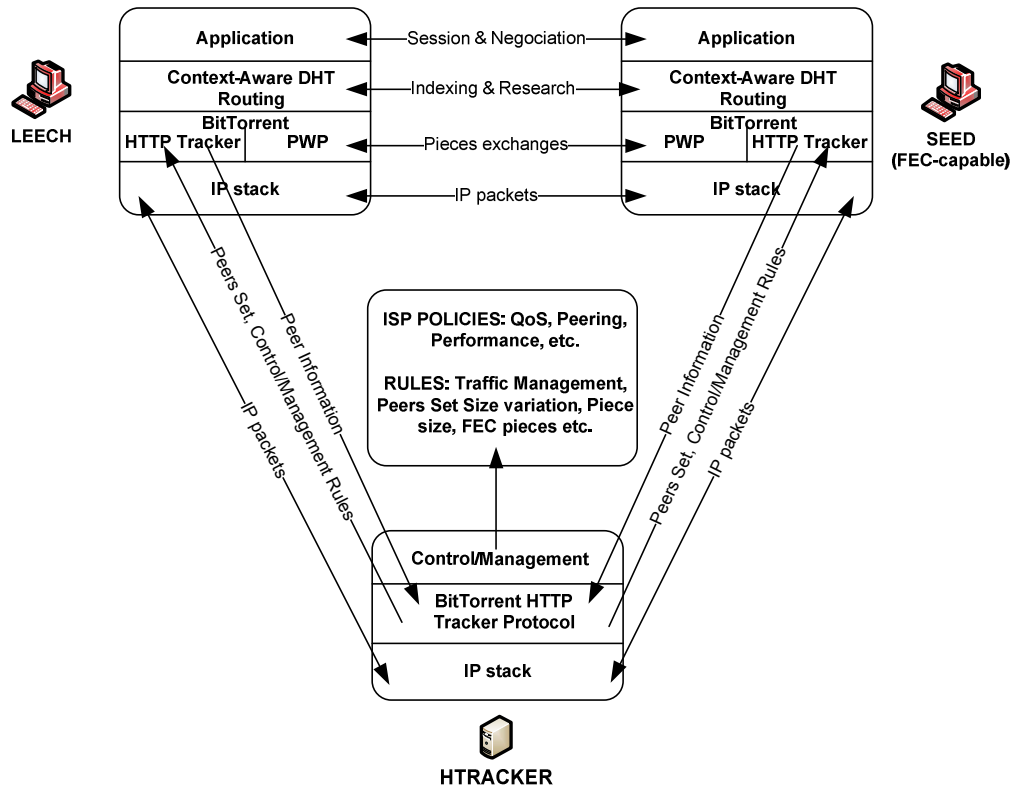
Figure 5.5: SPOP entities
