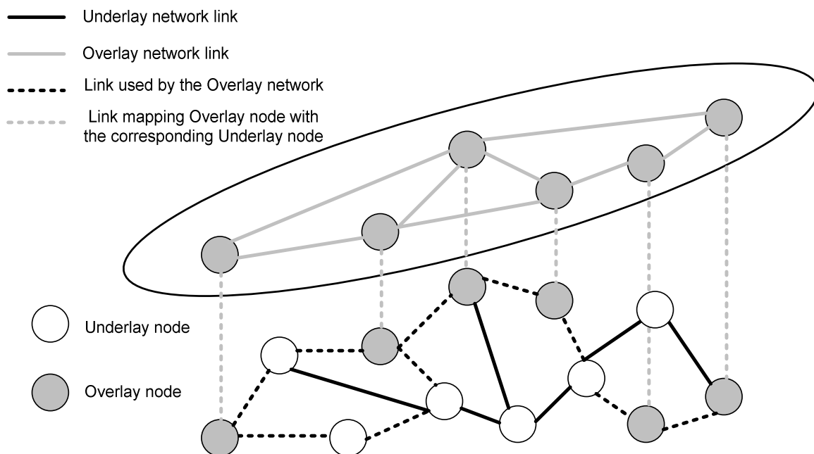
Figure 2.1: Overlay network
