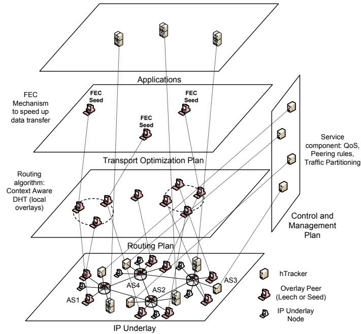
Figure 5.4: SPOP architecture
