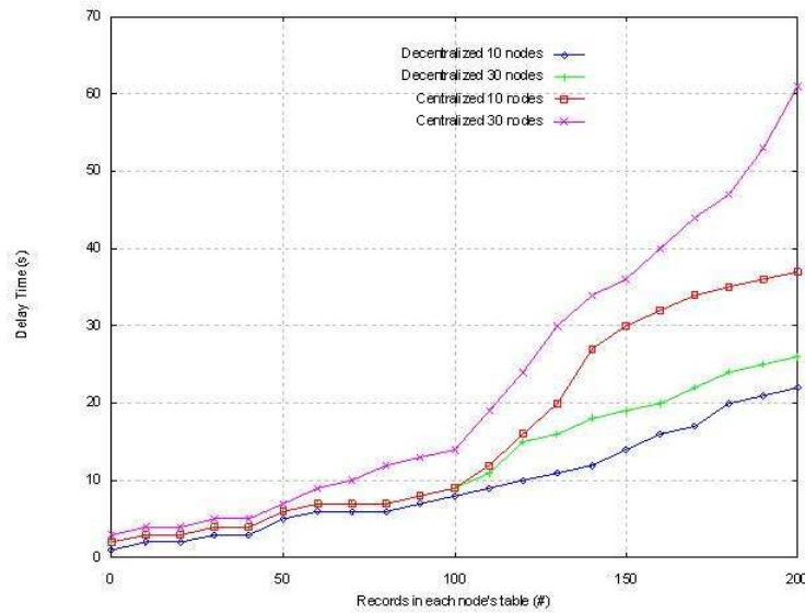
Figure 6.6: Comparison of the architecture with a centralized approach
