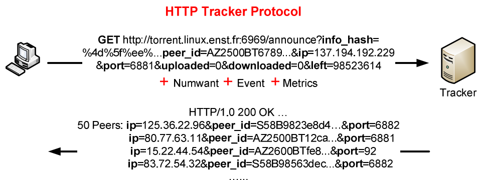
Figure 3.1: First exchange between a Leech and a Tracker
