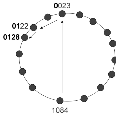
Figure 2.5: Pastry algorithm
