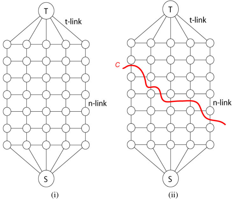
Figure 1.6: Example of a graph. (i) the graph G = (\mathcal{V}, \mathcal{E}) , (ii) an example of cut. C a cut partitioning the set of nodes \mathcal{E} in two subset S and T , containing respectively the source s and the sink t .
