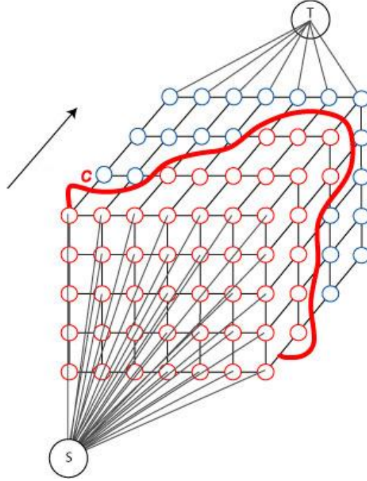
Figure 1.8: Example of a 3D graph for a stereo-matching problem. The arrow represents the direction of the increasing disparity, and C represent the cut partitioning the set of edges \mathcal{E} in two sub-sets S and T .
