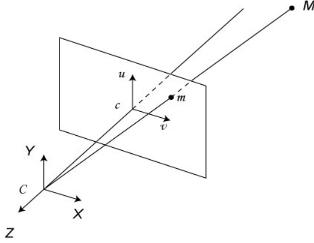
Figure 1.3: 3D Geometry in the case of one camera. The axes X , Y and Z , and the center C form the camera coordinates system while u , v and c form the image coordinates system. M is a given 3D point and m is its projection on the image according to m = PM where P is the projection matrix, associated to the camera.
