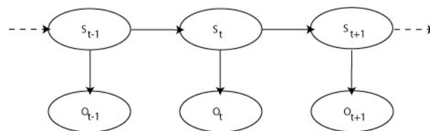
Figure 3.13: Modelisation of the Hidden Markov Model where S_t are the hidden parameter at time t and O_t the observation at time t .
