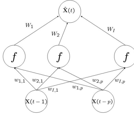
Figure 3.7: Neural network modeling the non-linear auto regressive process. The neural network is fed by the 3D coordinates of feature points from time t - 1 to t - p to estimate \hat{\mathbf{X}}(t) the 3D coordinates of feature points at time t .
