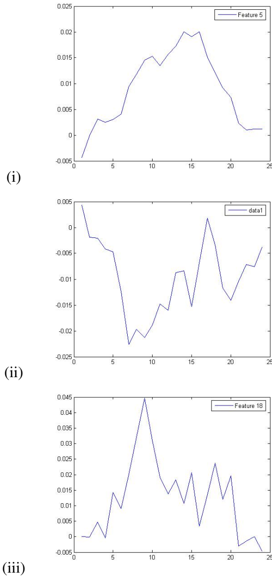
Figure 3.8: Graphs presenting the non-linearity of features displacements during an expression : (i) Vertical displacement of an inner eyebrow when expressing anger, (ii) Vertical displacement of a mouth's corner when expressing joy and (iii) Vertical displacement of lower lip's mid-point when expressing surprise. (One should note that the origin of the system of coordinates is at the top left corner of the image)
