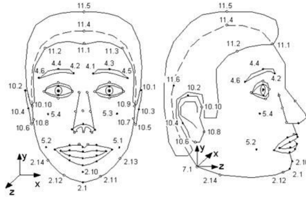
Figure 3.2: The 84 Features Points of the MPEG-4 standard for animation.
