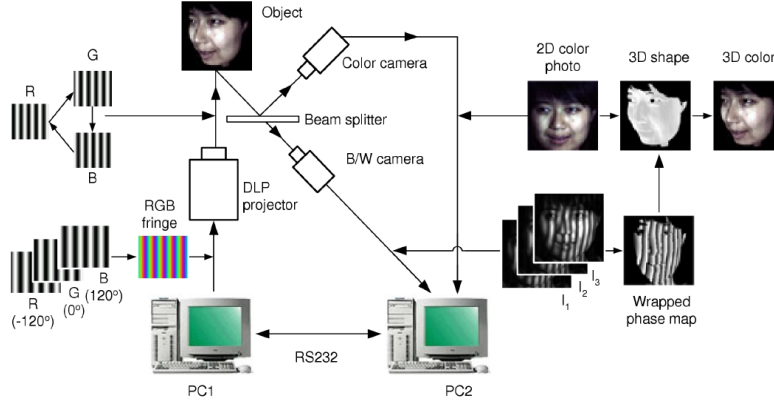
Figure 1.2: Structured light projection scheme proposed in [53].
