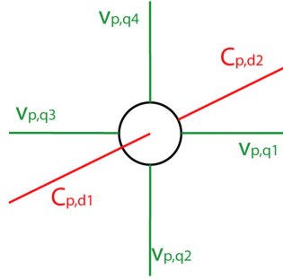
Figure 1.7: Six-connected vertex, in the case of stereo matching. In red, connections corresponding to the data term. In green, connections corresponding to the smoothness term.
