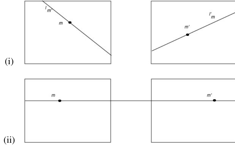
Figure 1.5: An example of images rectification : (i) The original images, (ii) the rectified images. m and m' are two corresponding points of coordinates (x, y)^T and (x', y')^T in the original images (i). The rectified images (ii) are wrapped such that m and m' coordinates become (x_r, y_r)^T and (x_r + d, y_r)^T where d is the corresponding disparity.
