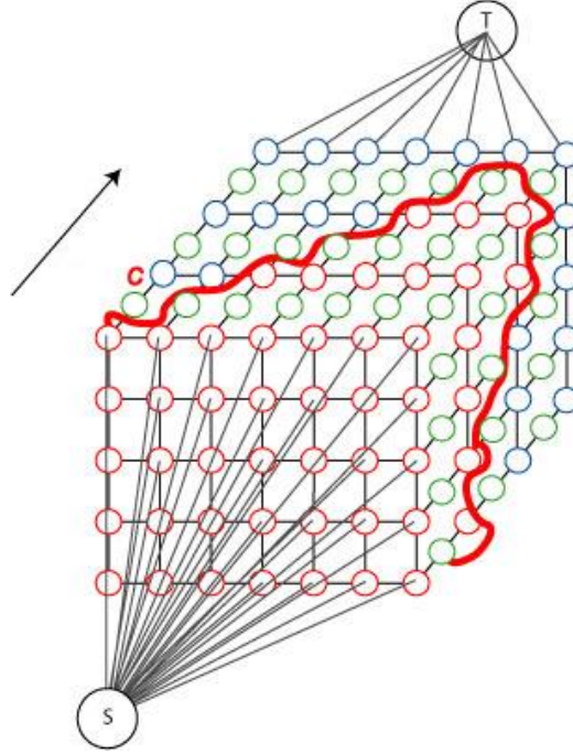
Figure 1.9: Example of a 3D graph for a stereo-matching problem using Super Resolution. The green nodes correspond to the added nodes between each existing nodes, and decreasing the disparity discretization to a half pixel.
