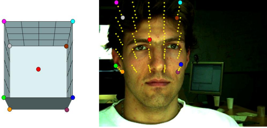
Figure 2.8: Projection of the 3D Grid on the image for one feature. The red dot refers to the current position of the considered control point and to the null translation label. The yellow dots represent the N^3 projections of considered candidates for a control point. This grid is refined in a coarse to fine approach.
