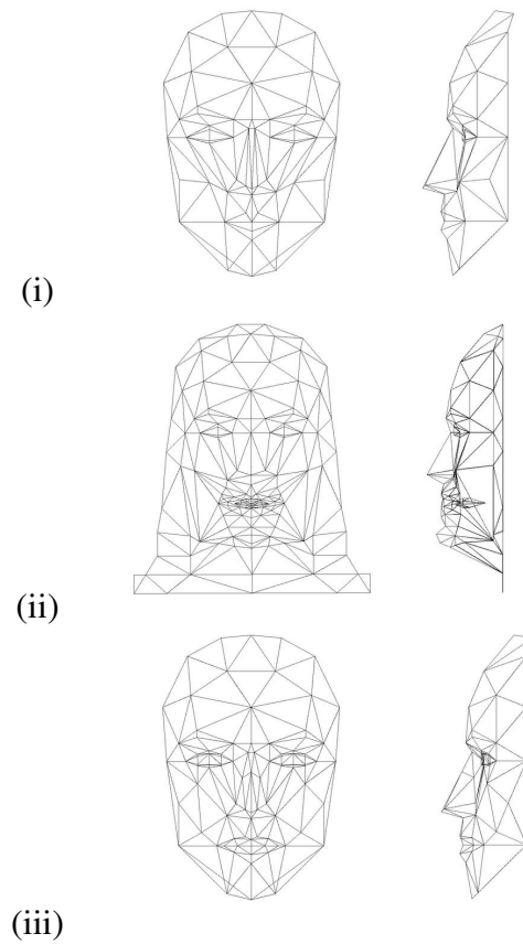
Figure 1.12: Evolution of the Candide Model. (i) The original Candide created in 1987 by Rydfalk. (ii) The second version of the Candide model by Bill Welsh in 1991 at British Telecom. (iii) The third version of the Candide model, developed by Jörgen Ahlberg in 2001 to simplify animation.
