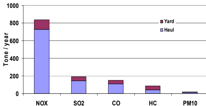
Figure 2.5: Pollutant emissions for rail road mobile sources.
