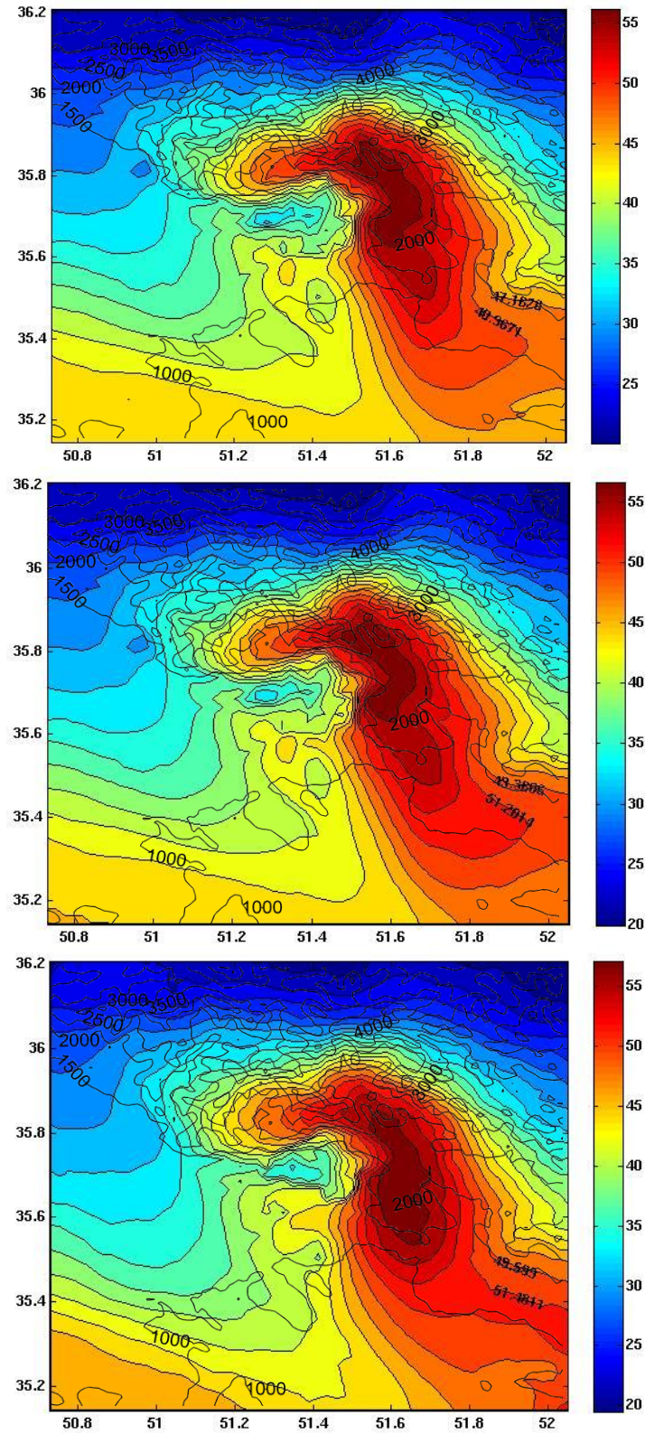
Figure 4.11 : O 3 concentration ( \mu\text{g}\cdot\text{m}^{-3} ) simulated by POLYPHEMUS with meteorological fields simulated by DA-SM2-U Q f : on (Run 1: top), DA-SM2-U Q f : off (Run 2: middle) and RA-SLAB (Run 3: bottom) at 10 m AGL, at 12 midday December 6 2005.
