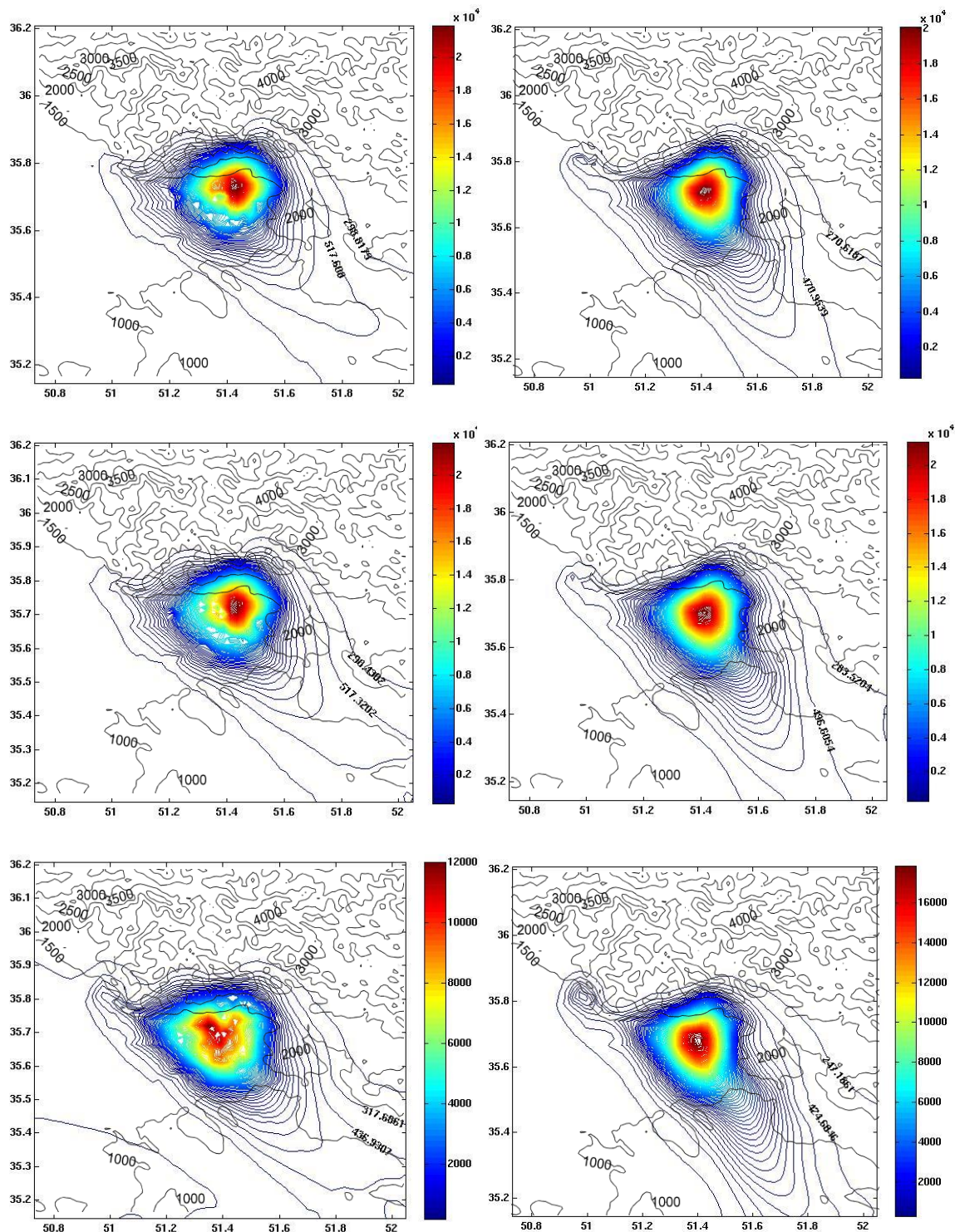
Figure 4.5: CO concentration ( \mu\text{g}\cdot\text{m}^{-3} ) simulated by POLYPHEMUS with meteorological fields simulated by DA-SM2-U Q f : on (Run 1: top), DA-SM2-U Q f : off (Run 2: middle) and RA-SLAB (Run 3: bottom) at 10 m AGL, at 10 am (left) and 10 pm (right) December 6 2005.
