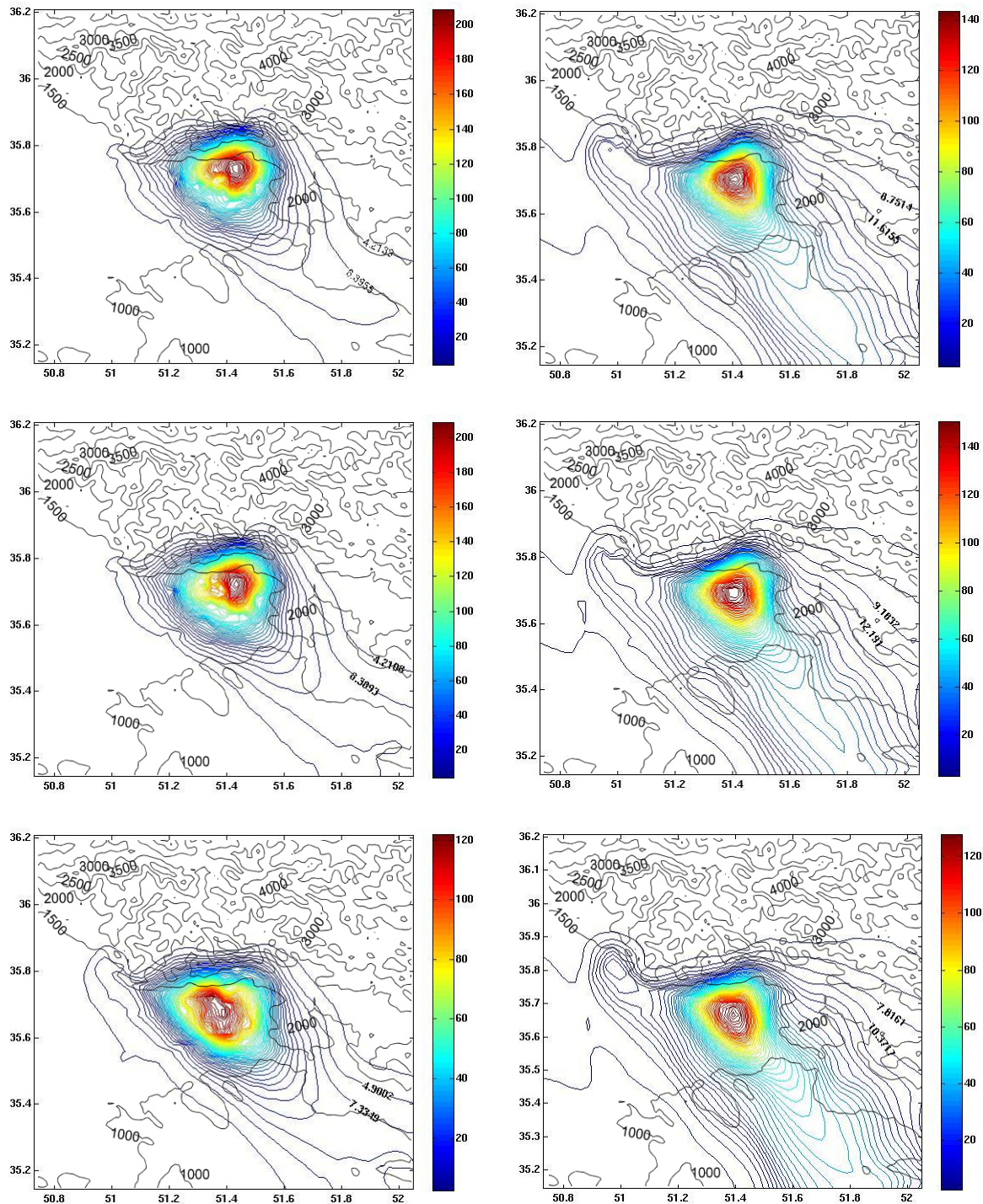
Figure 4.7 : NO 2 concentration ( \mu\text{g}\cdot\text{m}^{-3} ) simulated by POLYPHEMUS with meteorological fields simulated by DA-SM2-U Q f : on (Run 1: top), DA-SM2-U Q f : off (Run 2: middle) and RA-SLAB (Run 3: bottom) at 10 m AGL, at 10 am (left) and 10 pm (right) December 6 2005.
