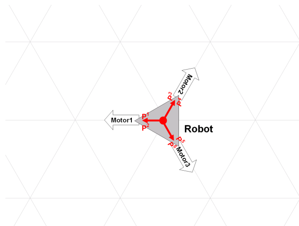
Figure 8.3: Definition of moving directions with respect to the nearest pattern during motion phase. The side length of the triangular lattice corresponds to the moving speed v_M .
