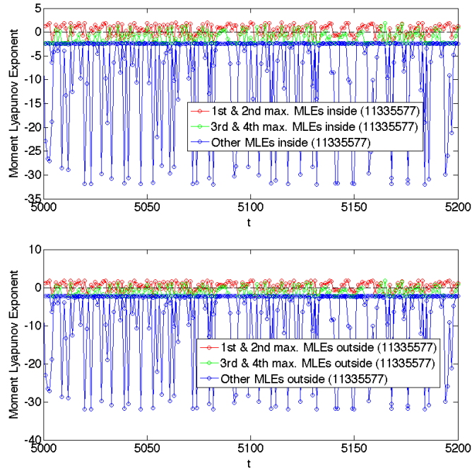
Figure 4.9: Temporal dynamics of moment Lyapunov exponents with initial condition inside of (11335577) . Top: Moment Lyapunov exponents to the direction inside of (11335577). Bottom: Moment Lyapunov exponents to the direction outside of (11335577). Horizontal axis: Time step t . Vertical axis: Moment Lyapunov exponent. k_r = 0.4 , \alpha = 5.0 .
