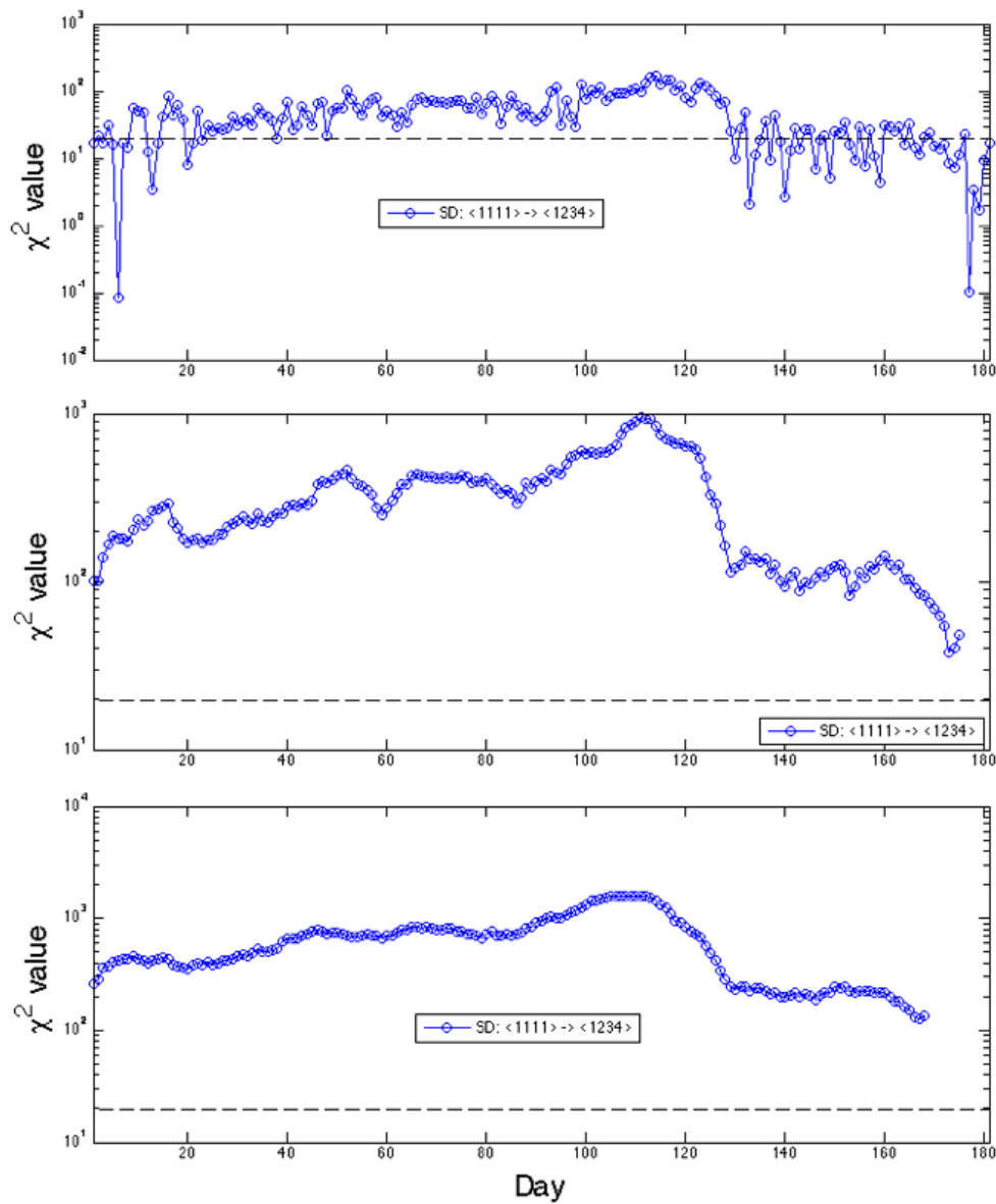
Figure 10.5: Degree of interaction lost by system decomposition \langle 1234 \rangle . Top: p(\mathbf{x}) was taken as daily scale distribution. Middle: Weekly scale. Bottom: Biweekly scale. Vertical axis: The \chi^2 value of the equation (10.53). Horizontal axis: Decimal date in Tab.10.1. The dashed line is the 5 % threshold of \chi^2 test.
