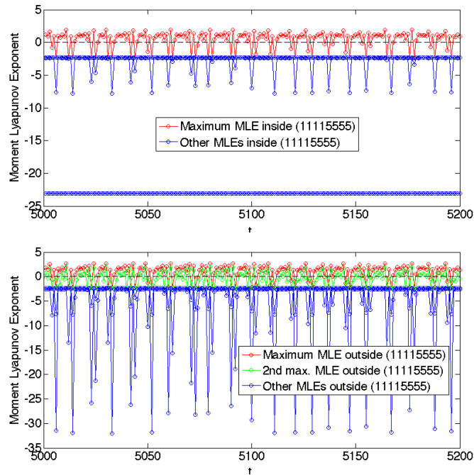
Figure 4.10: Temporal dynamics of moment Lyapunov exponents with initial condition inside of (11115555) . Top: Moment Lyapunov exponents to the direction inside of (11115555). Bottom: Moment Lyapunov exponents to the direction outside of (11115555). Horizontal axis: Time step t . Vertical axis: Moment Lyapunov exponent. k_r = 0.4 , \alpha = 5.0 .
