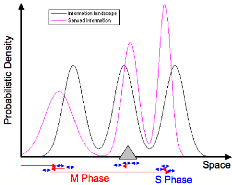
Figure 8.16: Multi-scale evaluation of collective infotaxis with respect to the actual information landscape. Both actual information landscape (black line) and sensed information (magenta line) are approximated as Gaussian mixture distribution. The KL divergence between them allows us to quantify the efficiency of the collective search varying both in temporal and spacial resolution, as well as between the mean and variance components.
