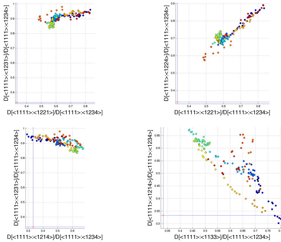
Figure 12.14: Examples of uncorrelated and correlated dynamics of political weblog data on D_{SD} coordinates in biweekly scale. The surface color of the circles represents the time axis during the presidential. The blue lines correspond to the partial extreme values C_c^R(1) , while the red asterisk is C_c^R(2) . Both uncorrelated and correlated dynamics can be approximately explained as a geodesic flow on D_{SD} toward C_c^R(1) and C_c^R(2) , respectively. The last figure shows an example of negative correlation representing the transition of complexity from one subsystem to another, during the 1st and the 2nd round (112th-127th day) of presidential.
