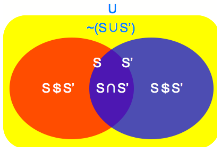
Figure 4.17: Venn diagram of symmetric difference $. The exclusive disjunction or XOR of two cognitive sets S and S' coincides with S\$S' , within the universe of possible cognitive sets U . Based on [48].
