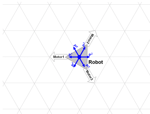
Figure 8.2: Definition of moving directions with respect to the nearest pattern during search phase. The side length of the triangular lattice corresponds to the moving speed v_S .
