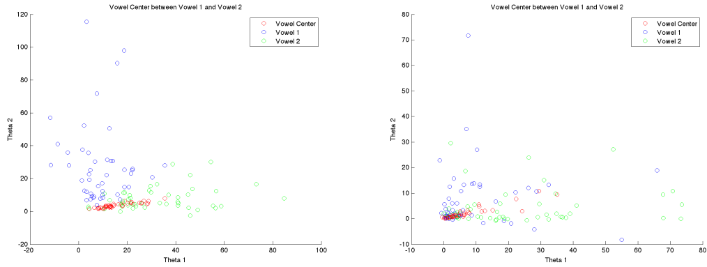
Figure 18.10: Examples of localization of 2nd order circumcenter in \theta coordinates. Left: Plot of /a/(blue), /e/(green) and their 2nd order circumcenter(red) in \theta_1 - \theta_2 plane of individual B. Right: Plot of /a/(blue), /e/(green) and their 2nd order circumcenter(red) in \theta_1 - \theta_2 plane of 26 male and 29 female population.
