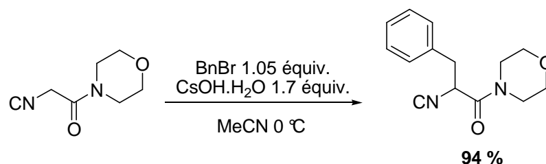
Figure 73 : Alkylation d' \alpha -isocynoamides
