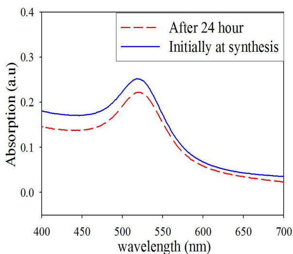
Figure 2.6: Stability of 15 gold NPs with time.
