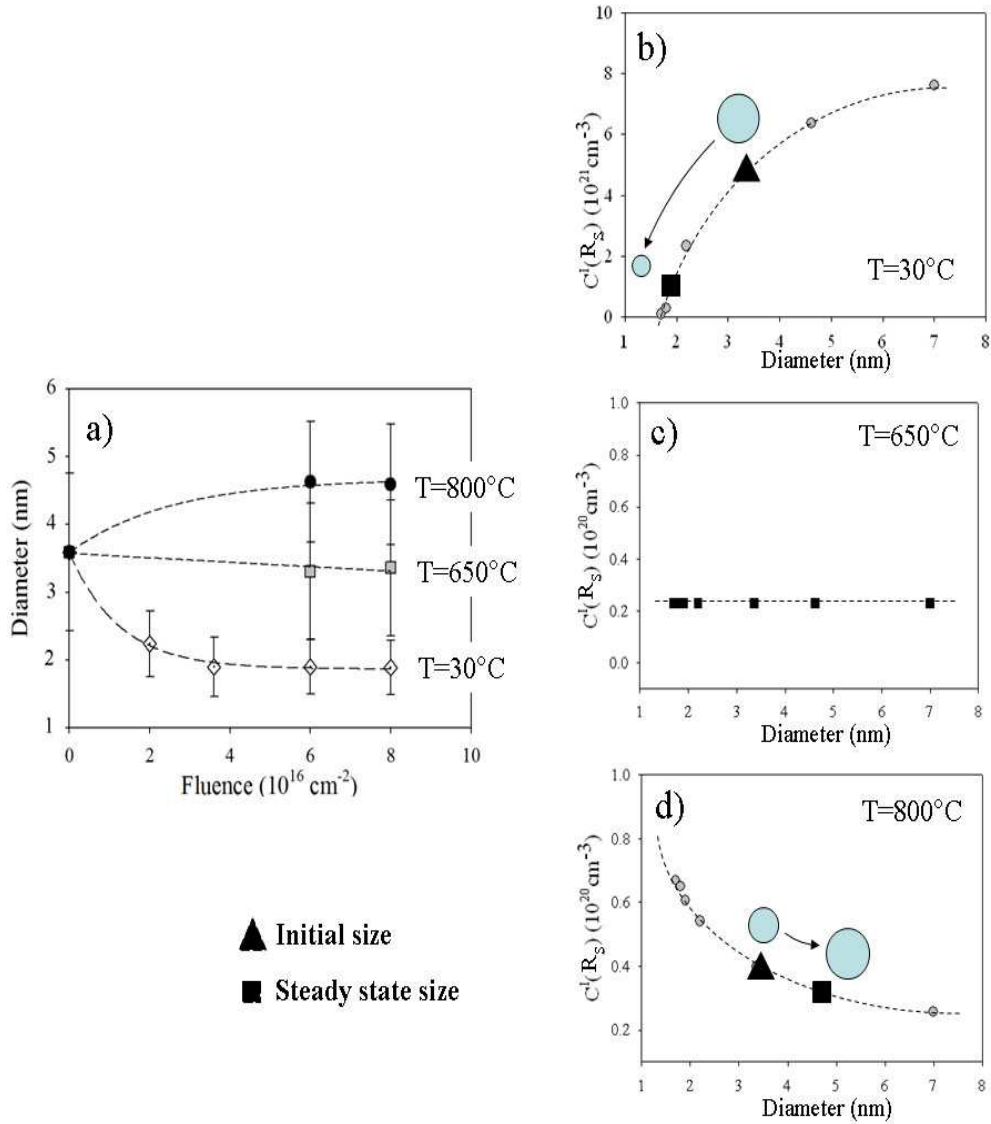
Figure 7.17: a) experimental evolution under irradiation of 3.6nm Au NPs with temperature. b-d) steady-state concentration, C^I(R) with the irradiation temperatures: b) 30°C, c) 650°C, and d) 800°C. Full triangle represents the initial NP size and full square the steady-state size. The evolution of the system is indicated by the arrows.
