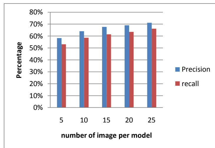
Figure 4-22: precision and recall with respect to the number of images per model (number of images in query is N=10)
