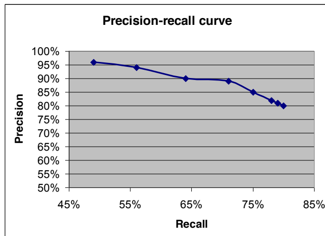
Figure 4-10: Precision-recall curve in our first person re-identification experiment.
