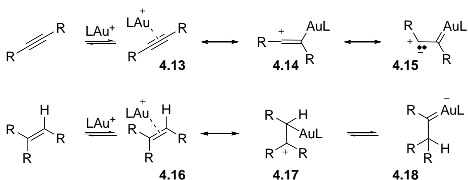
Scheme 4.3: Resonance structures of gold-alkyne and gold-alkene complexes.
