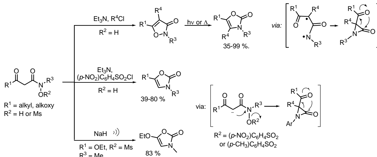
Scheme 3.1: Some examples of oxazolones synthesis starting from ( N -aryl- N -hydroxy)-acetylammides derivatives.
