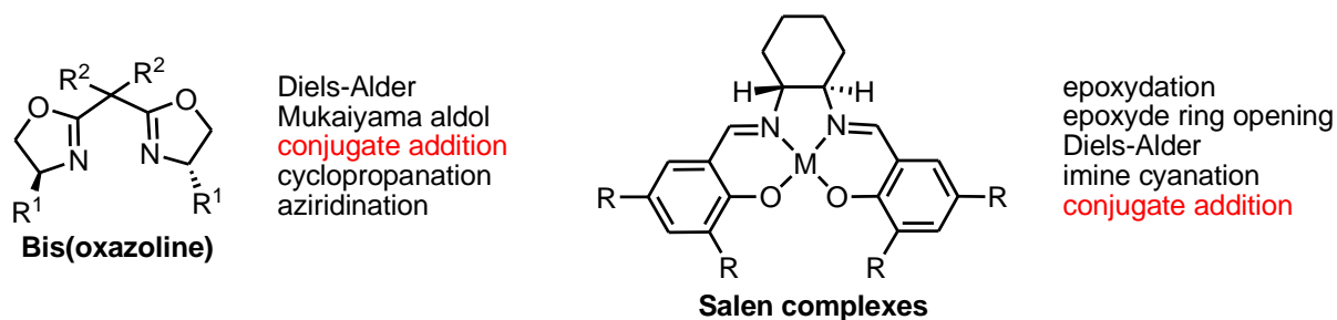
Figure 1.4: Examples of two possible competent ligands in the Michael addition to alkylidene isoxazolones, bis(oxazoline) and Salen complexes.
