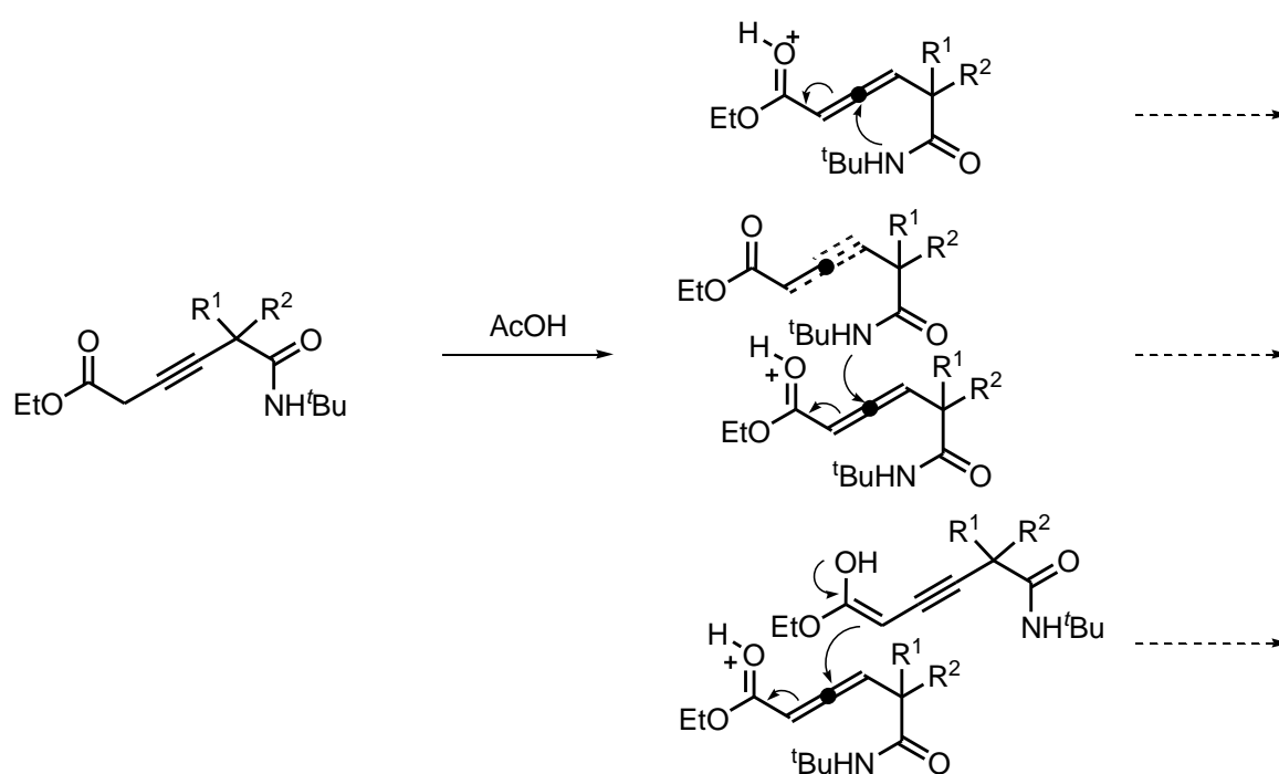
Scheme 1.36: Examples of possible degradation pathways for compounds 1.23h and 1.23i , hypothesized from a common allene precursor, which can ultimately even culminate in oligomerization products.
