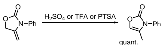
Scheme 3.8: Isomerization of alkyldene carbamates under acidic conditions
