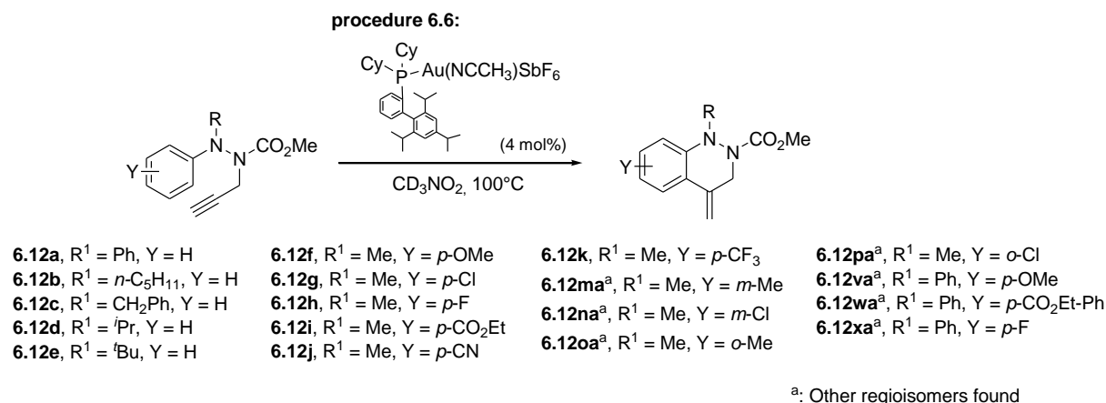
Scheme B.3.5.2: Gold catalyzed transformation towards tetrahydrocinnolines 6.12a-x .
