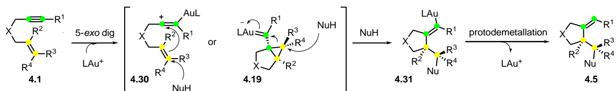
Scheme 4.8: Mechanistic proposal for gold-mediated alkoxy cyclization reactions.
