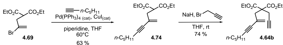
Scheme 4.21: synthesis of substrate 4.64b .
