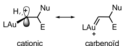
Figure 2.11: Non-ligand p -orbitals are lower in energy than \pi^* orbitals of \pi -ligands and thus, more suitable for back-donation from gold. In complexes where strong back-donation is present, the carbenoid mesomeric form should better describe the nature of this intermediate.
