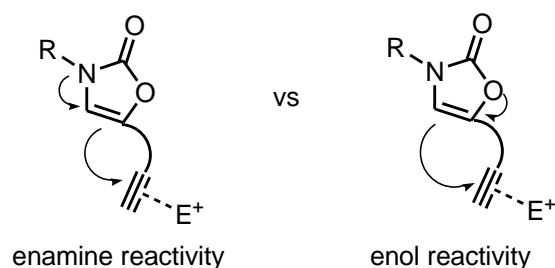
Figure 3.5: The possible reason for the inertness of 4-oxazol-2-ones towards electrophiles can be the low nucleophilicity of the double bond due to the antithetic reactivities accessed by enol against enamine modes of attack (“push-push system”).
