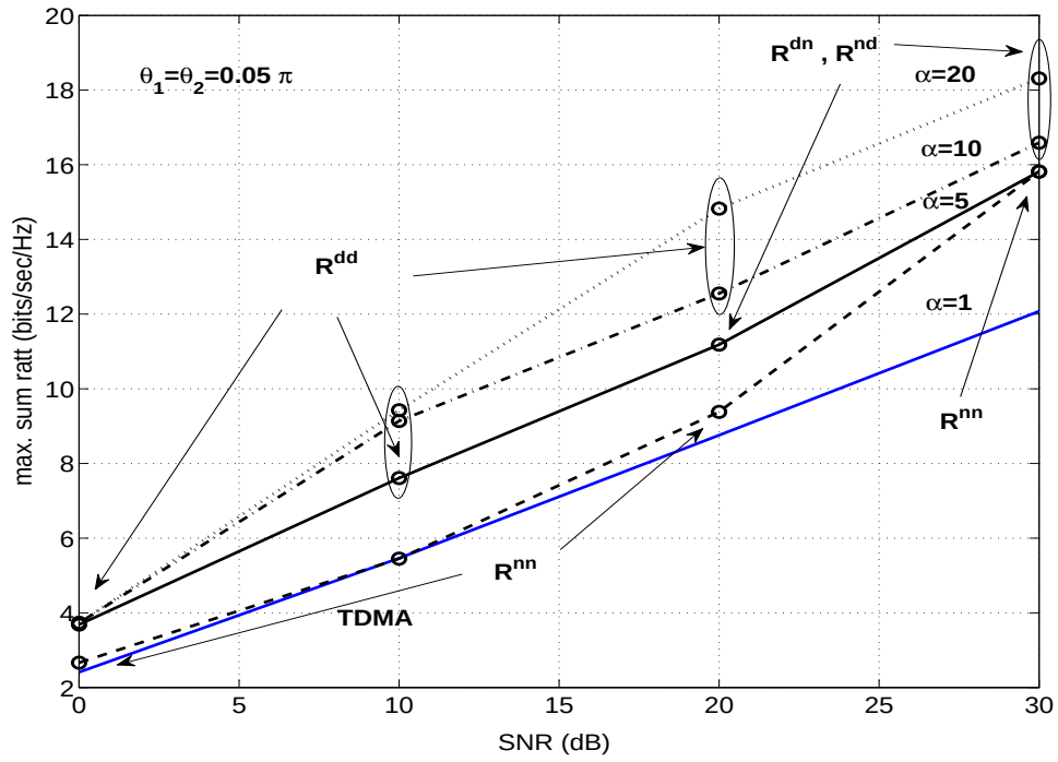
Figure 5.12: The averaged sum rate of different decoding structure comparing to TDMA in symmetric channel when the system SNR increases.
