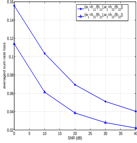
(a) The averaged sum rate difference between maximum sum rate point and MRT strategies in \mathbf{R}^{nd} .
