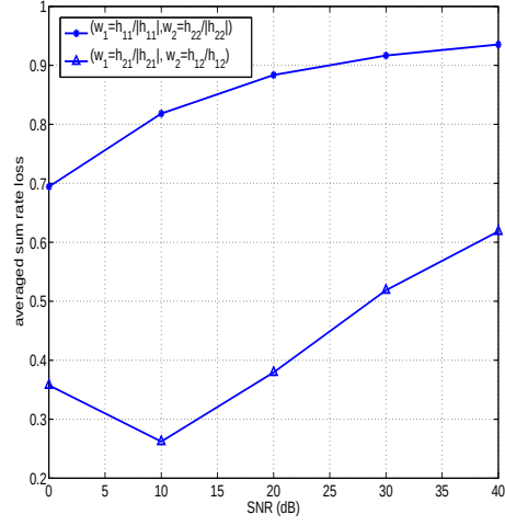
(b) The averaged sum rate difference between maximum sum rate point and MRT strategies in \mathbf{R}^{dd} .
