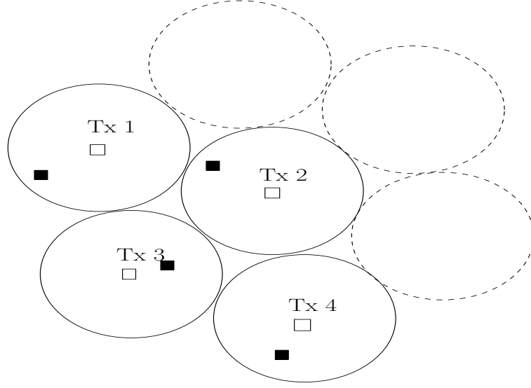
Figure 4.1: This figure illustrates a system of N = 7 cells where N_c = 4 cells form a coordination cluster. Empty squares represent transmitters whereas filled squares represent receivers. The noise power (which includes out-of-cluster interference) undergone in each cell varies from link to link.
