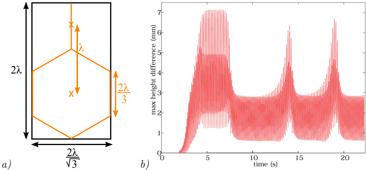
Figure 3.1: a) : Horizontal dimensions of the periodic box that includes one hexagon. Orange : hexagonal pattern. Black : borders of the box. b) : Evolution of \Delta\zeta(t) in the nonlinear saturated regime. Resolution: 180 points in z , 50 points per wavelength in x and y . The hexagonal state is reached when the height amplitude is maximum.
