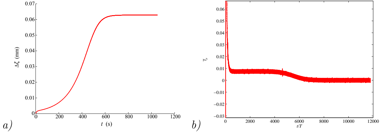
Figure 4.3: a) Growth of a small perturbation of the flat interface. Envelope of \Delta\zeta as a function of time for a = 0.0543g > a_c = 0.054186g . b) Growth rate of \Delta\zeta , i.e. the time derivative of a).
