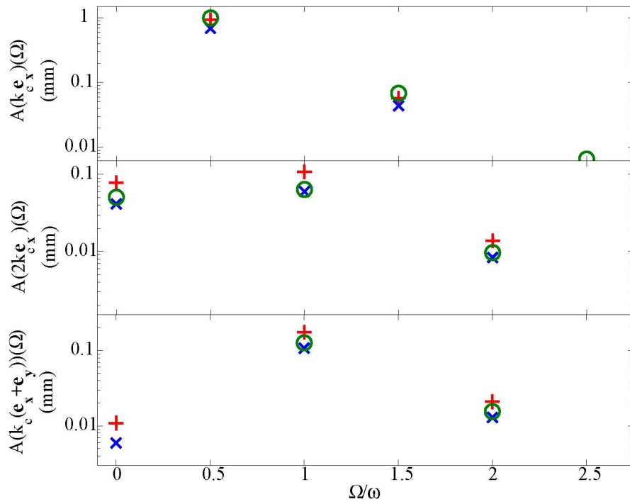
Figure 2.11: Temporal Fourier transform of the amplitudes in figure 2.10. Circles indicate experimental results of Kityk et al. (2009), while crosses and plus signs indicate numerical data with \langle \zeta \rangle = 1.6 mm and \langle \zeta \rangle = 1.7 mm respectively.
