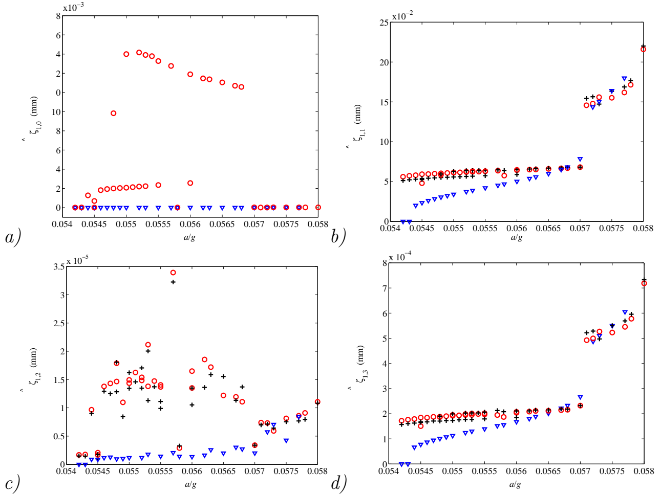
Figure 4.15: Spatiotemporal modes k=k_c as a function of the acceleration. a) \omega = 0 ; b) \omega = \pm\omega_0/2 ; c) \omega = \pm\omega_0 ; d) \omega = \pm 3\omega_0/2 . Red circles: leftward propagating waves ( n > 0 ). Black crosses: rightward propagating waves ( n < 0 ). Blue triangles: leftward and rightward propagating waves of the forced solution with reflection symmetry to make the comparison easier. The waves of zero temporal frequency do not move.
