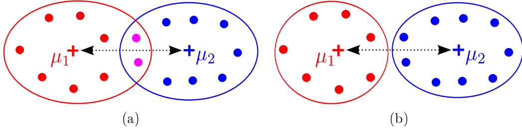
Figure 4.8: Separation between two clusters. Unlike conventional separation indices that base their separation measure on \|\boldsymbol{\mu}_1 - \boldsymbol{\mu}_2\| , which gives the same value for both (a) and (b), OSI criterion computes the separation as the sum of [2 \gamma_i^2 / (\gamma_i^1 + \gamma_i^2)] for all data points \mathbf{x}_i being classified to cluster #1 (red) and [2 \gamma_i^1 / (\gamma_i^1 + \gamma_i^2)] for all data points \mathbf{x}_i being classified to cluster #2 (blue). Using probabilities \gamma_i^k of data points \mathbf{x}_i to belong to cluster # k ensures to take the overall geometric structure between clusters into account [Kim et al. 2004].
