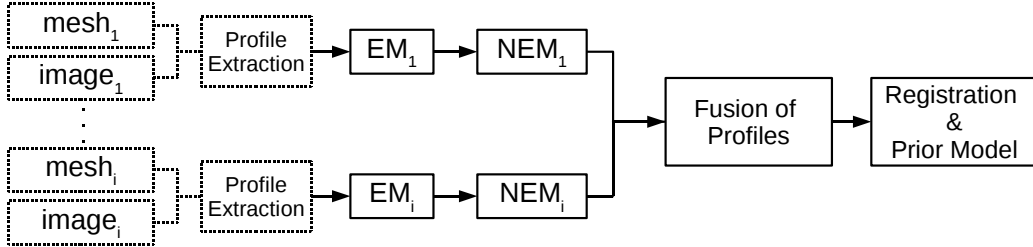
Figure 4.2: Pipeline for Multimodal Prior Appearance Model (MPAM) construction, which includes the Expectation-Maximization (EM) and Neighborhood EM (NEM) algorithms.
