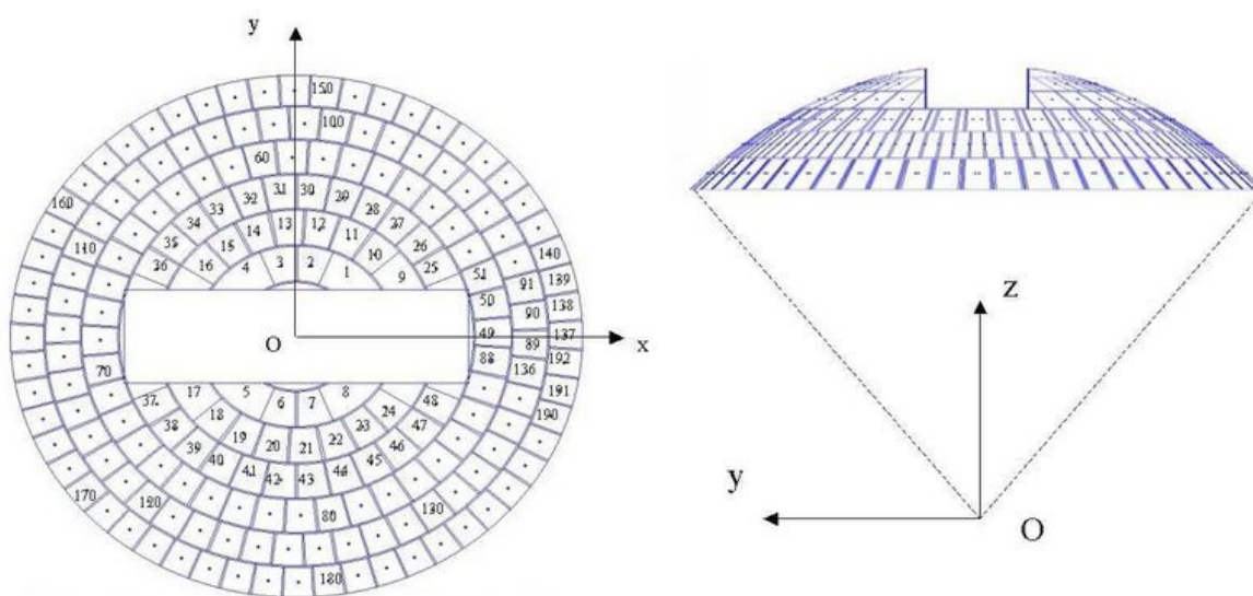
FIGURE 4.2 – Plans du dispositif
