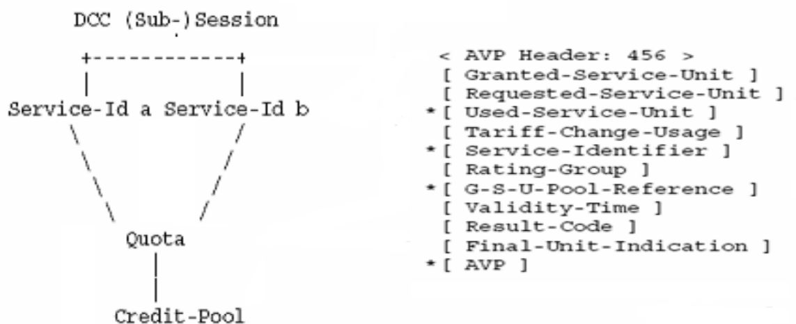
Figure 50: Multi-service-credit-control AVP
