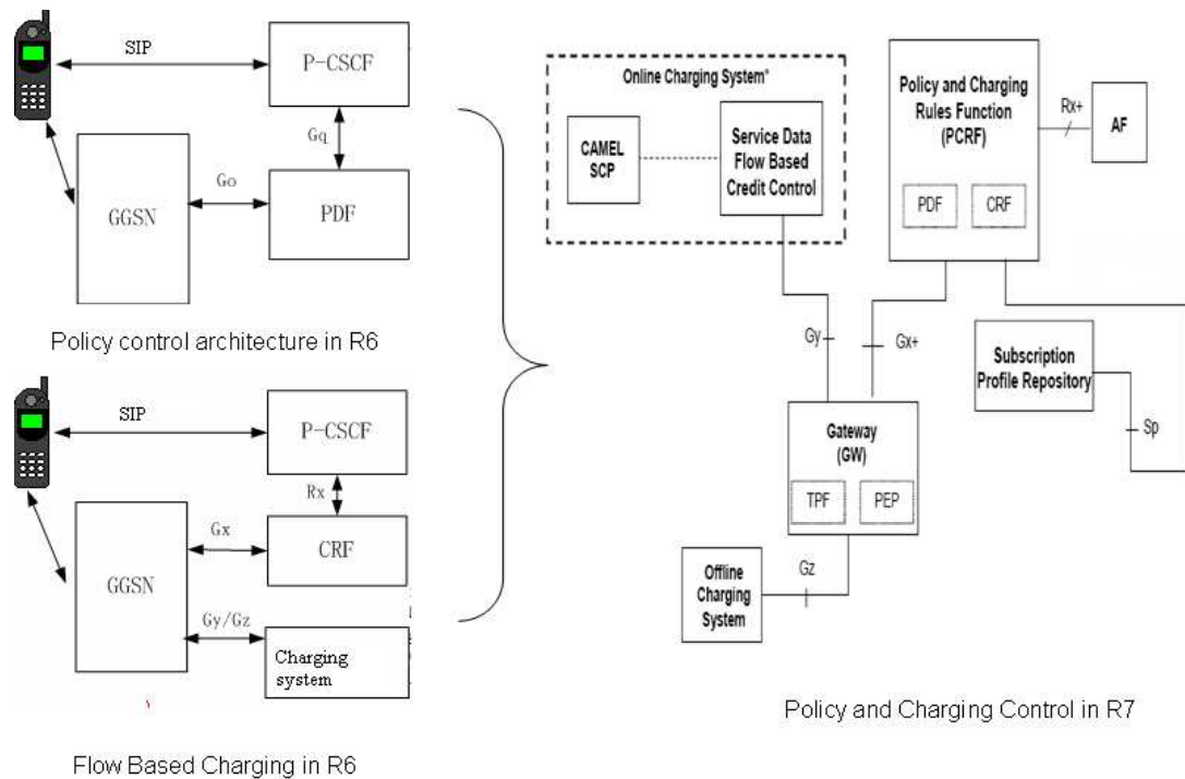
Figure 15 : Evolution vers Policy Charging control
