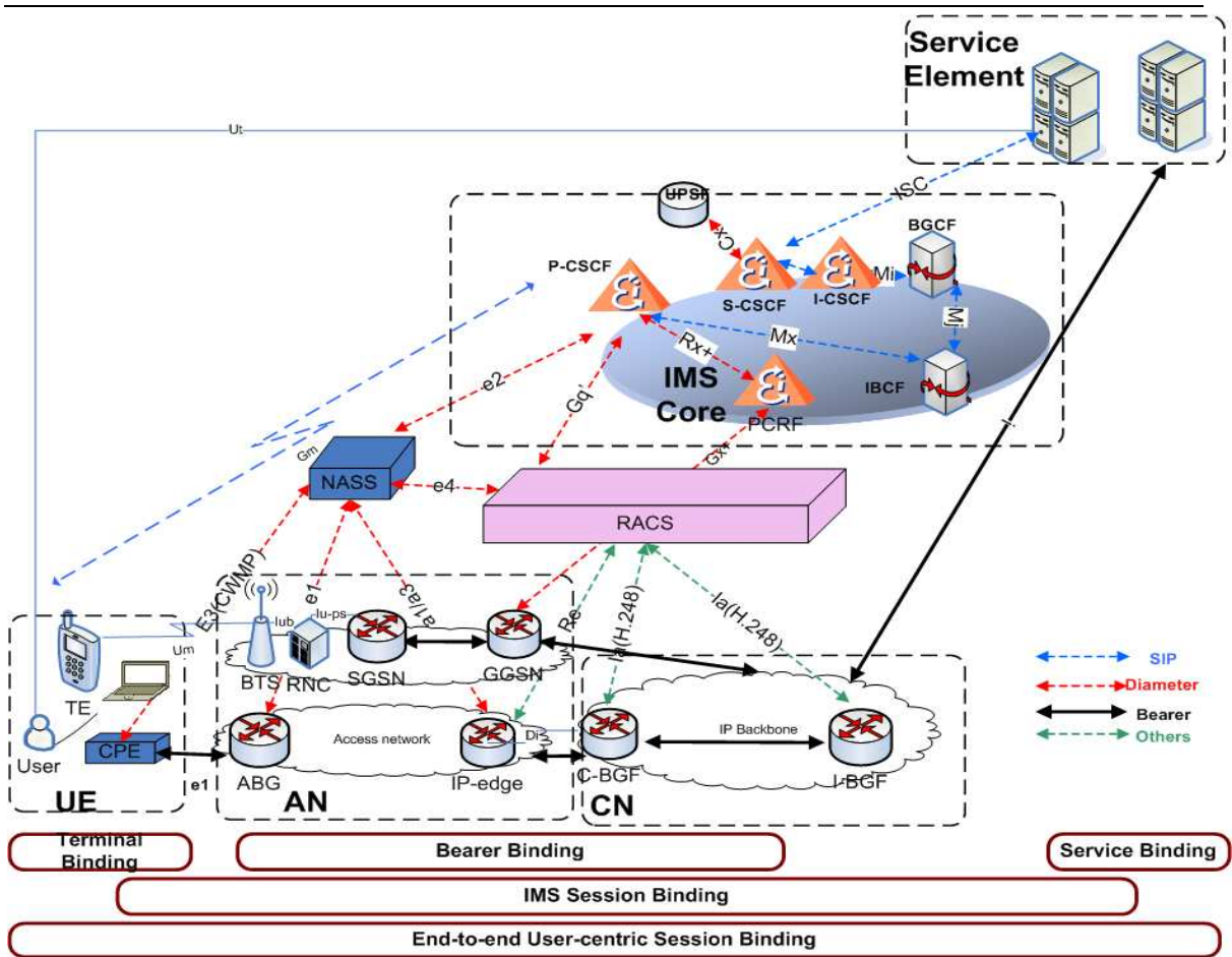
Figure 45 : Binding de la session user-centric
