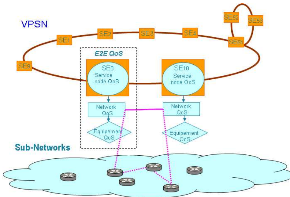
Figure 40 : QoS description of service component
