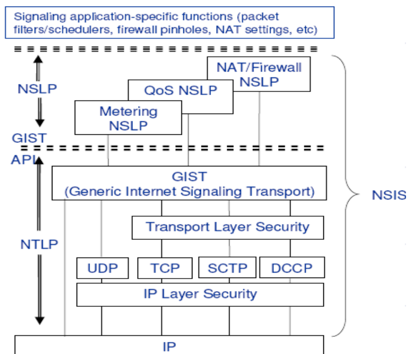
Figure 24 : Architecture NSIS
