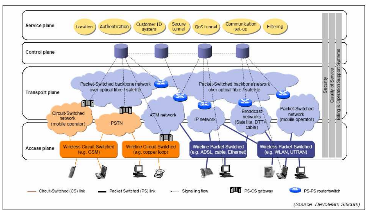
Figure 1 : Next Generation Network
