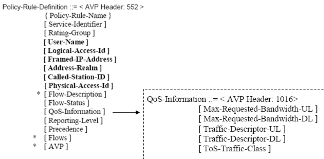
Figure 51: Policy-Rule-Definitaion AVP and QoS information AVP
