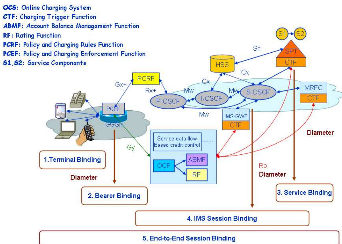
Figure 47 : Architecture globale de Charging user-centric
