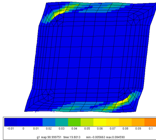
(a) Microstructure size 5.5 \cdot 10^{-7} mm
