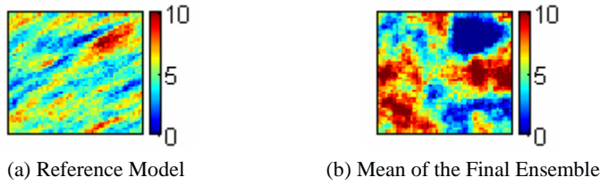
Figure 3-18 In k model (a) Reference Model, (b) Final updated mean model with a new initial ensemble.
