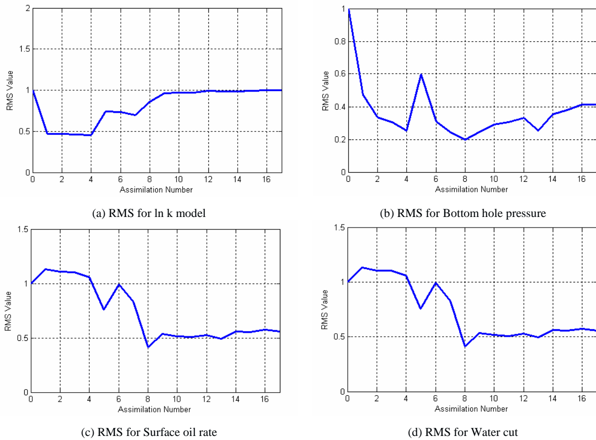
Figure 3-19 RMS against the number of assimilation for (a) In k Mean Model, (b) Bottom hole pressure, (c) Surface oil rate, (d) Water Cut. The initial ensemble consists of In k models with an isotropic spherical variogram.
