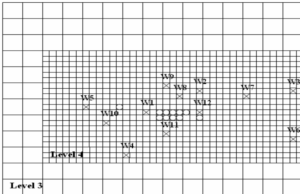
Figure A-2 Well placement in the reservoir (Level 4). Observation wells are displayed by cross and injection/production wells by white circles (from Le Ravalec-Dupin et al. (2004))
