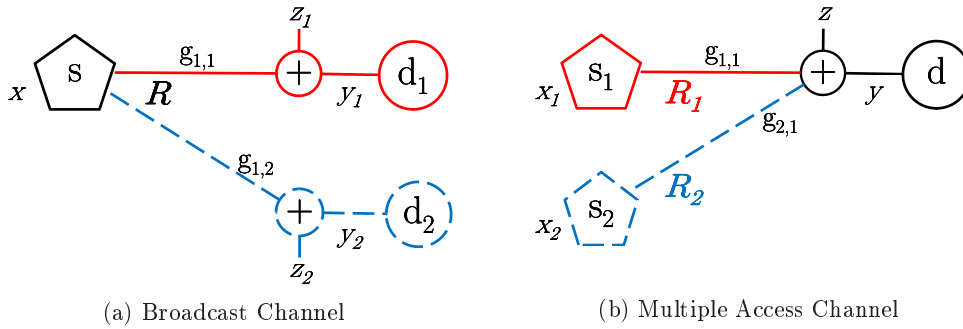
FIGURE 2.1 – Two-user Broadcast Channel versus two-user Multiple Access Channel.
