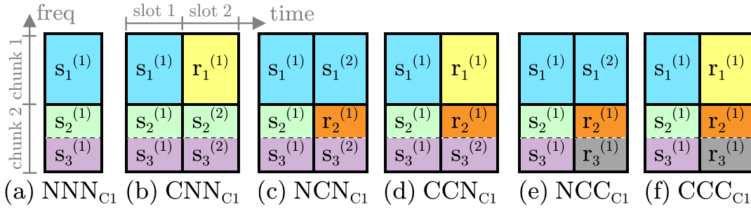
FIGURE 3.4 – Most representative resource allocation patterns for Classic 1 family.
