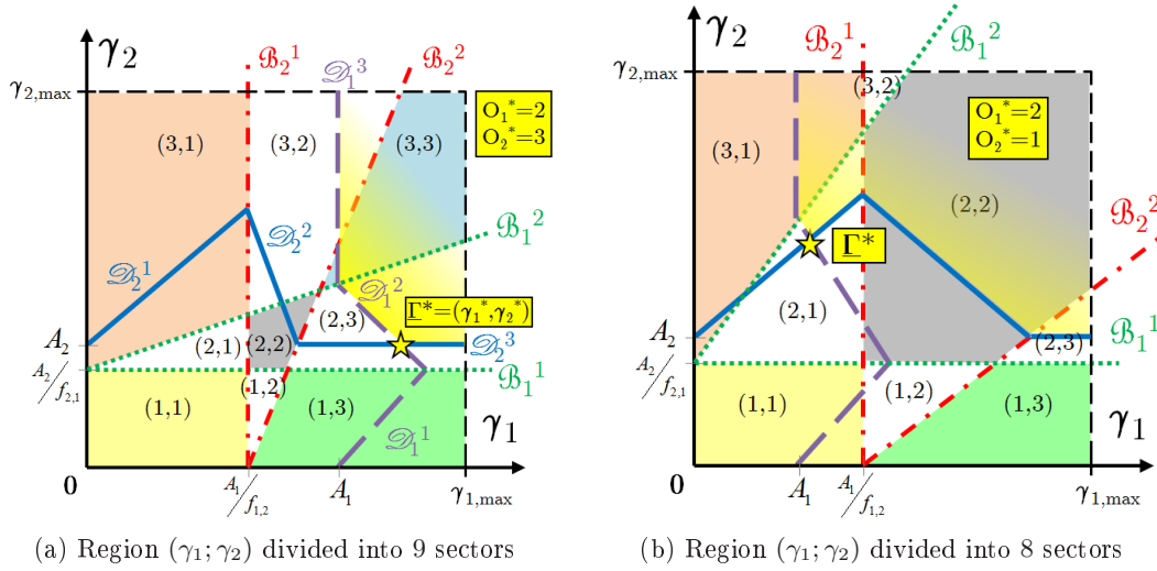
FIGURE 5.4 – Superposition of both achievable SNR regions \mathcal{R}_1^* and \mathcal{R}_2^* . A partition \Omega of the region into nine (left) and eight (right) sectors is achieved.
