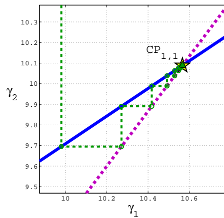
FIGURE 6.4 – Illustration of the ‘ping-pong’ process for power allocation.
