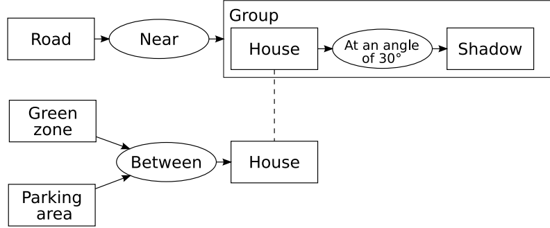
Figure 5.3: Example of nested graph with coreference links, represented as dotted lines.
