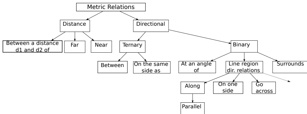
Figure 1.15: Metric relations.
