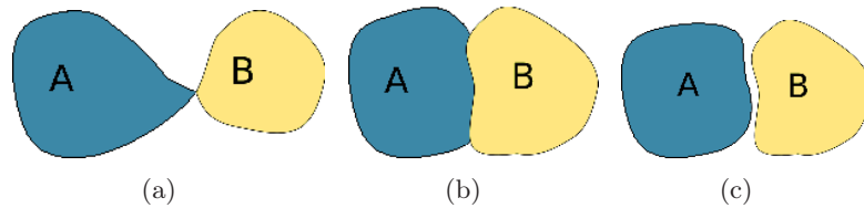
Figure 1.4: Illustrations where the relations of adjacency should be considered as a matter of degree.
