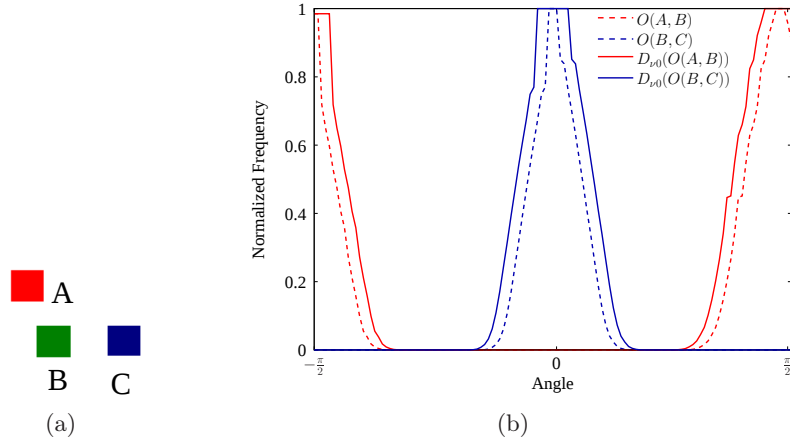
Figure 2.13: (a) Objects. (b) Orientation histograms of the objects (a) and dilated orientation histograms.
