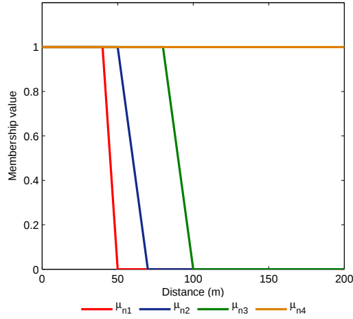
Figure 2.8: Membership functions for \mu_n .
