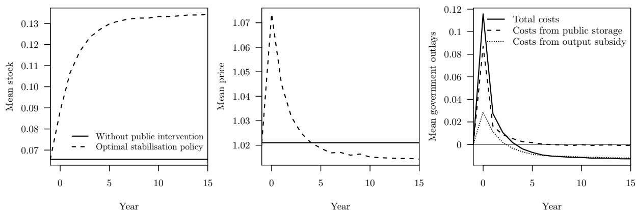
Figure 4.3. Transitional dynamics. Before period 0, the system is on the asymptotic distribution of the model without public intervention. The unexpected policy is announced and starts in period 0. (Obtained by Monte Carlo simulation as the average over 100,000 simulated paths.)
