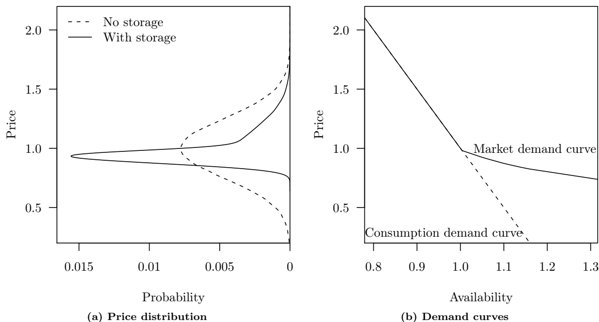
Figure 2.4. Characterisation of the competitive storage model behaviour. Parameters: a = 1.2 , b = 0.2 , c = 0.8 , d = 0.2 , \delta = 1\% , r = 3\% , \phi'(X) = 0.02 , \epsilon \sim N(0, 0.05^2) . These parameters imply mean production and price at 1 when there is no shock, and supply and demand elasticities of 0.2 and -0.2 . In the demand curves (b), the dashed line is consumption demand, the solid line includes consumption demand and demand for carryover.
