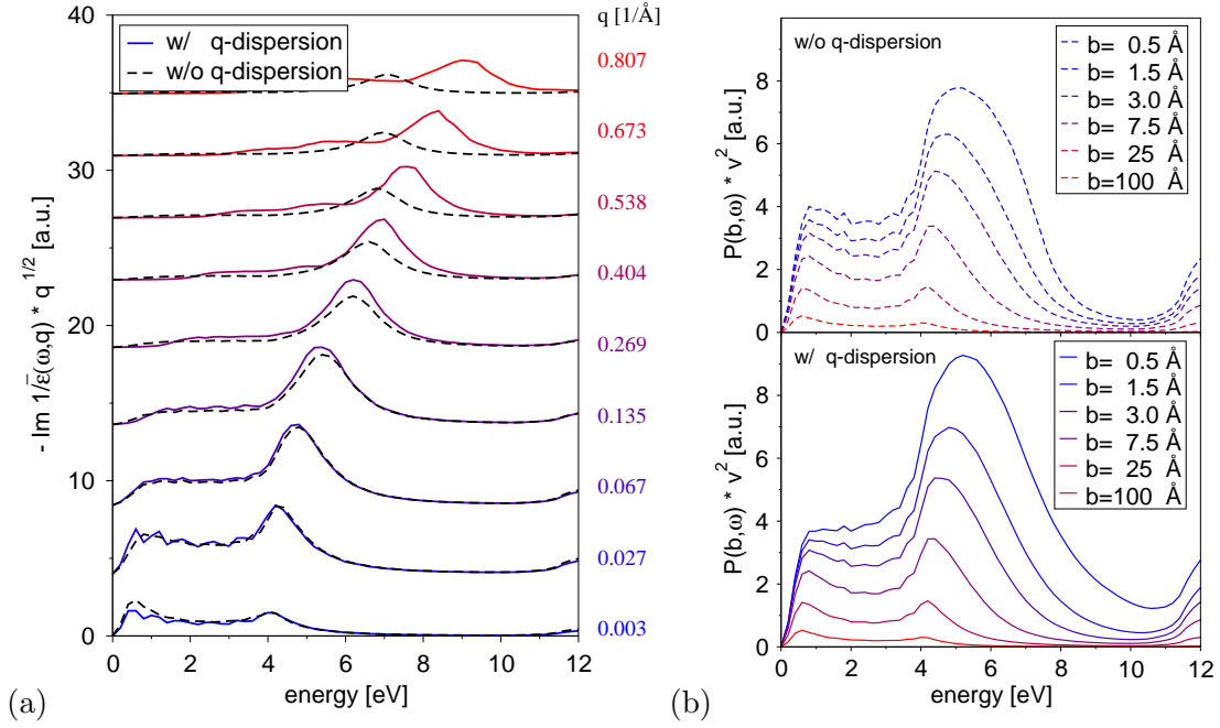
Fig. 7.2: Electron energy-loss spectra for a graphene sheet with and without nonlocal effects. (a) Angular-resolved EELS -\text{Im } \bar{\epsilon}^{-1}(\bar{\mathbf{q}}) \propto \pi L_z v(\bar{\mathbf{q}}) S(\bar{\mathbf{q}}) for different in-plane momentum transfers \bar{q} . The spectra have been shifted along the ordinate. (b) Spatially-resolved EELS for several impact parameters b [see eq. (7.6)]. In (a) and (b), the dynamic structure factor S(\bar{\mathbf{q}}) of graphene is calculated in a local approximation [eq. (7.8), dashed] or by full ab-initio calculations (solid).
