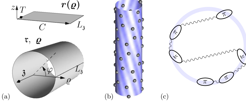
Fig. 6.5: Zone-folding for the microscopic polarisability. (a) Geometry of the cylinder and the unrolled graphene sheet. (b) Surface mode in a (4, 1) nanotube for a helical momentum \xi = (l, p) with angular projection l=10 and on-axis part p=10 \text{ \AA}^{-1} . (c) Non-locality of the susceptibility.
