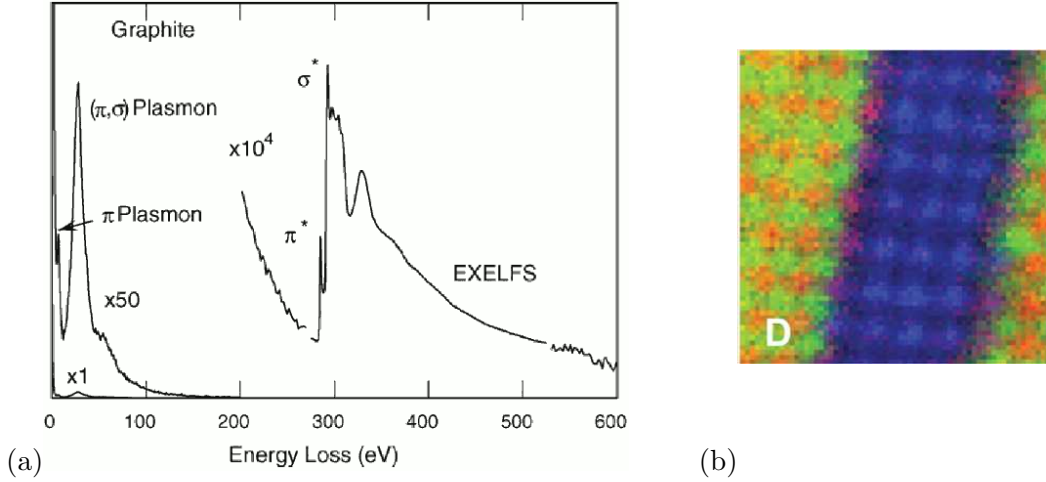
Fig. 1.3: STEM measurements. (a) Electron energy-loss spectrum for graphite in the valence- and core-loss region (Reprinted from [24], Micron © 2008, with permission from Elsevier). (b) An atomic-resolution elemental map of a multilayer system. Colours indicate different edge signals attributed to La (green), Ti (blue), and Mn (red) atoms (Reprinted by permission from Macmillan Publishers Ltd: Nature Materials [15], © 2009).
