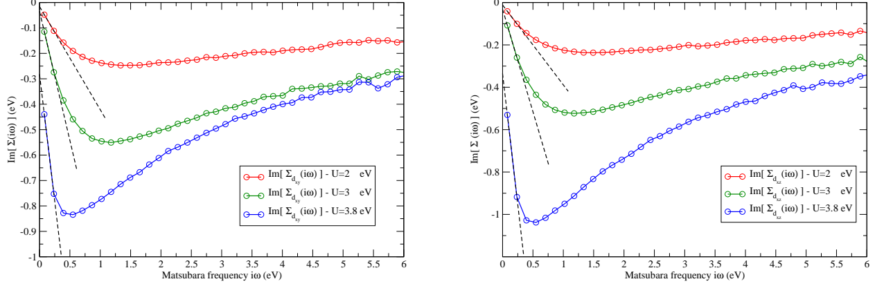
Figure 5.30: Imaginary parts of the LDA+DMFT self-energy on the Matsubara axis associated to the d_{xy} (left panel) and the d_{xz} (right panel) Wannier orbitals for U=2, 3, and 3.8 eV. Parameters as in fig. 5.28. The dashed lines are the linear extrapolations of the self-energy to i\omega = 0 , their slope \alpha is related to the quasi-particle weight Z by the relation Z = (1 - \alpha)^{-1} .
