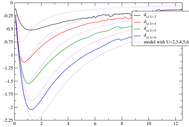
Figure B.1: Imaginary part of \Sigma_{d_{xz}}(i\omega) for undistorted \text{Sr}_2\text{IrO}_4 without spin-orbit coupling T=300 K ( \beta = 40 \text{ eV}^{-1} ) and with J=0.2 eV. The purple curves are the modeled behavior of the imaginary part of the self-energy for a 3/4 filled band in the atomic limit. For U \geq 4 eV \Sigma_{d_{xz}}(i\omega) behaves quite similarly as that of the model.
