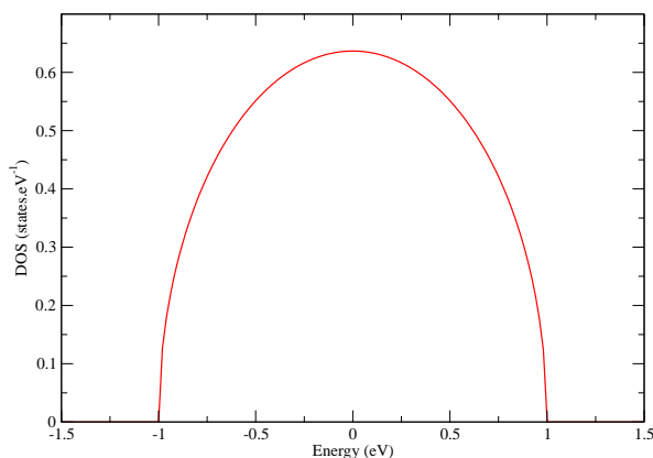
Figure 1.2: Density of states of the Bethe lattice in infinite dimensions, with a half bandwidth D = 1.0 eV.
